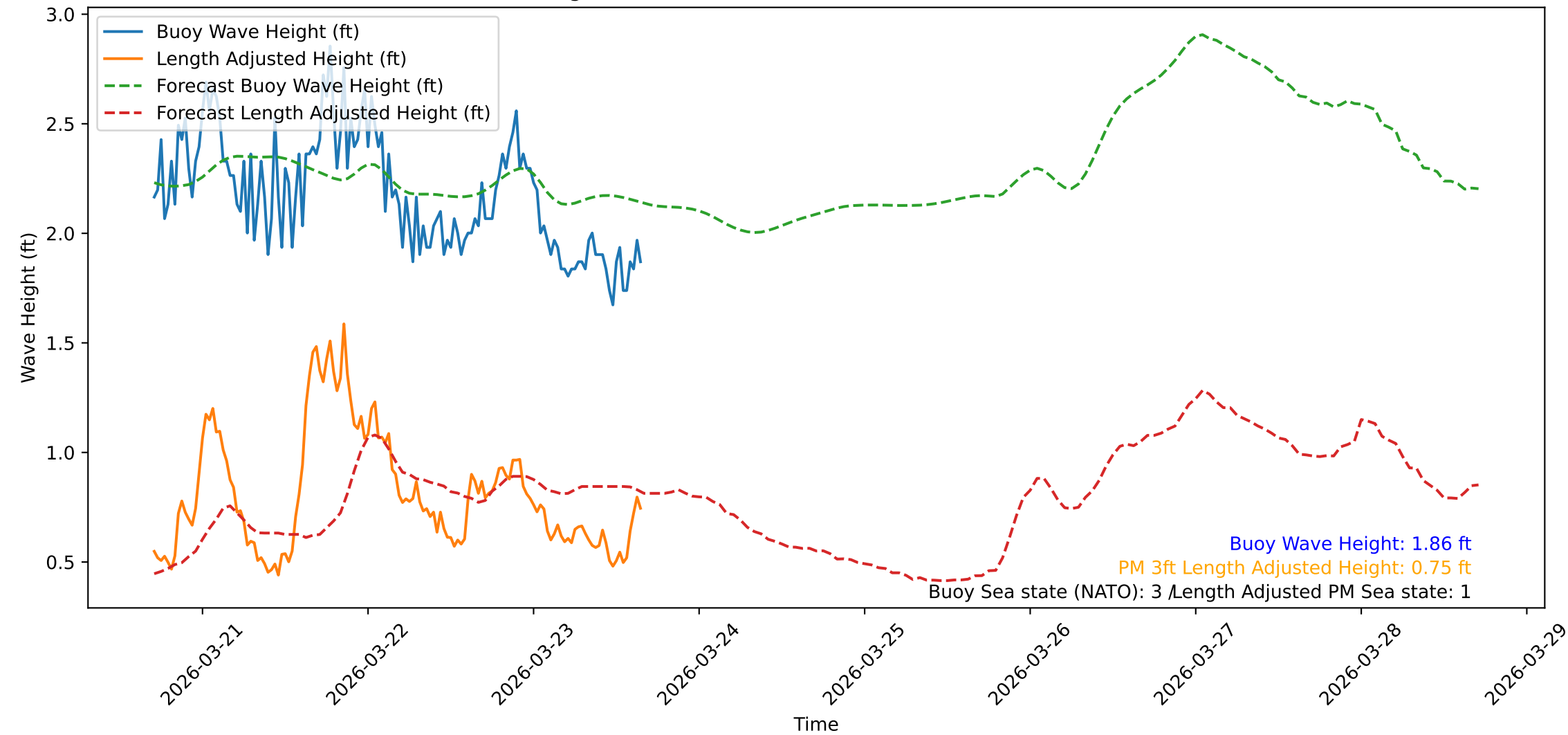
Wave Heights over Time for Red Beach at 2026-03-23 16:40:47
