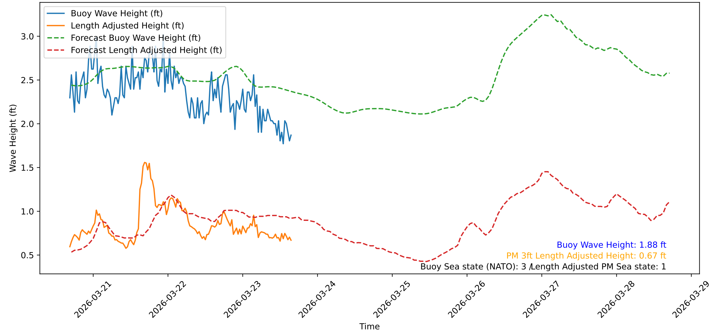
Wave Heights over Time for Oceanside Harbor at 2026-03-23 16:40:31
