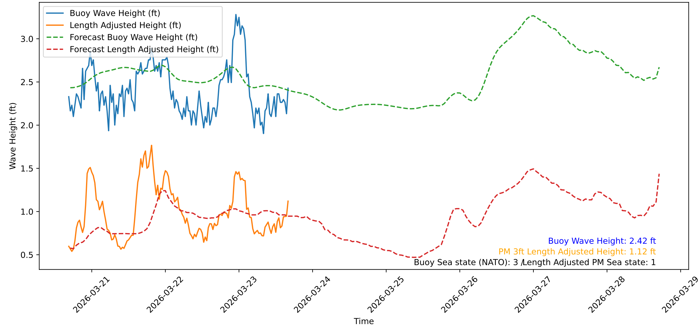
Wave Heights over Time for Green Beach at 2026-03-23 16:41:09
