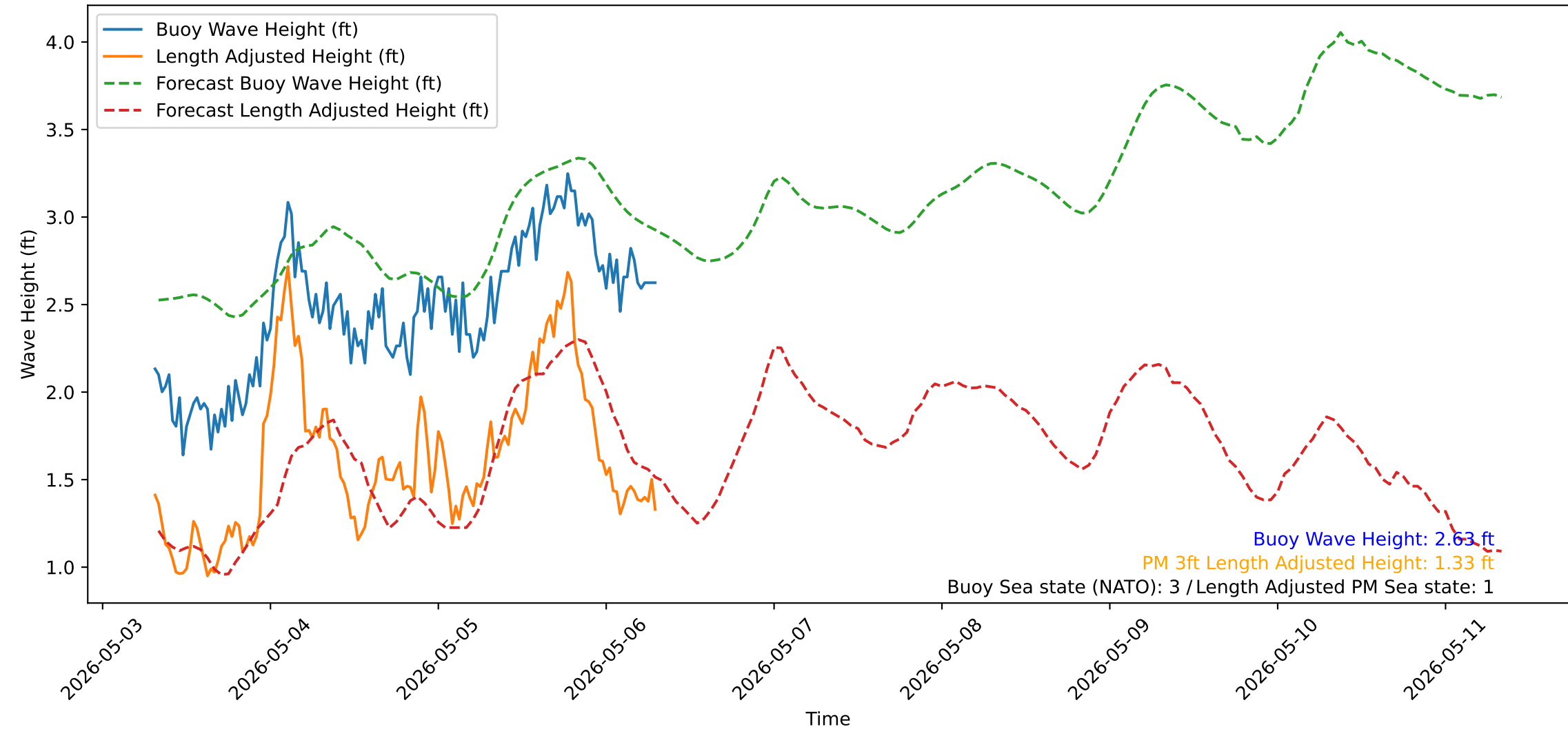
Wave Heights over Time for Oceanside Harbor at 2026-05-06 07:30:31
