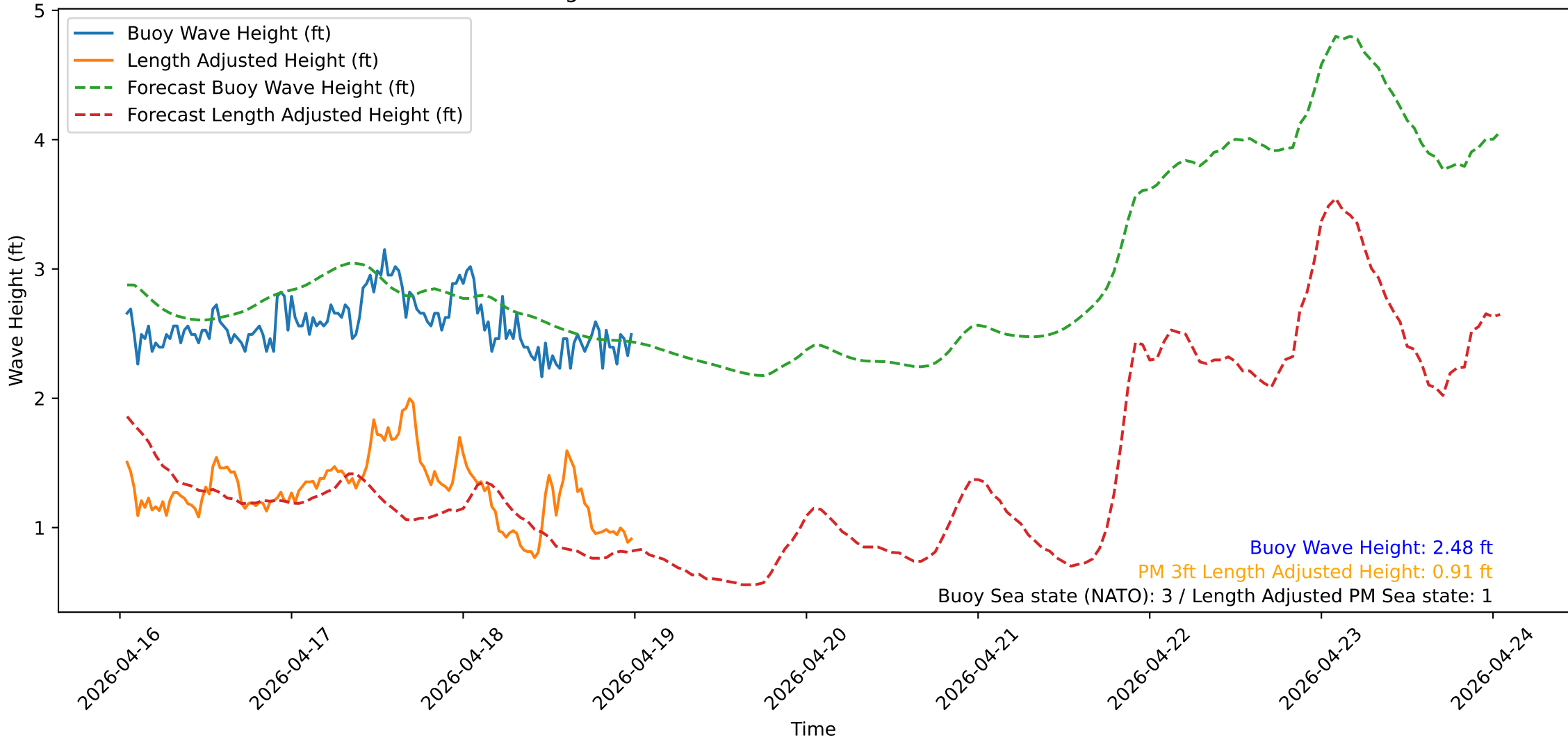
Wave Heights over Time for Red Beach at 2026-04-19 00:30:51
