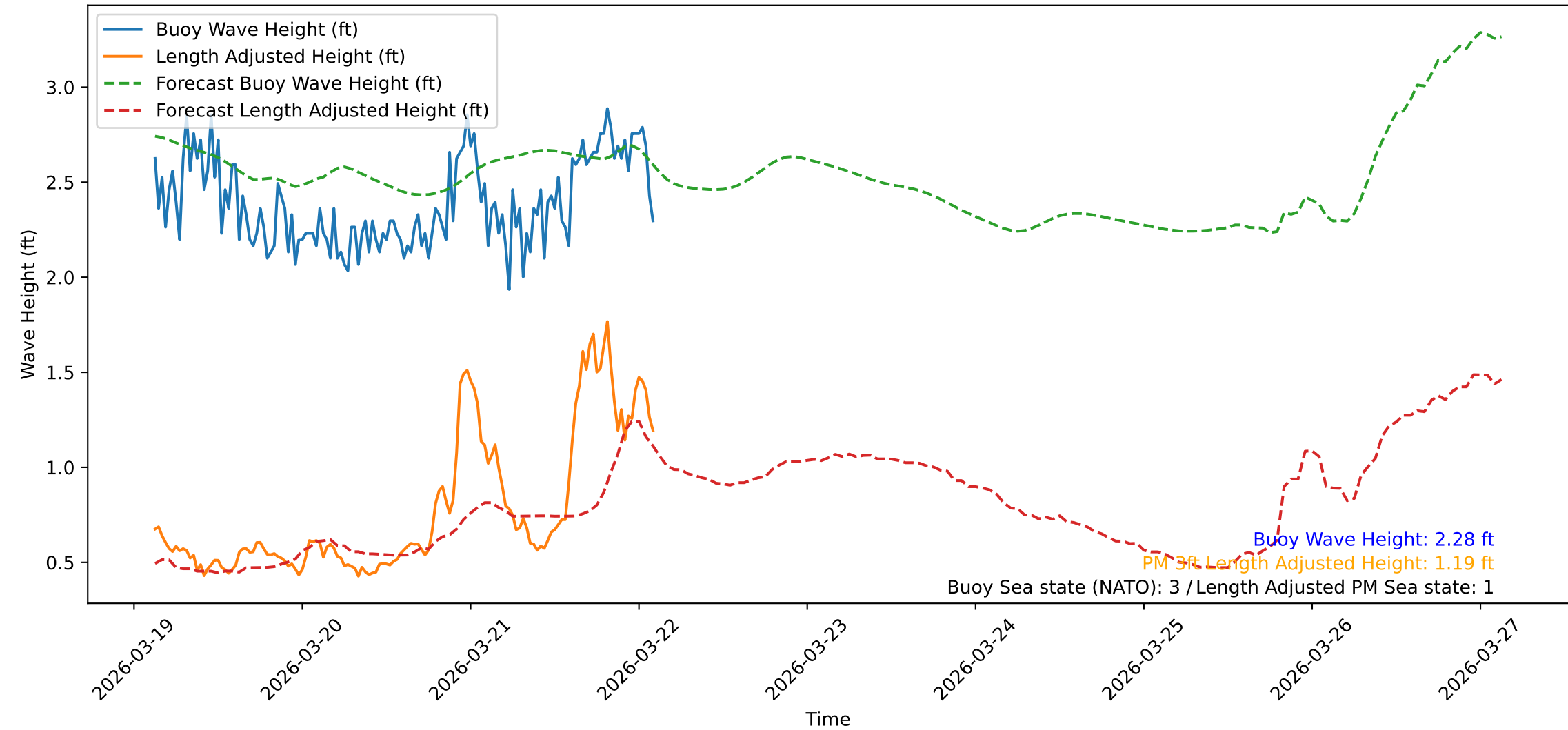
Wave Heights over Time for Green Beach at 2026-03-22 03:01:09
