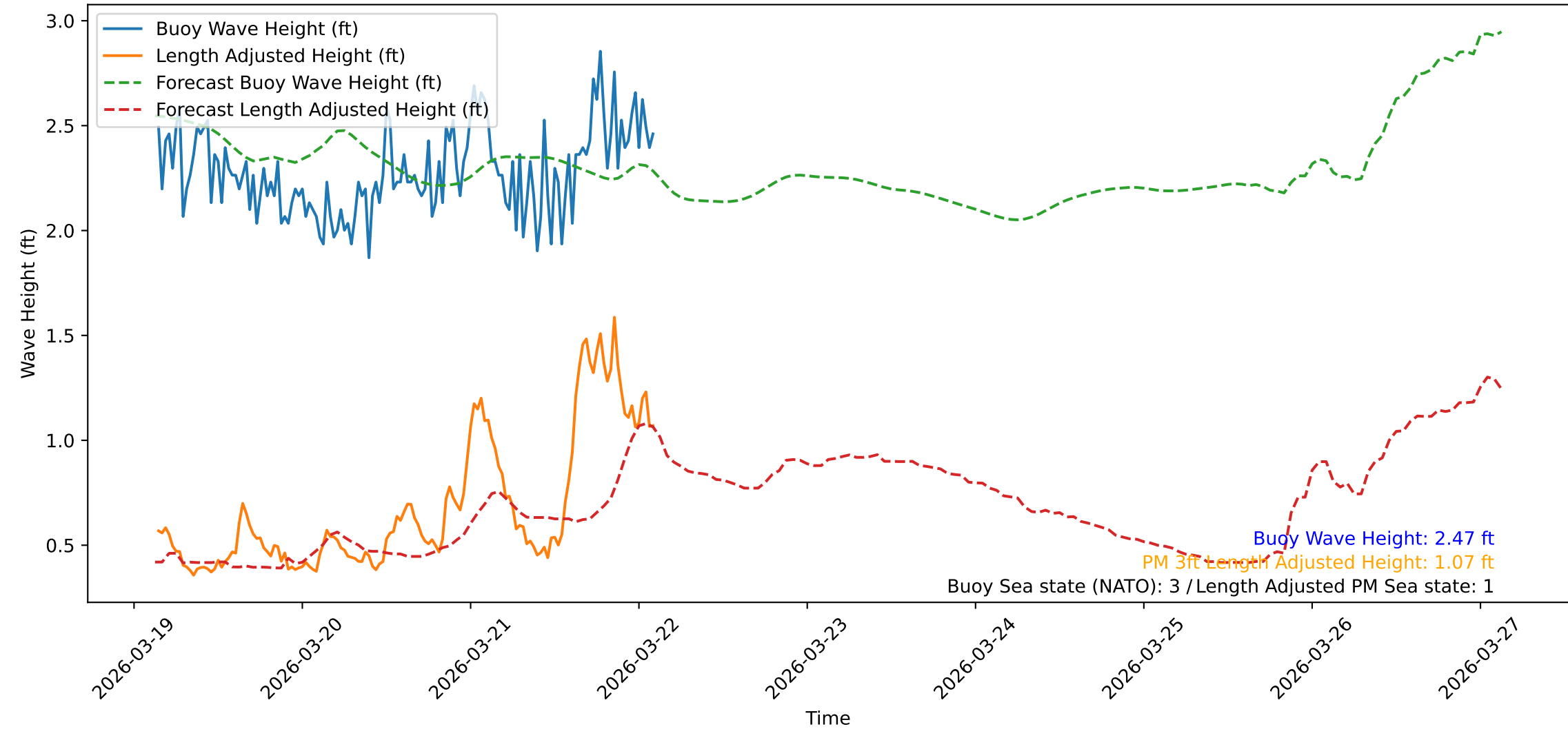
Wave Heights over Time for Red Beach at 2026-03-22 03:00:47
