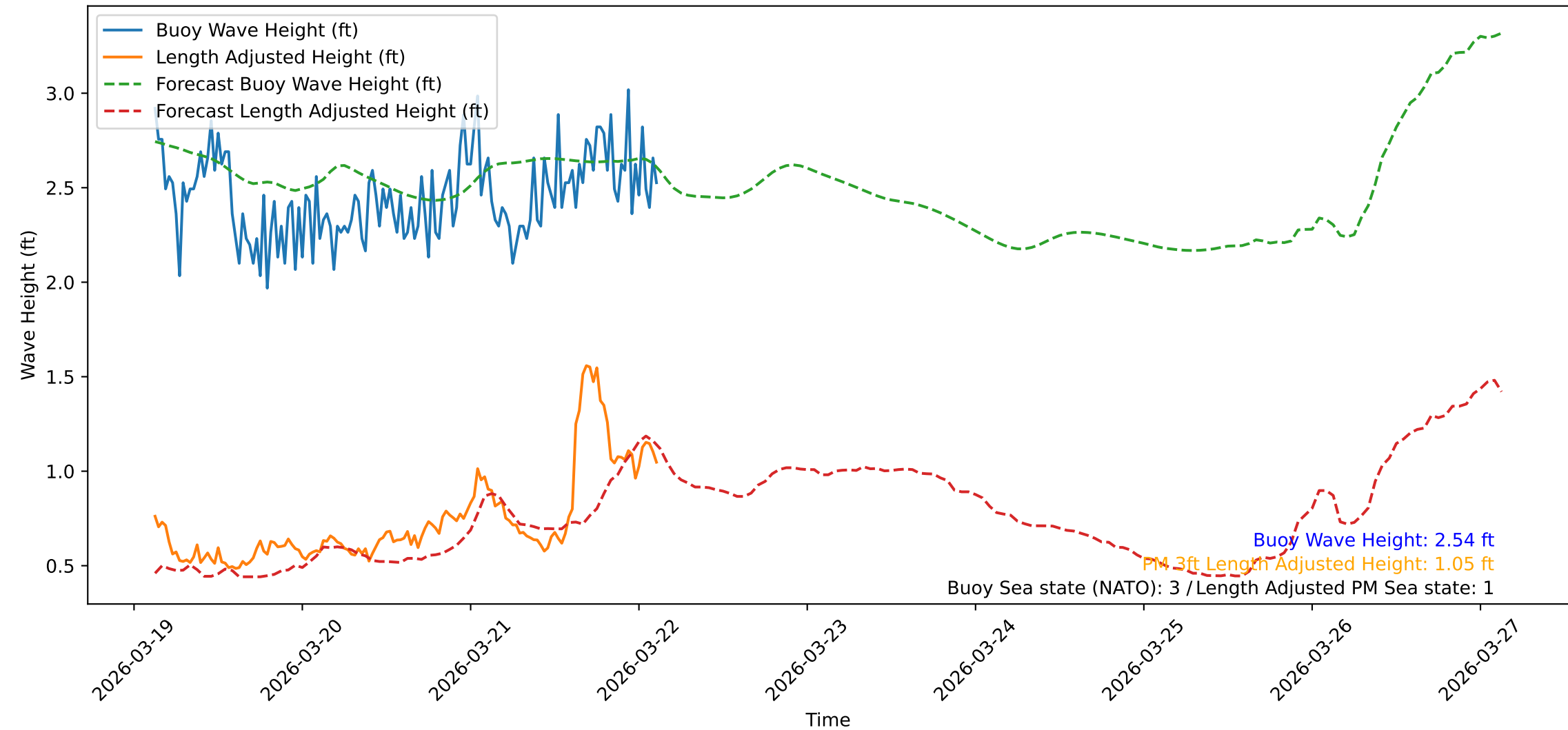
Wave Heights over Time for Oceanside Harbor at 2026-03-22 03:00:31
