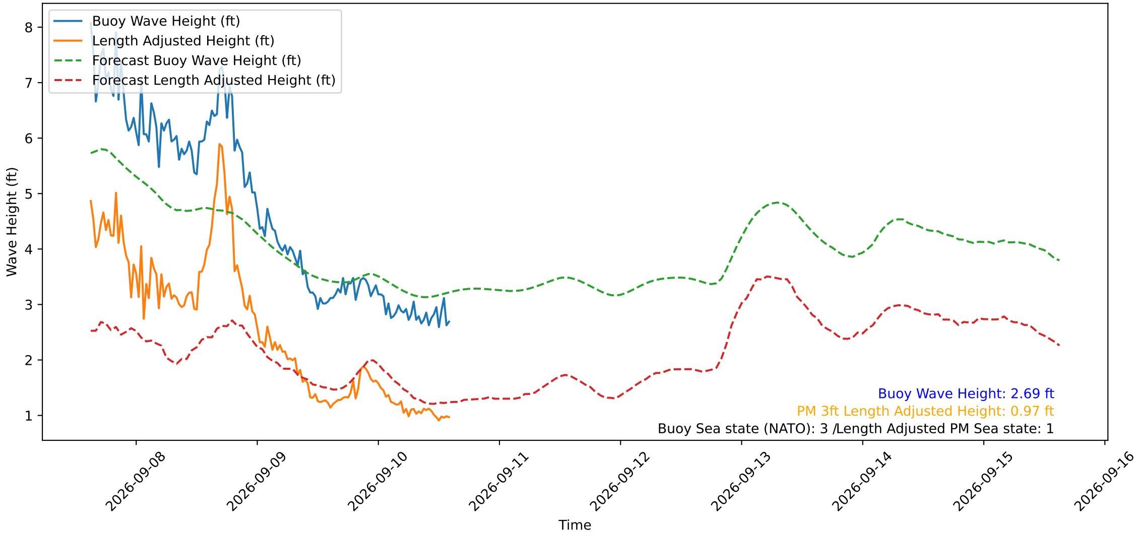
Wave Heights over Time for Green Beach at 2026-09-10 14:41:12
