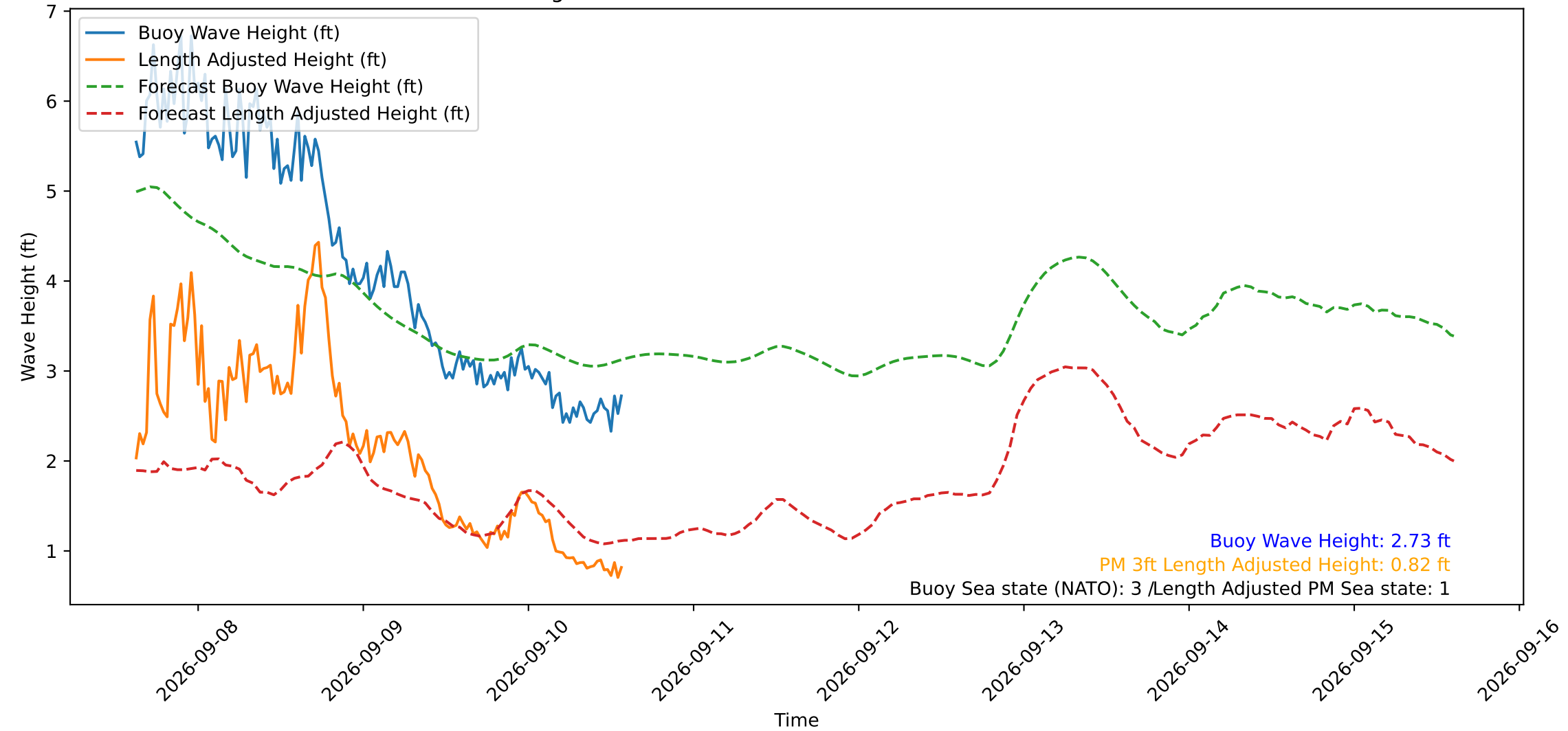
Wave Heights over Time for Red Beach at 2026-09-10 14:40:50
