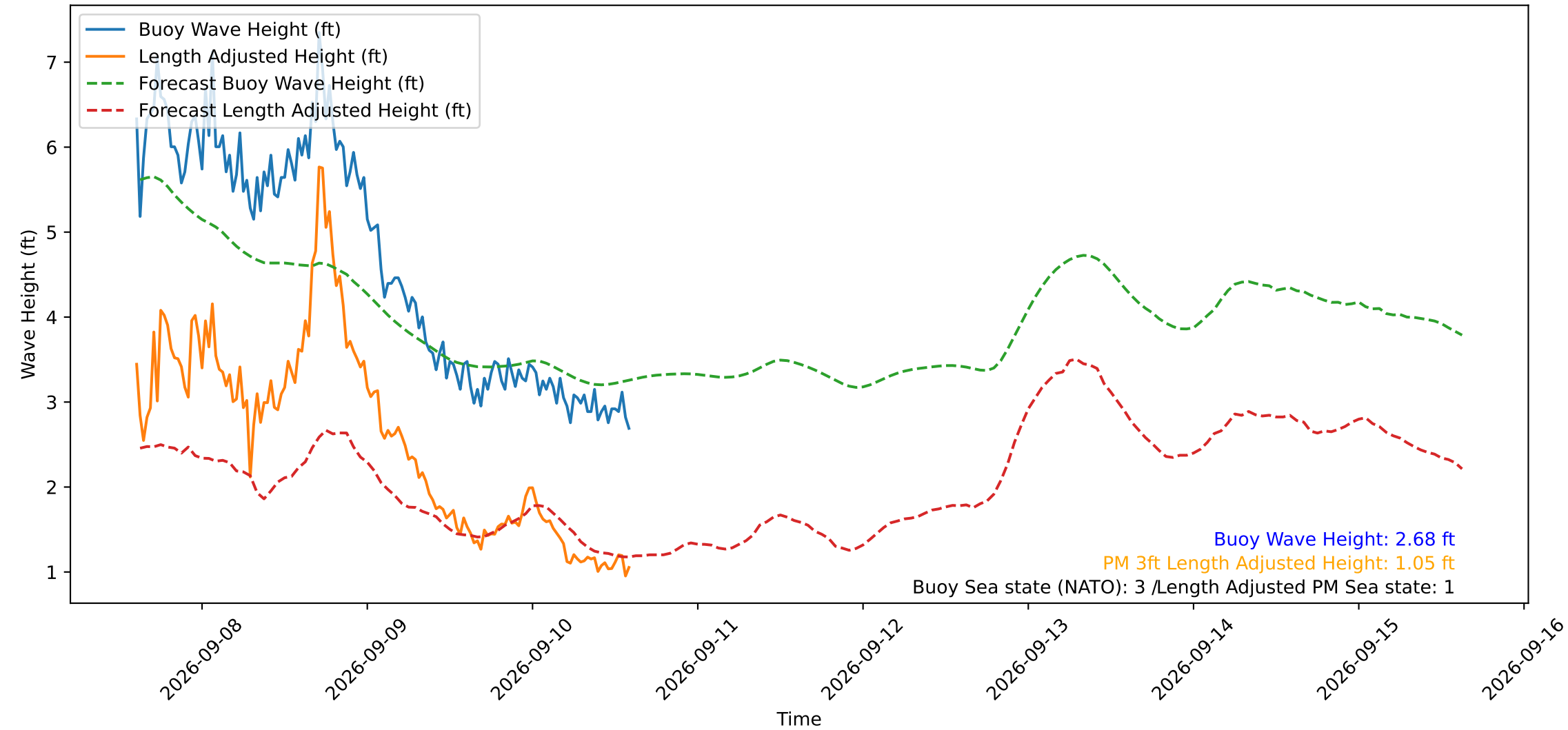
Wave Heights over Time for Oceanside Harbor at 2026-09-10 14:40:30
