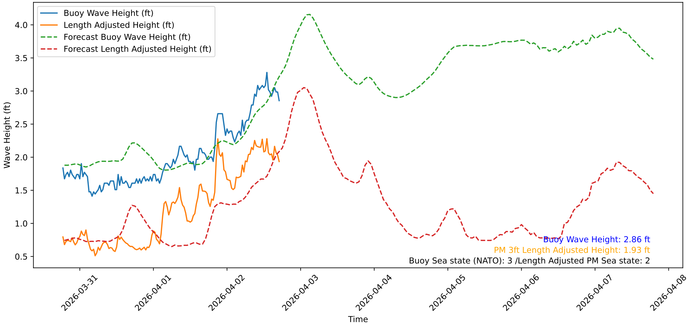
Wave Heights over Time for Green Beach at 2026-04-02 18:31:09
