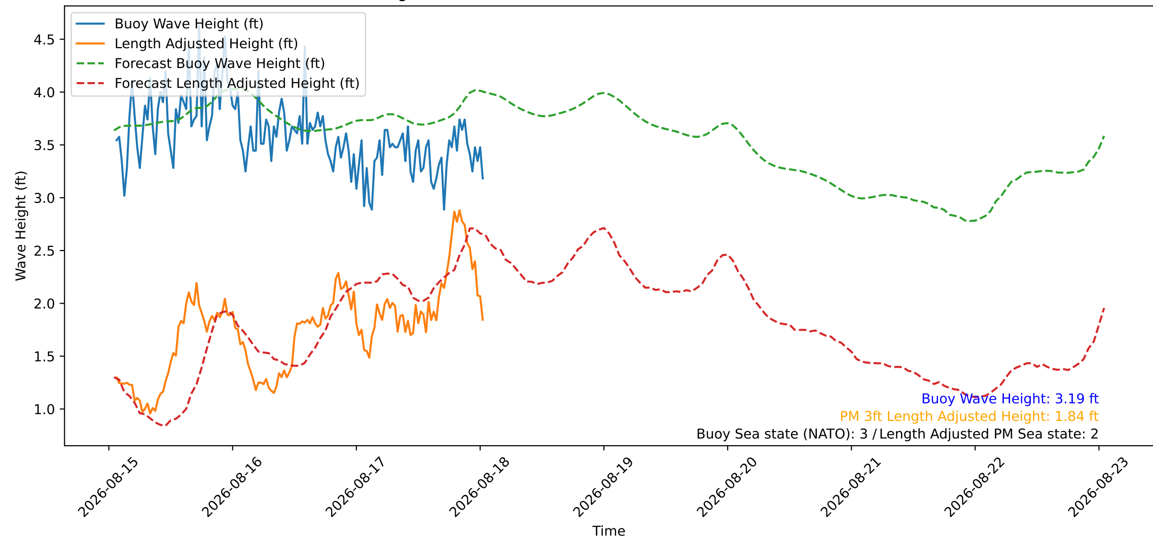
Wave Heights over Time for Oceanside Harbor at 2026-08-18 01:20:26
