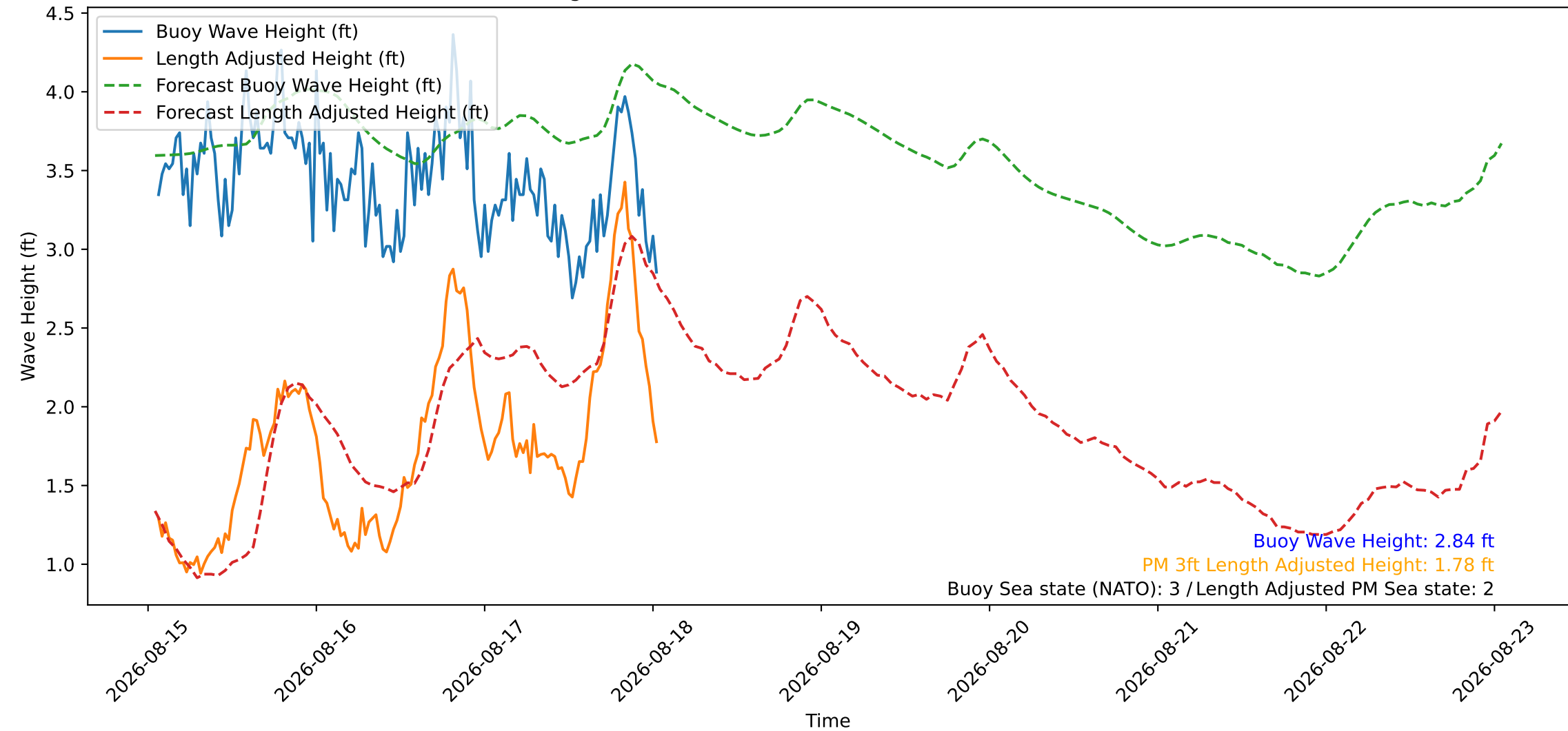
Wave Heights over Time for Green Beach at 2026-08-18 01:21:10
