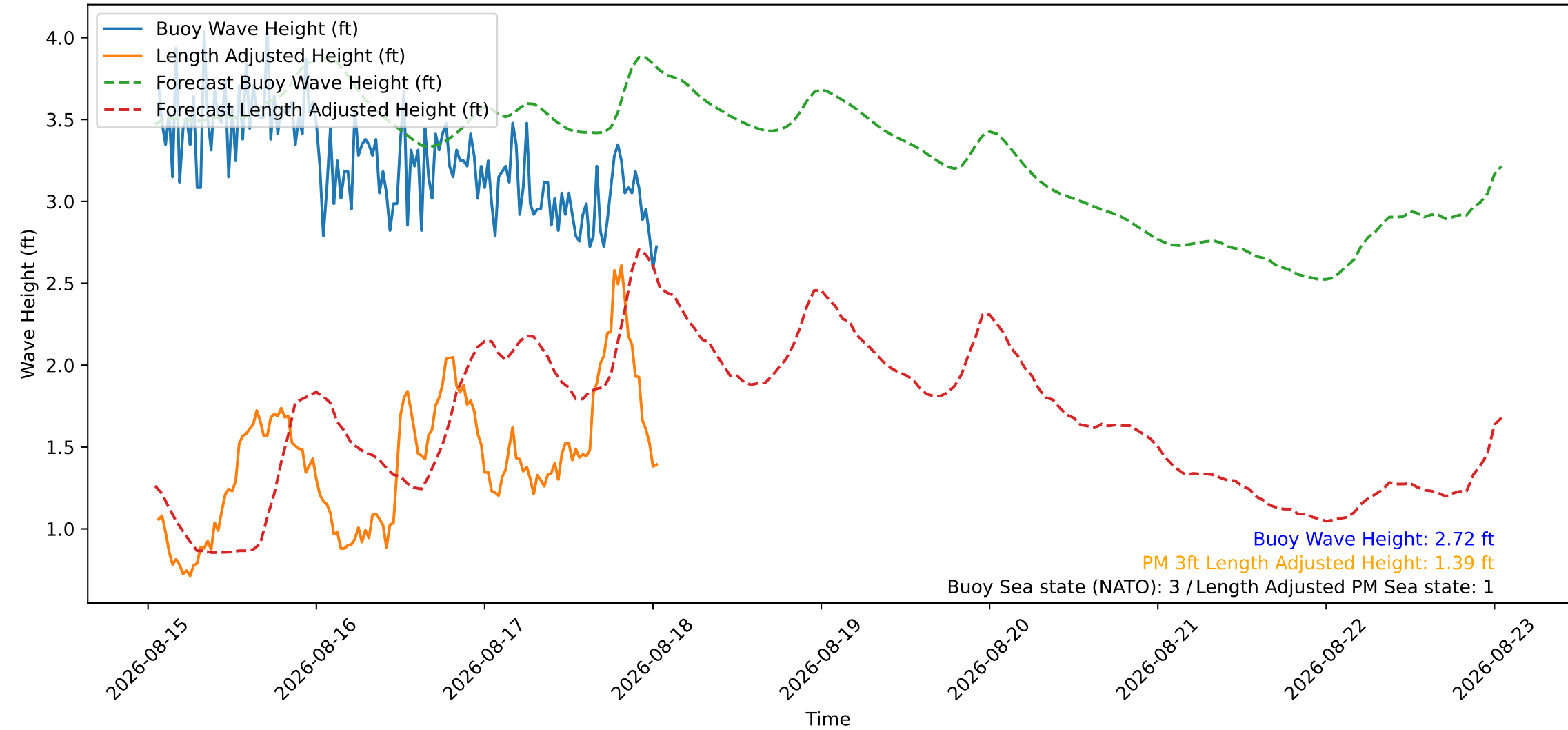
Wave Heights over Time for Red Beach at 2026-08-18 01:20:47
