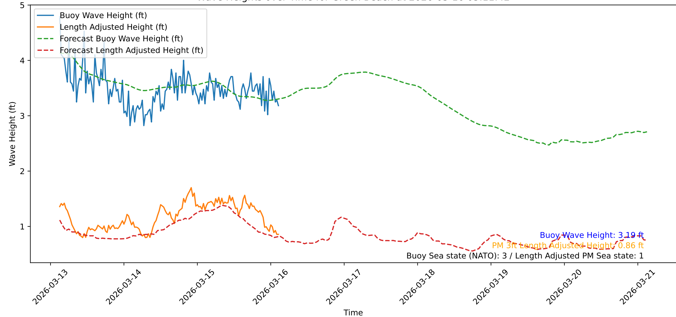
Wave Heights over Time for Green Beach at 2026-03-16 03:11:42
