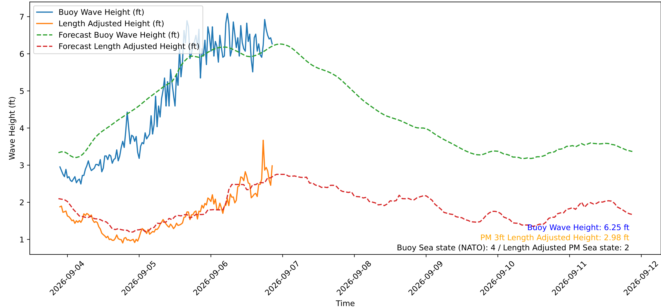
Wave Heights over Time for Green Beach at 2026-09-06 21:11:11
