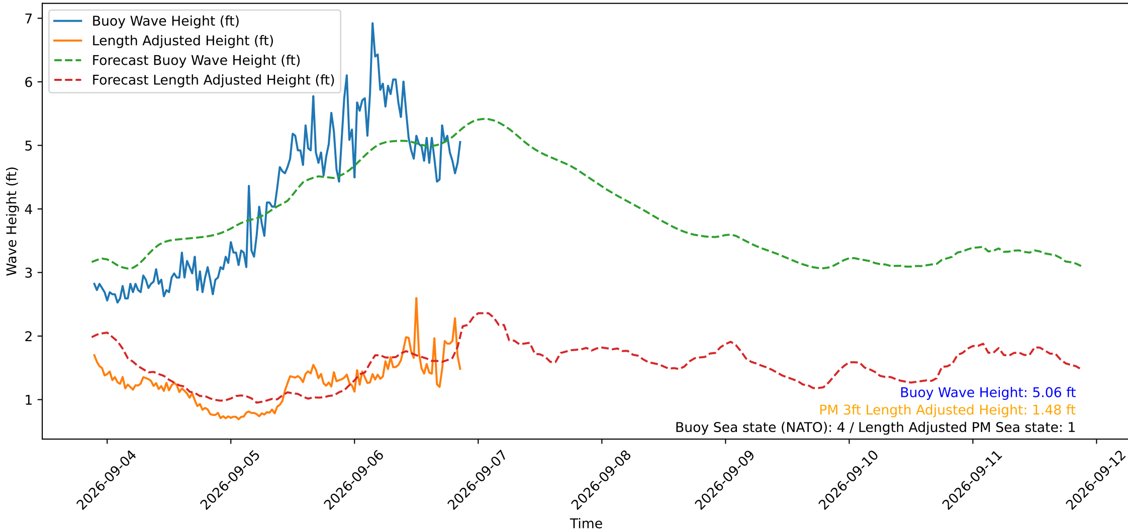
Wave Heights over Time for Red Beach at 2026-09-06 21:10:49
