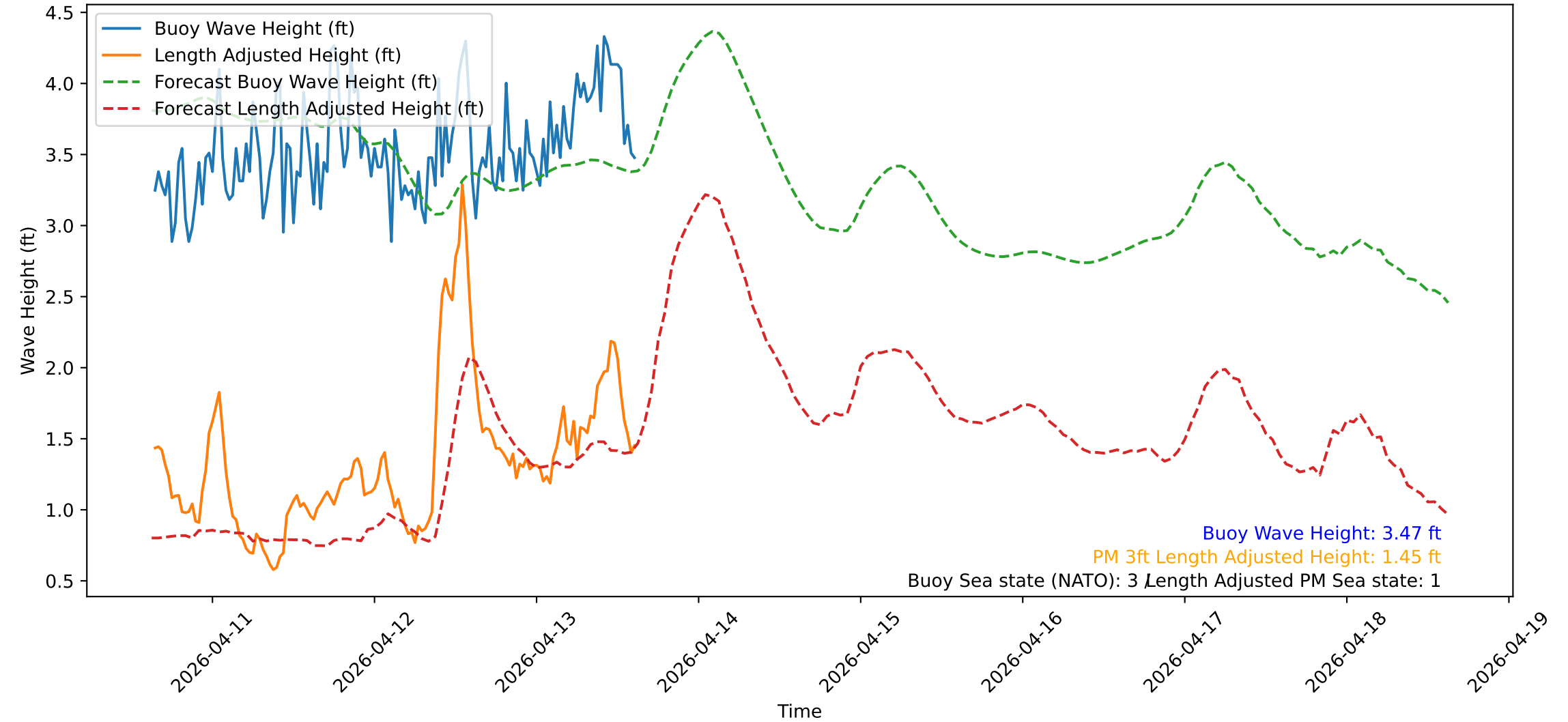
Wave Heights over Time for Red Beach at 2026-04-13 15:10:50
