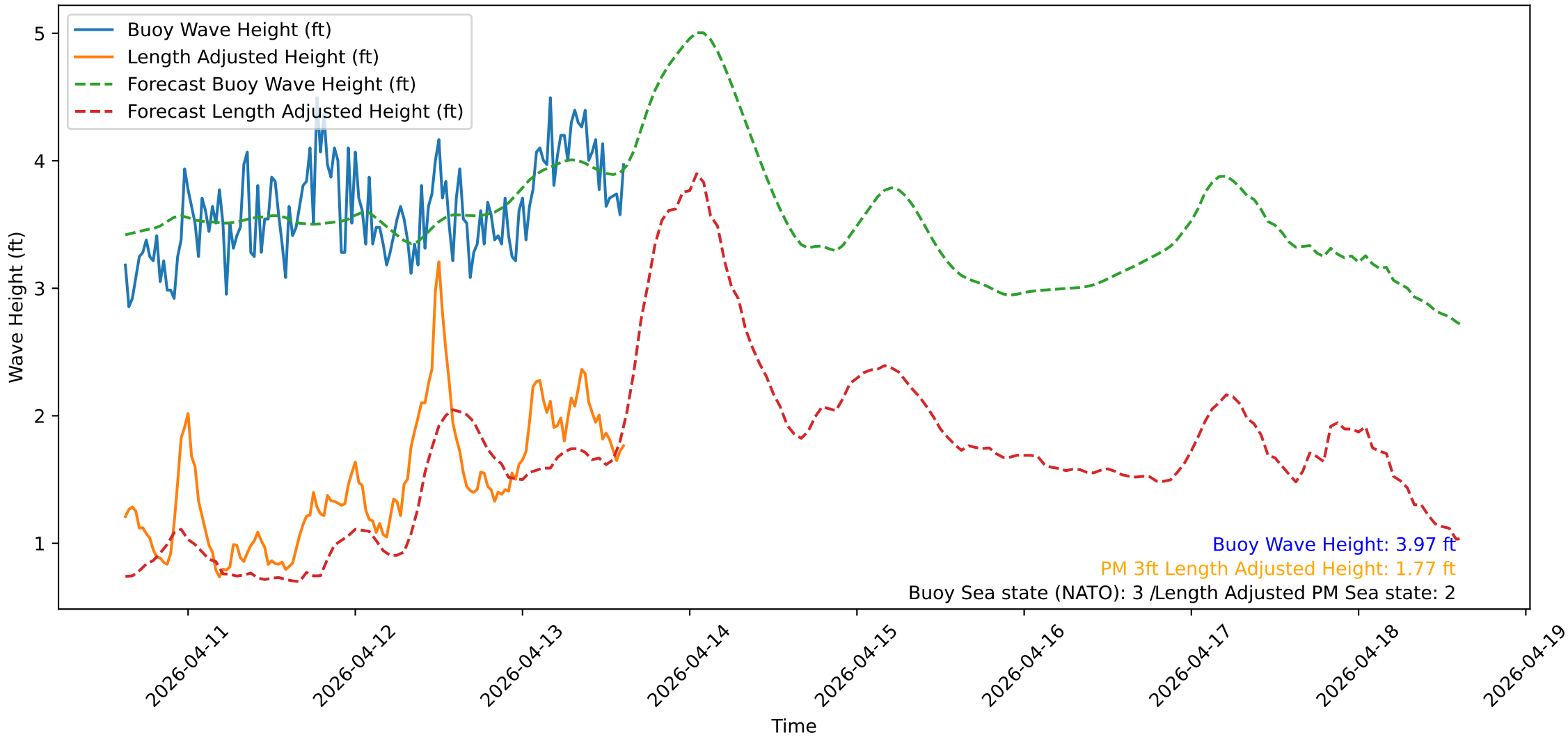
Wave Heights over Time for Green Beach at 2026-04-13 15:11:13
