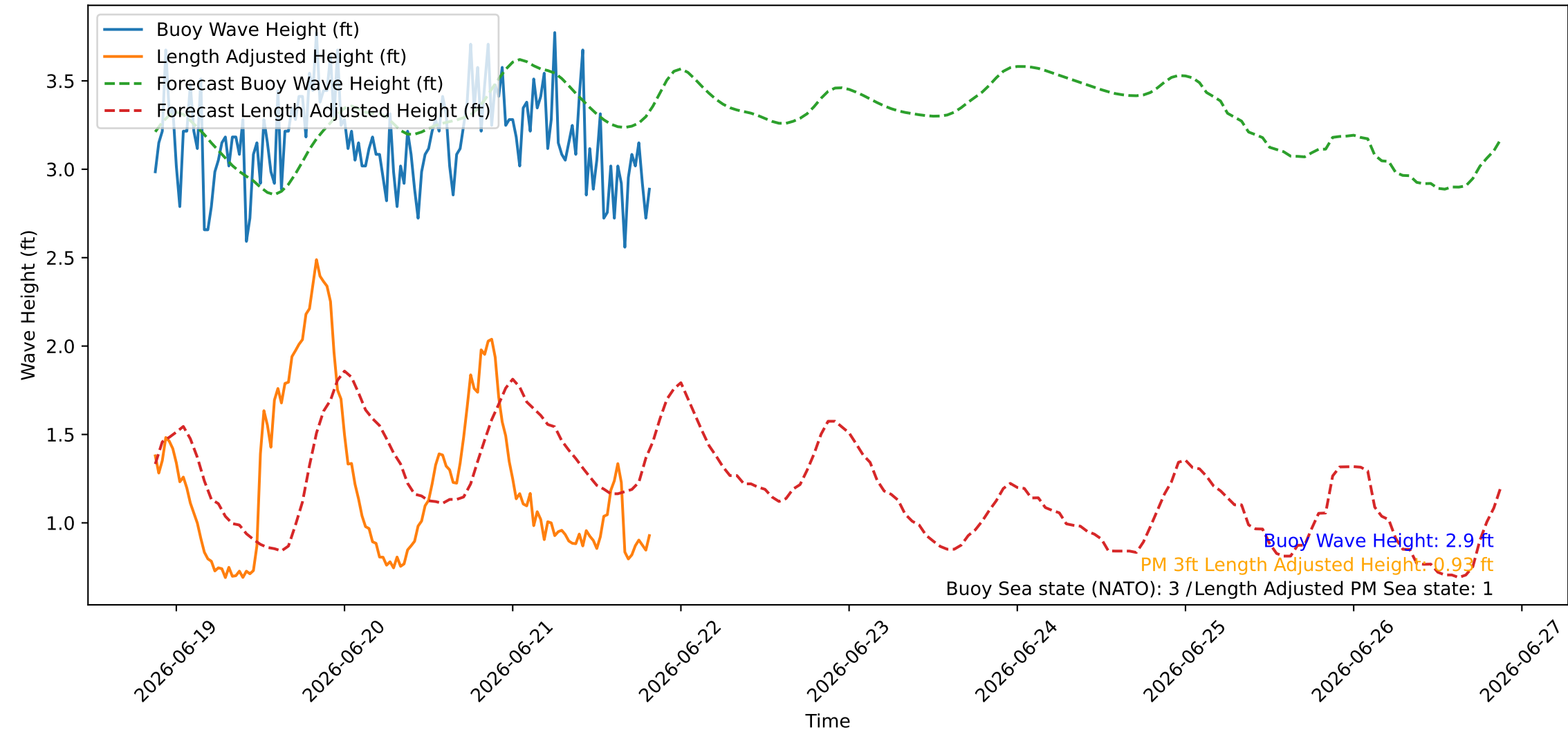
Wave Heights over Time for Red Beach at 2026-06-21 20:30:45
