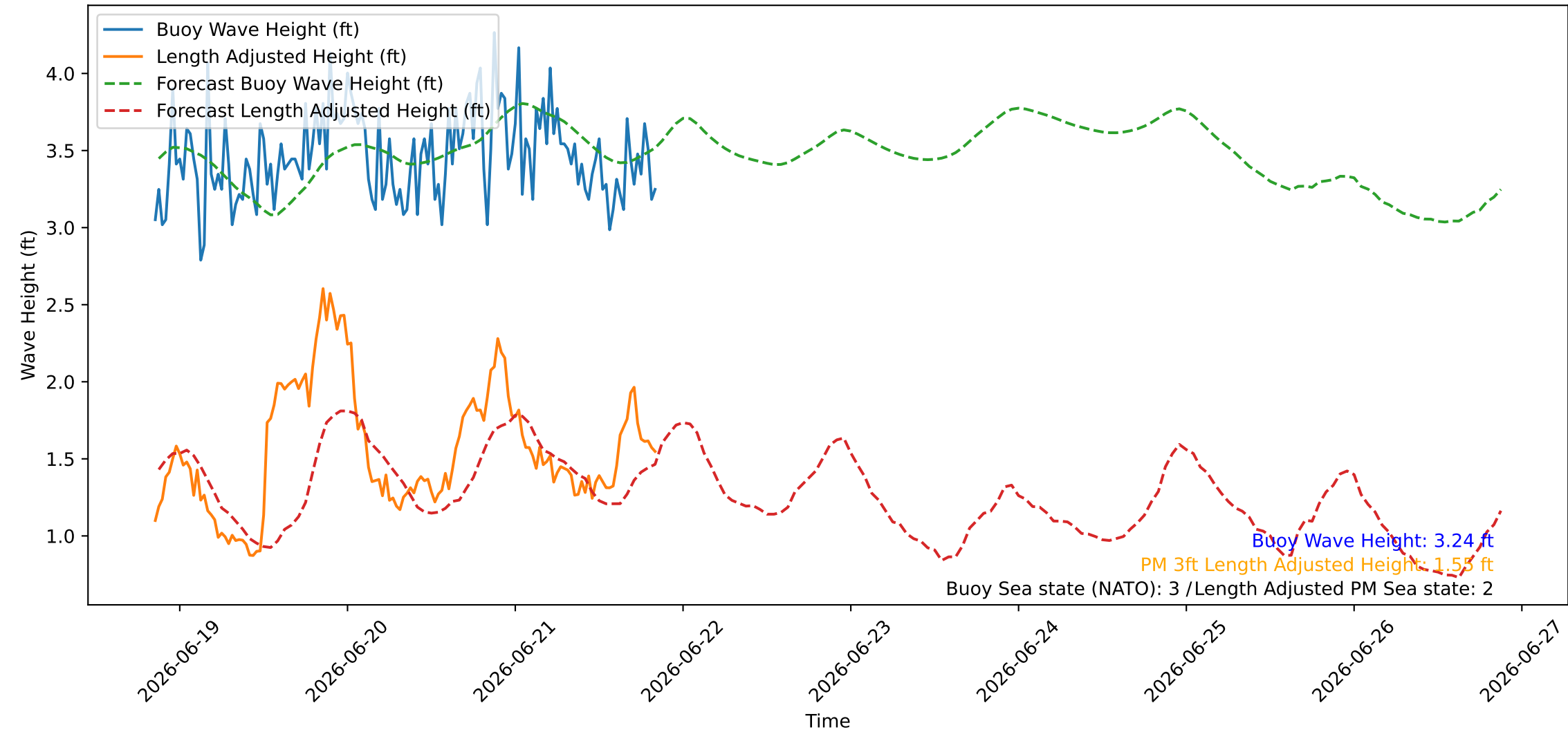
Wave Heights over Time for Oceanside Harbor at 2026-06-21 20:30:26
