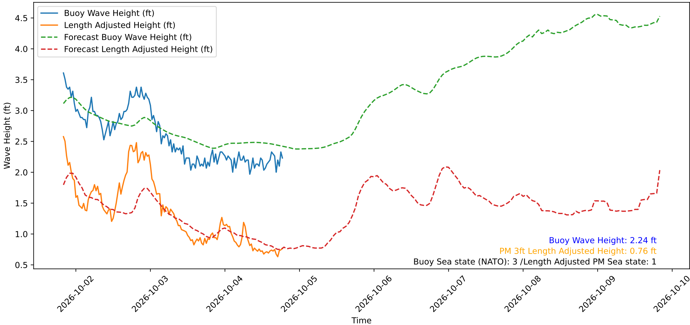
Wave Heights over Time for Green Beach at 2026-10-04 19:31:12
