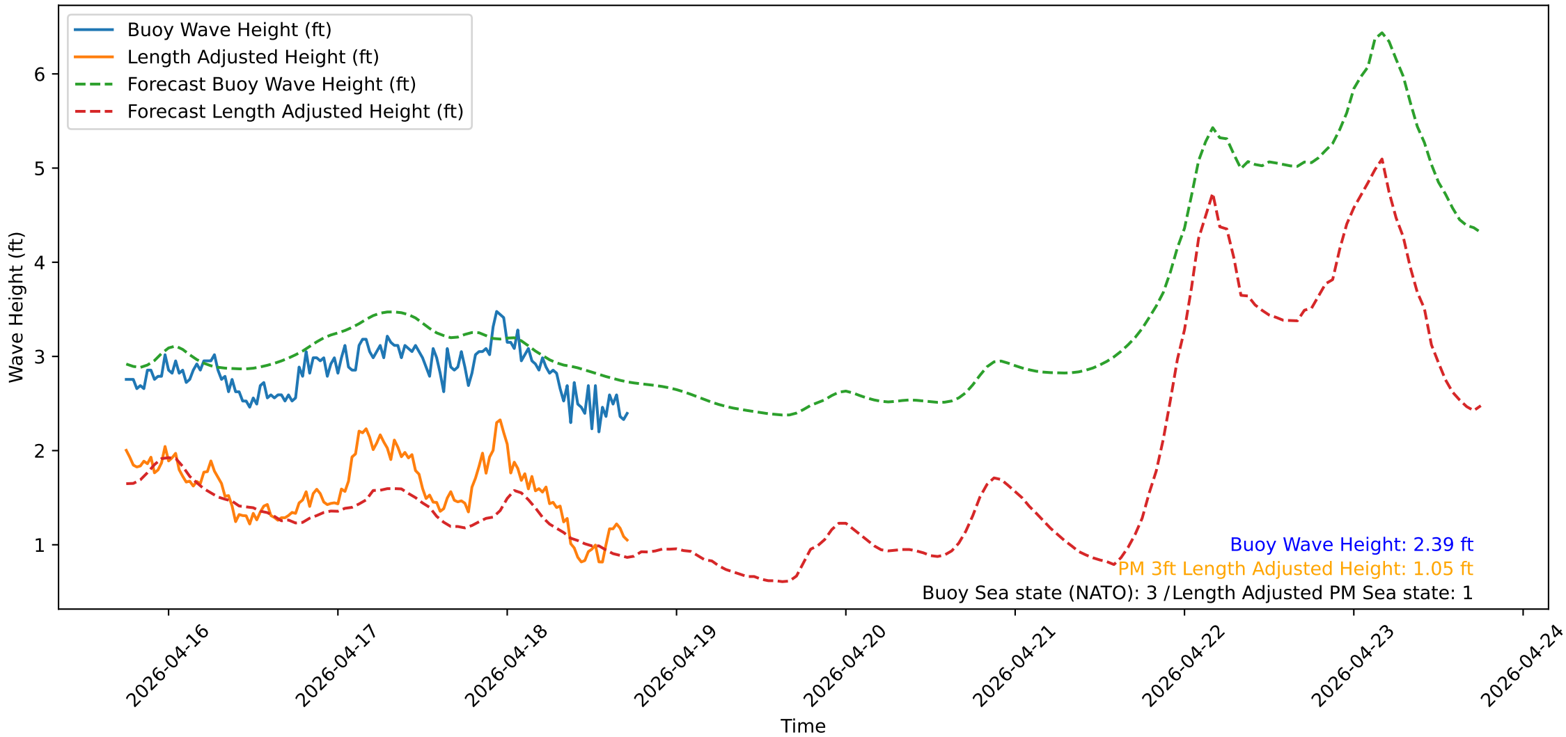
Wave Heights over Time for Green Beach at 2026-04-18 18:11:13
