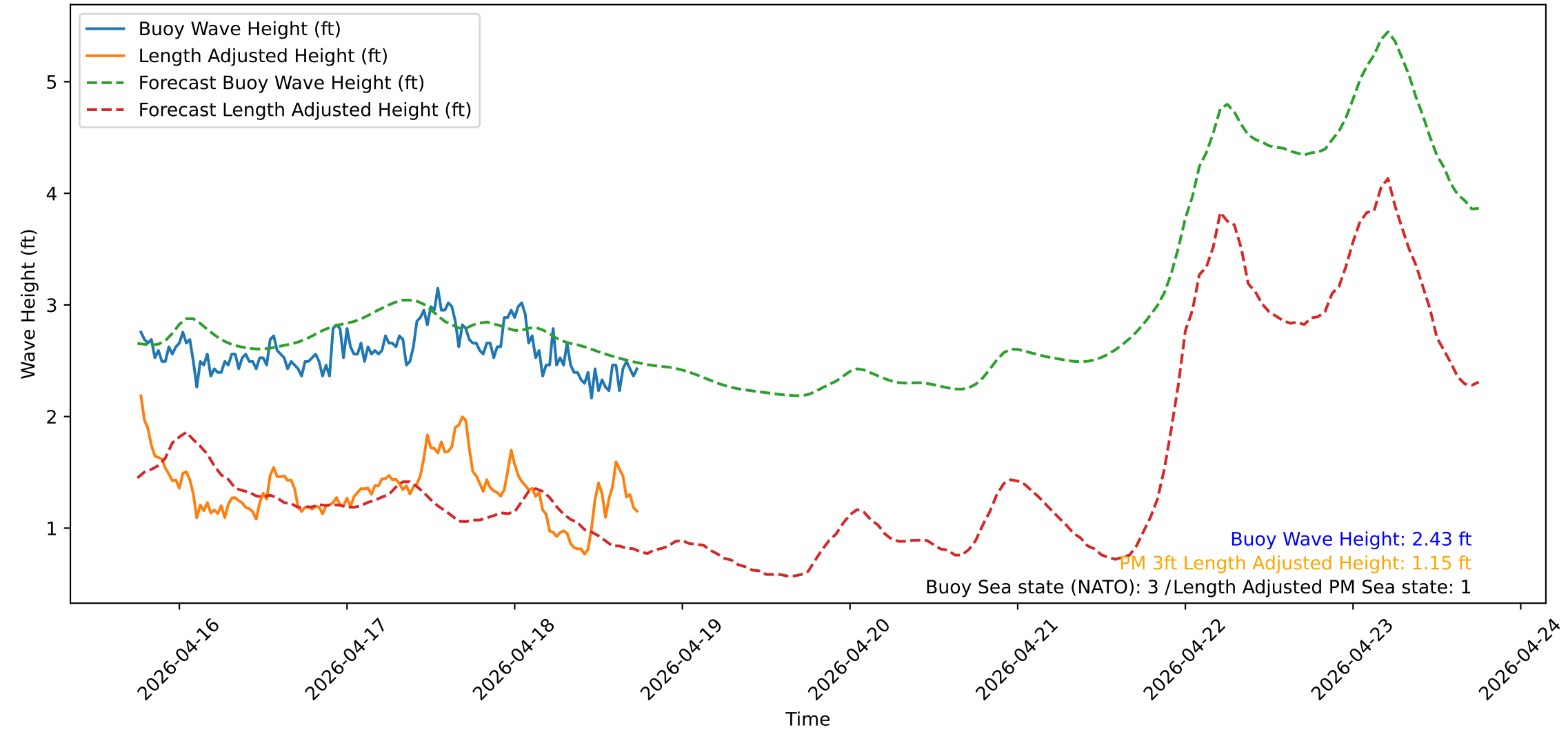
Wave Heights over Time for Red Beach at 2026-04-18 18:10:50
