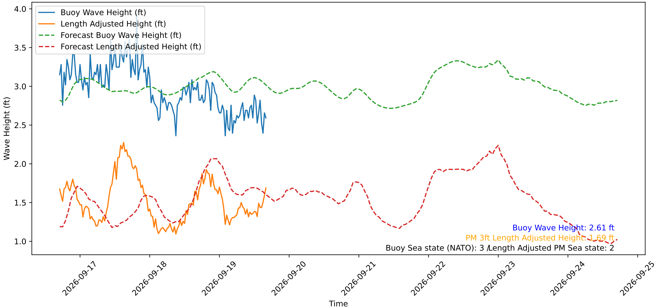
Wave Heights over Time for Oceanside Harbor at 2026-09-19 17:10:30
