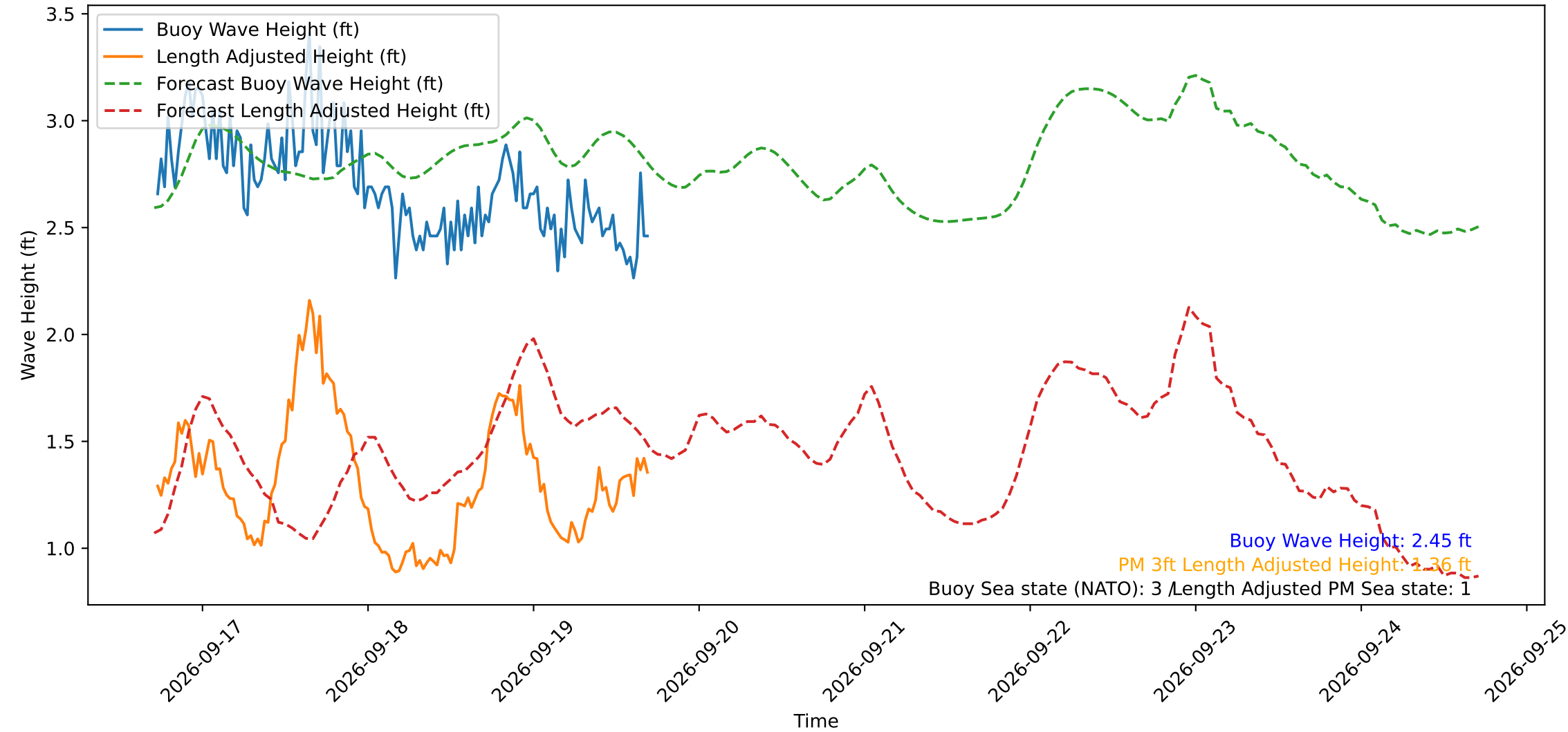
Wave Heights over Time for Red Beach at 2026-09-19 17:10:49
