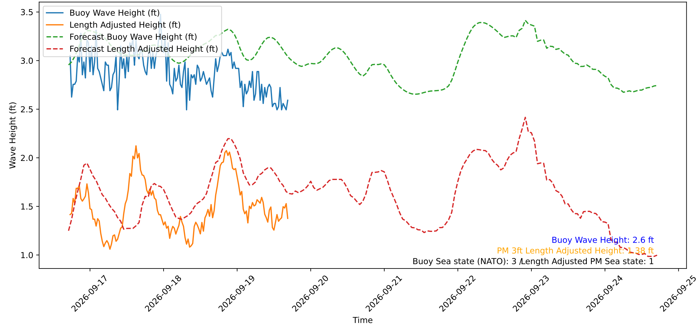
Wave Heights over Time for Green Beach at 2026-09-19 17:11:12
