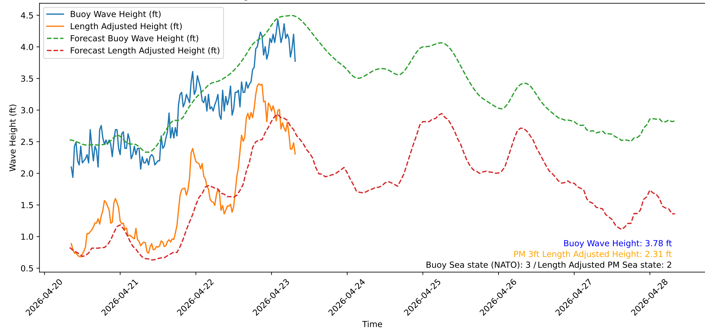
Wave Heights over Time for Oceanside Harbor at 2026-04-23 08:20:30
