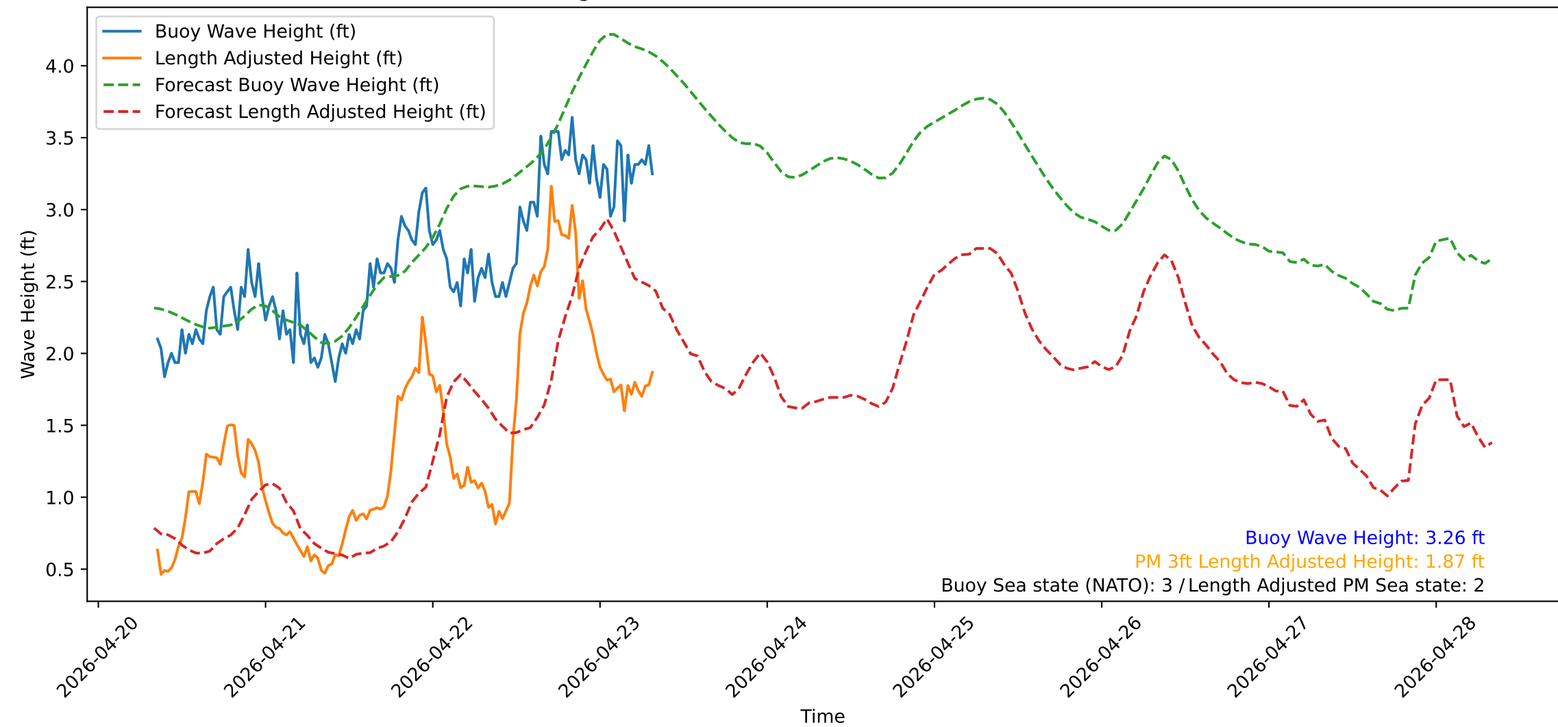
Wave Heights over Time for Red Beach at 2026-04-23 08:20:51
