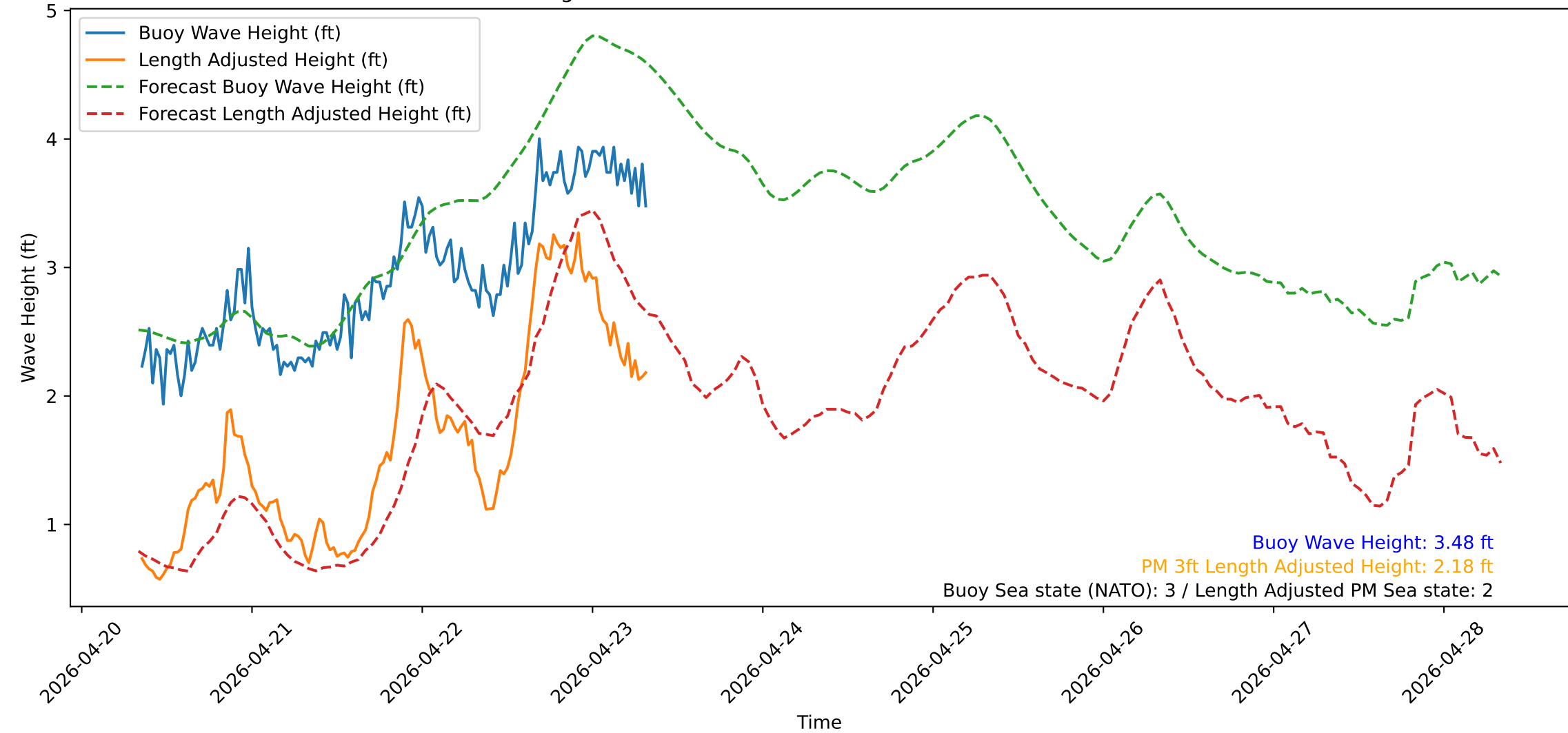
Wave Heights over Time for Green Beach at 2026-04-23 08:21:13
