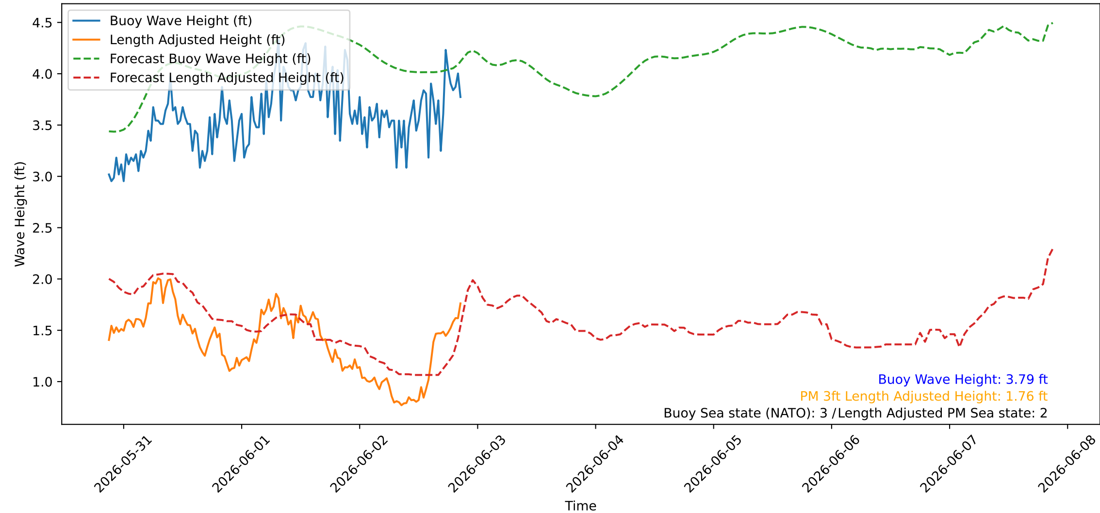
Wave Heights over Time for Green Beach at 2026-06-02 21:11:07
