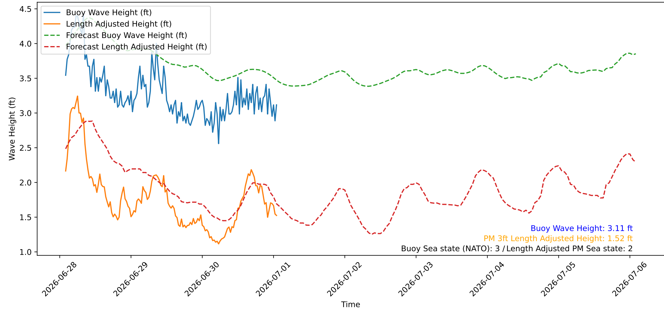
Wave Heights over Time for Oceanside Harbor at 2026-07-01 01:50:25
