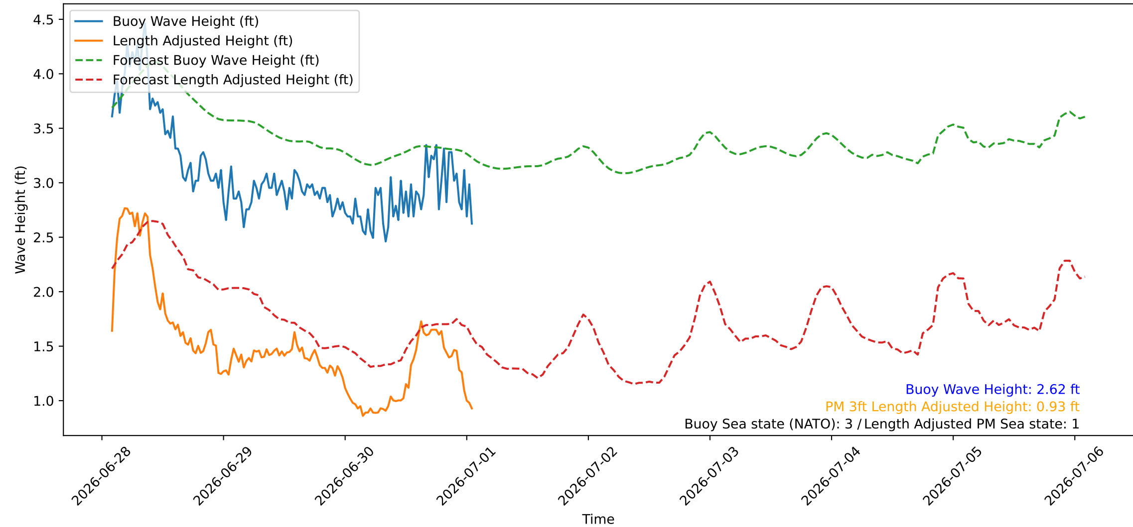
Wave Heights over Time for Red Beach at 2026-07-01 01:50:46
