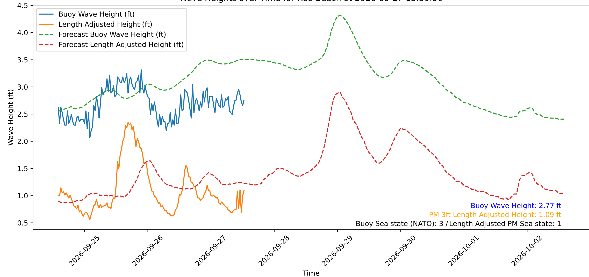
Wave Heights over Time for Red Beach at 2026-09-27 13:30:50
