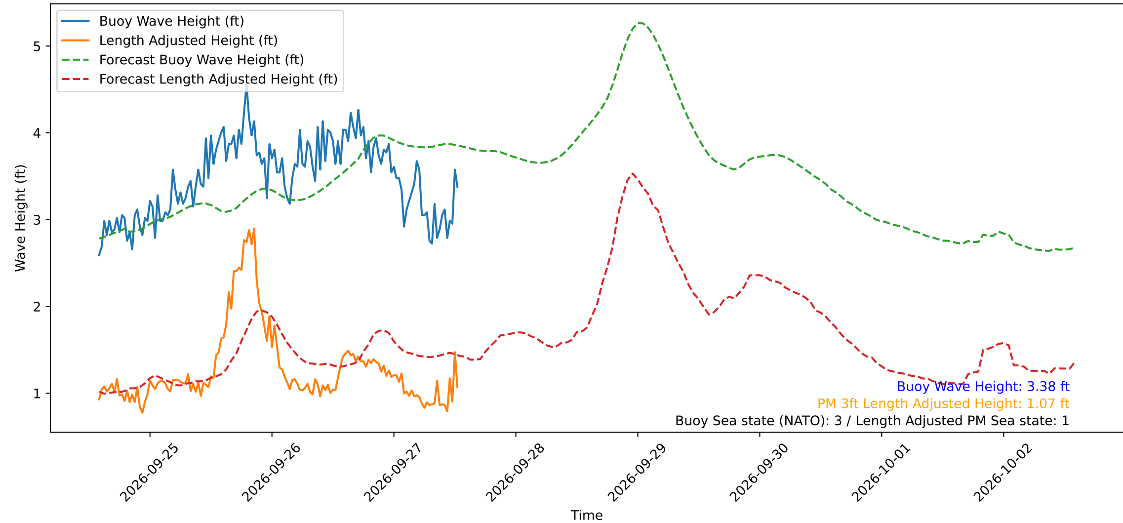
Wave Heights over Time for Green Beach at 2026-09-27 13:31:12
