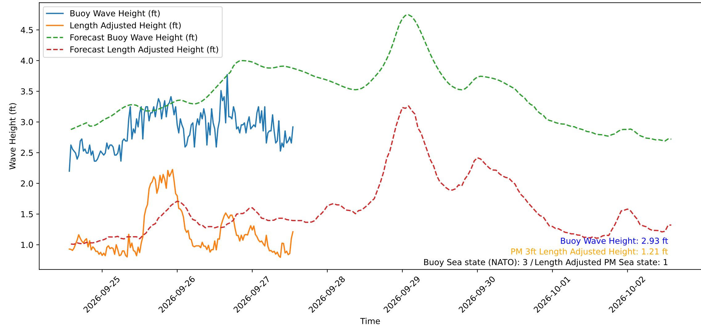
Wave Heights over Time for Oceanside Harbor at 2026-09-27 13:30:30
