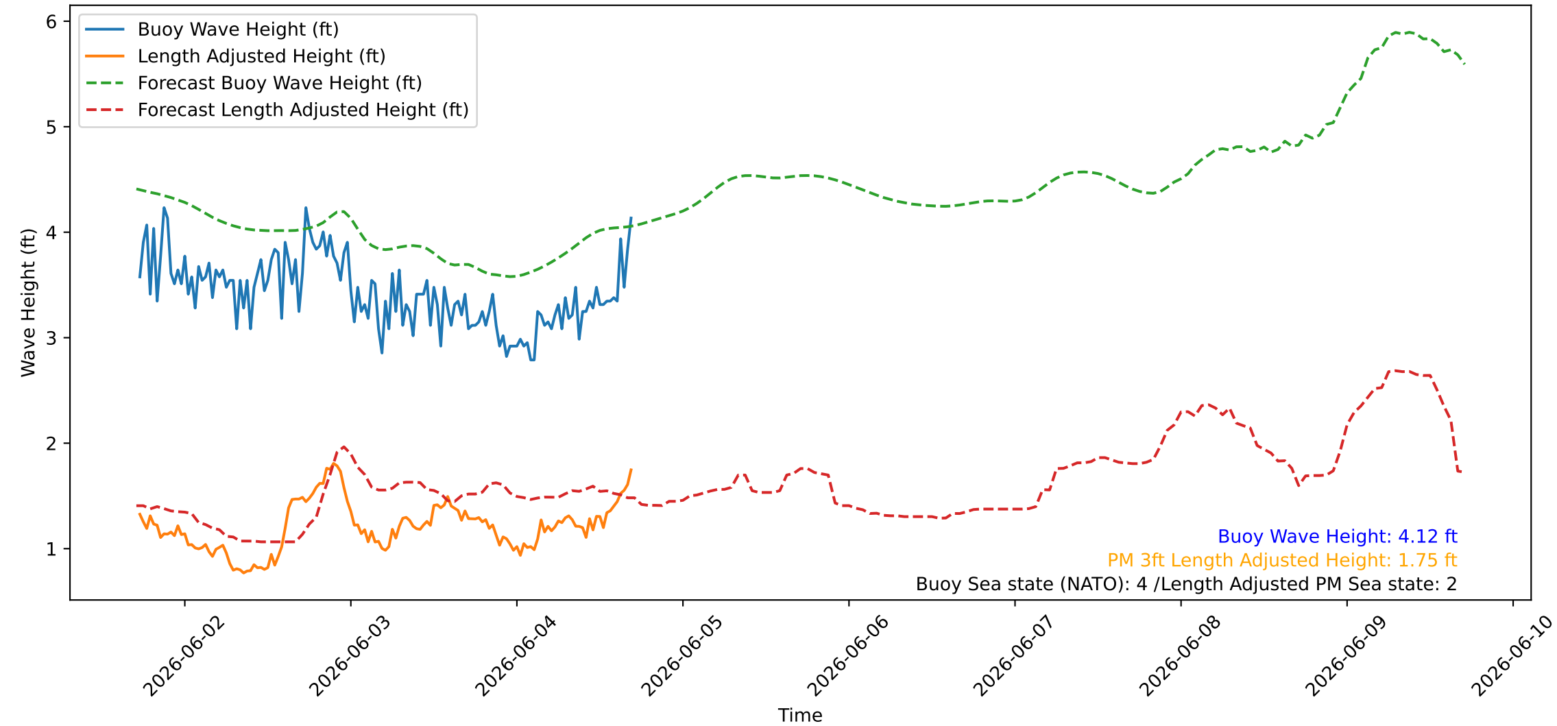
Wave Heights over Time for Green Beach at 2026-06-04 17:21:09
