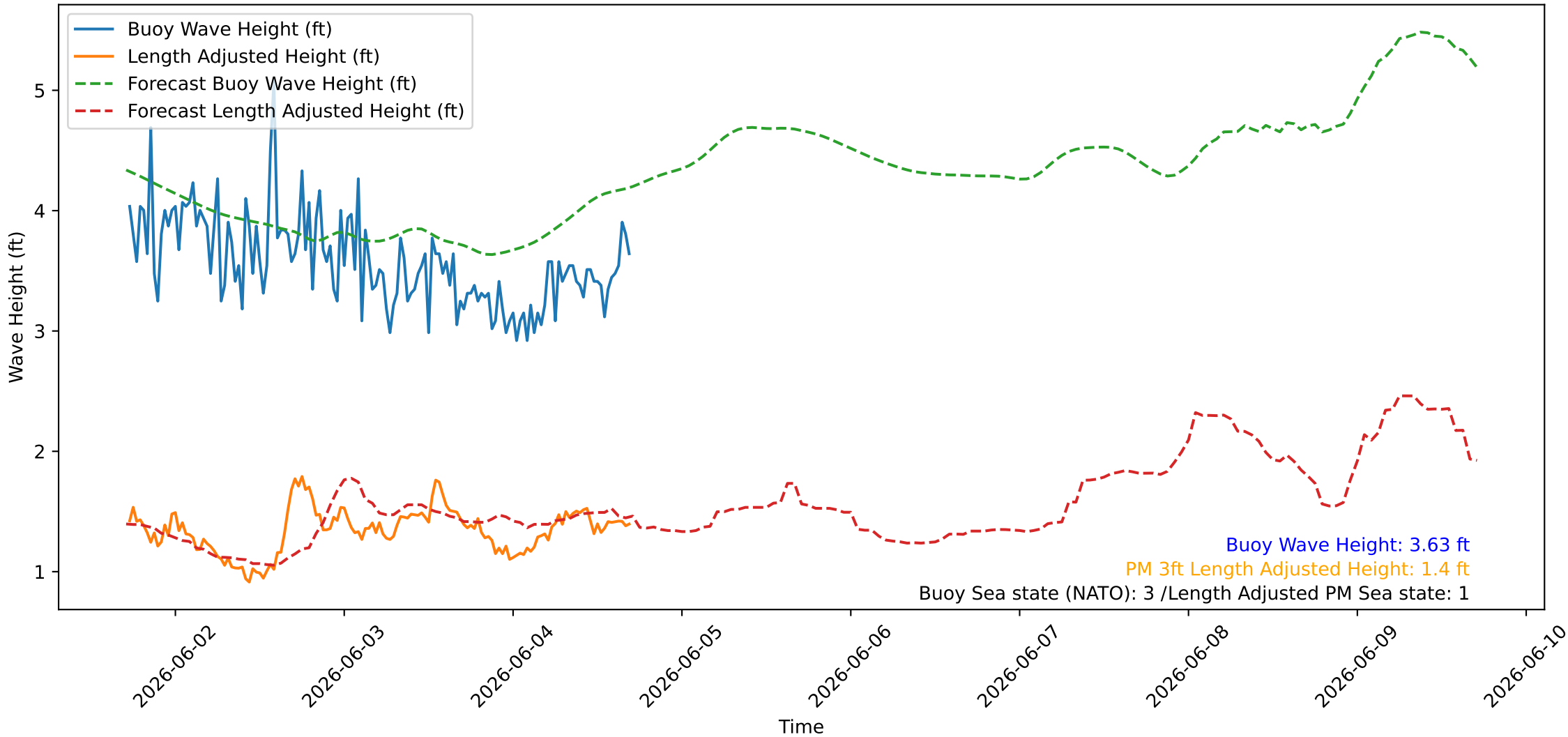
Wave Heights over Time for Oceanside Harbor at 2026-06-04 17:20:26
