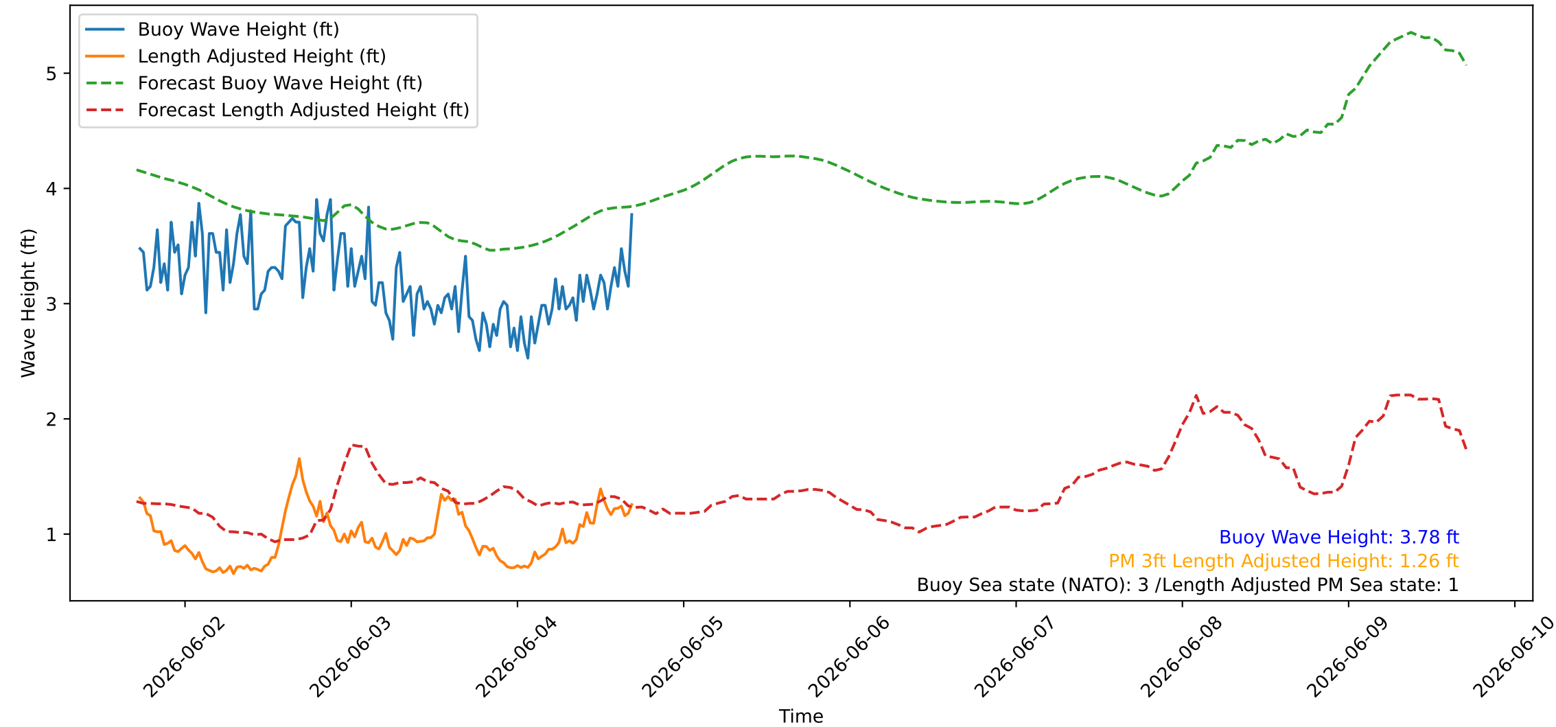
Wave Heights over Time for Red Beach at 2026-06-04 17:20:46
