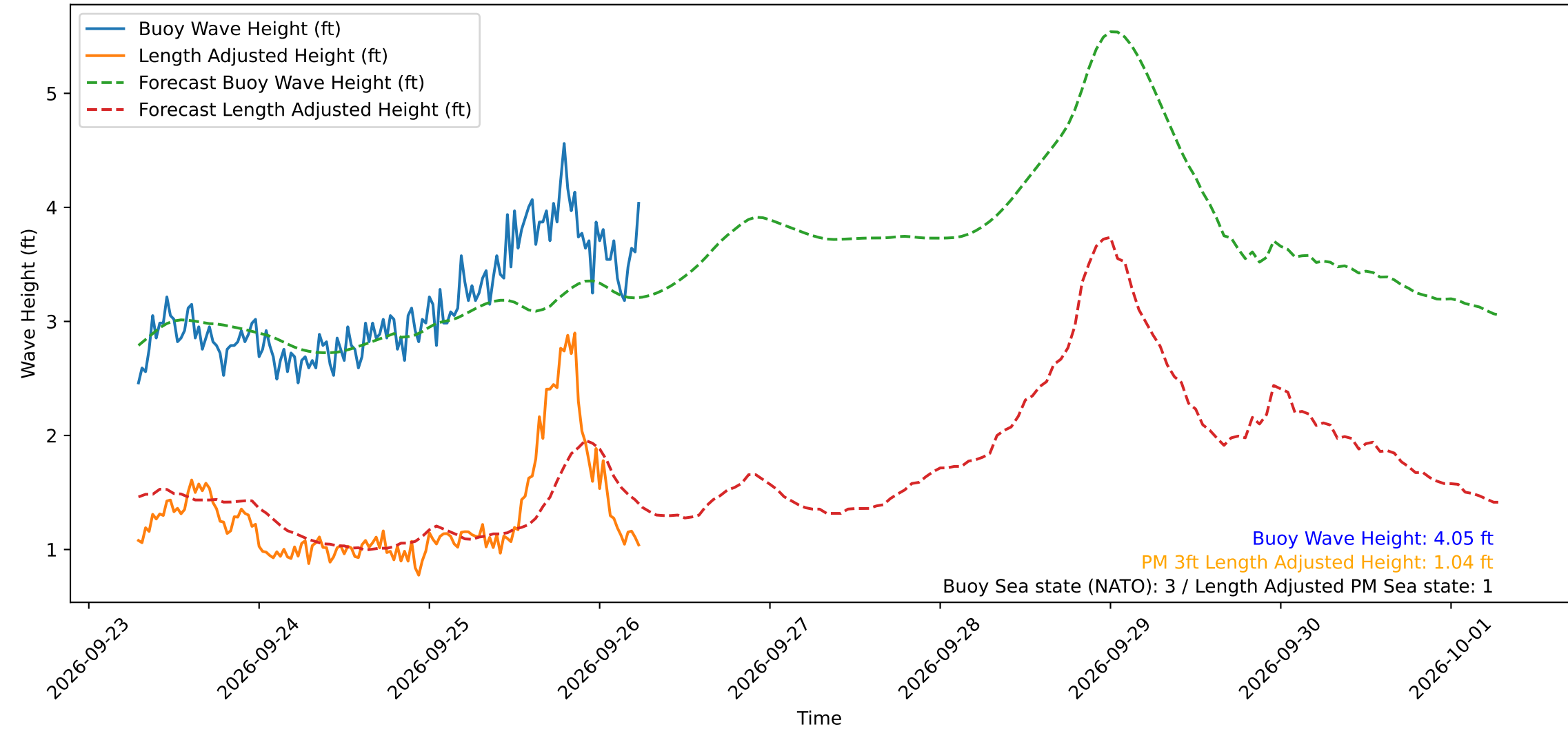
Wave Heights over Time for Green Beach at 2026-09-26 06:51:14
