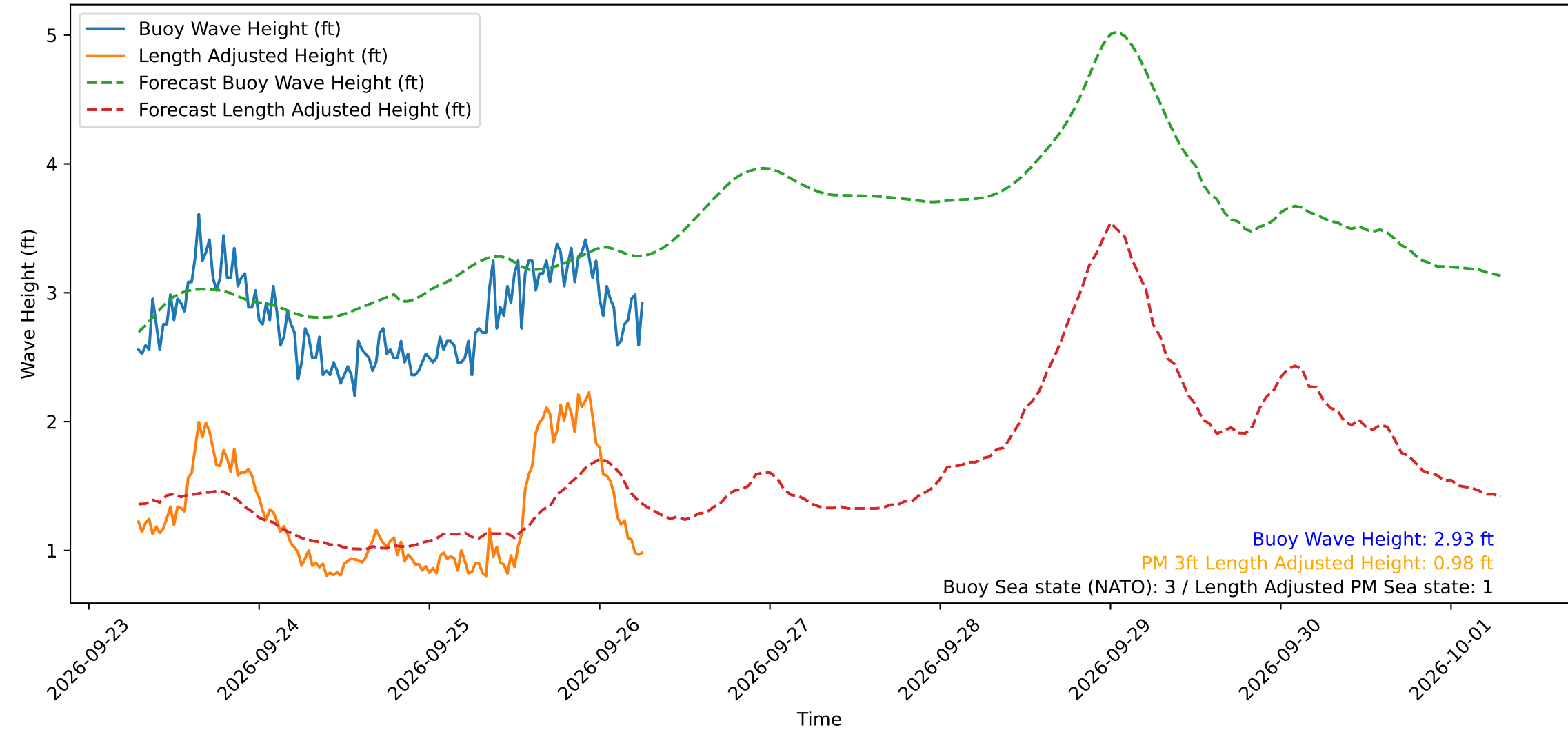
Wave Heights over Time for Oceanside Harbor at 2026-09-26 06:50:29
