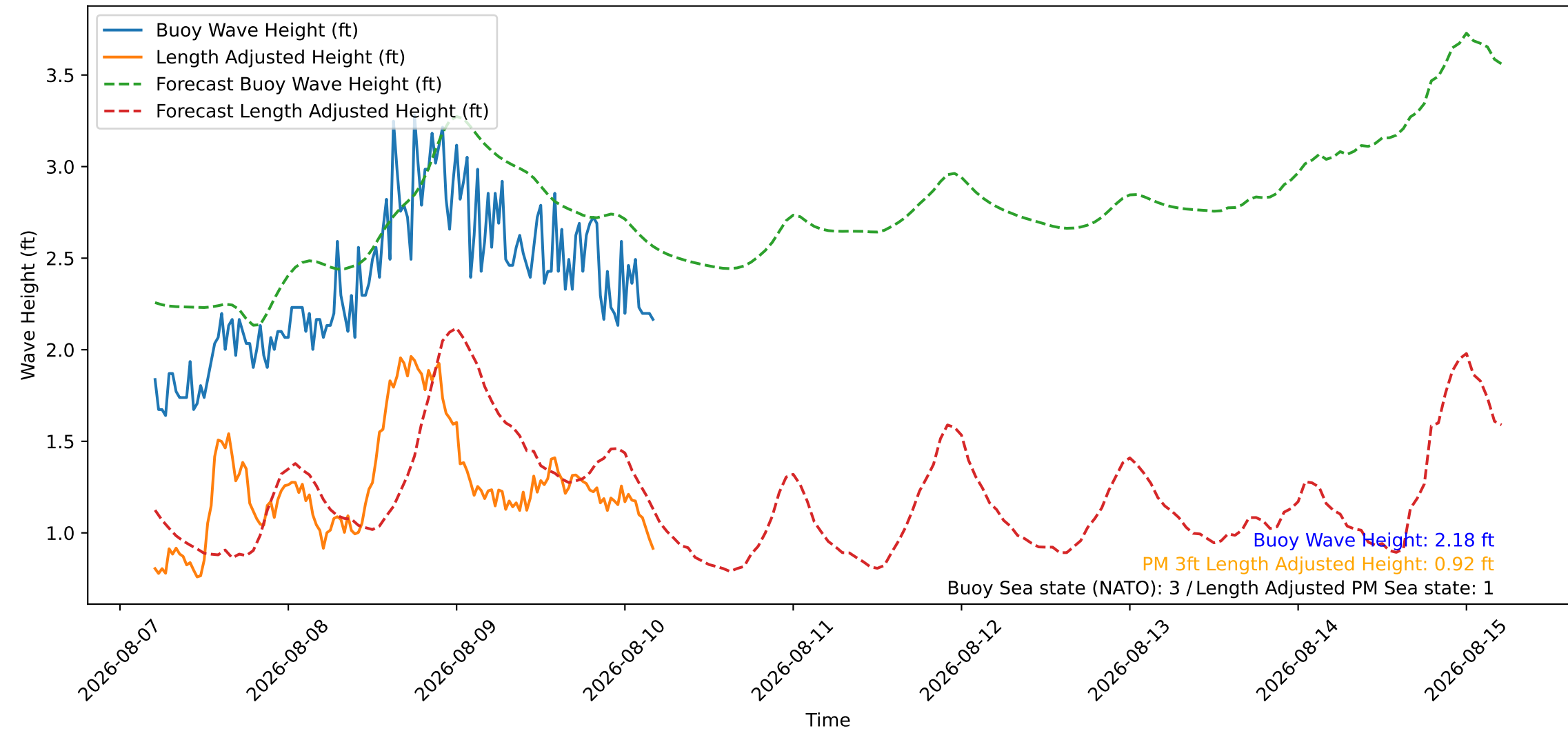
Wave Heights over Time for Oceanside Harbor at 2026-08-10 04:50:26
