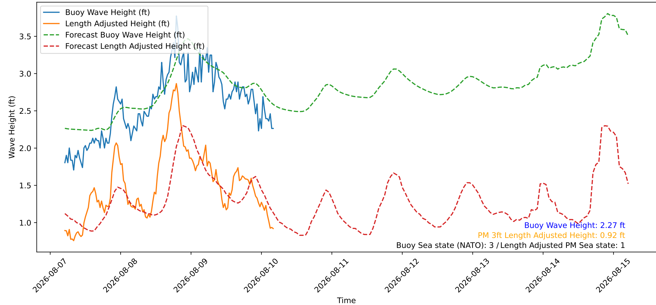
Wave Heights over Time for Green Beach at 2026-08-10 04:51:10
