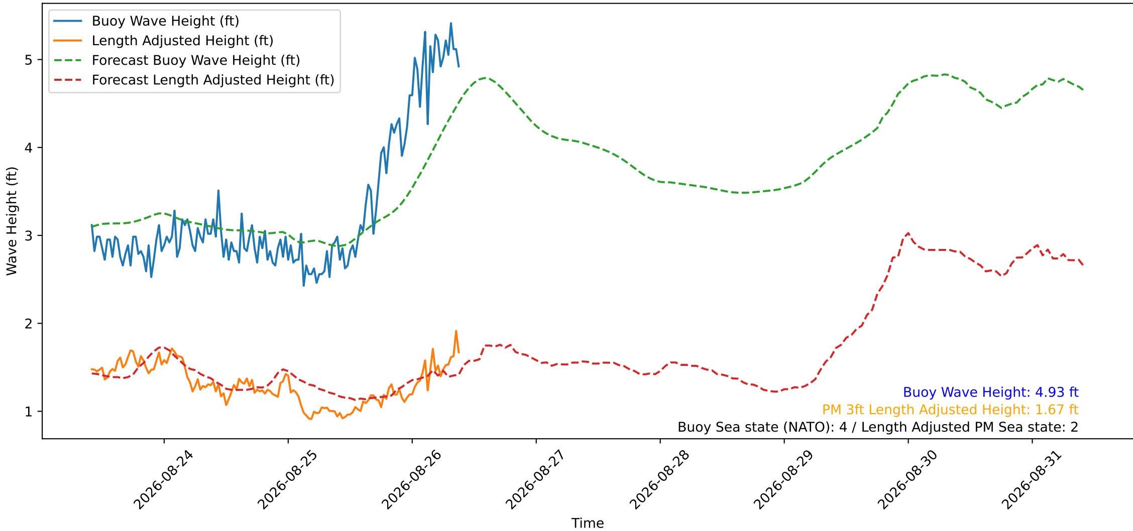
Wave Heights over Time for Oceanside Harbor at 2026-08-26 10:00:31
