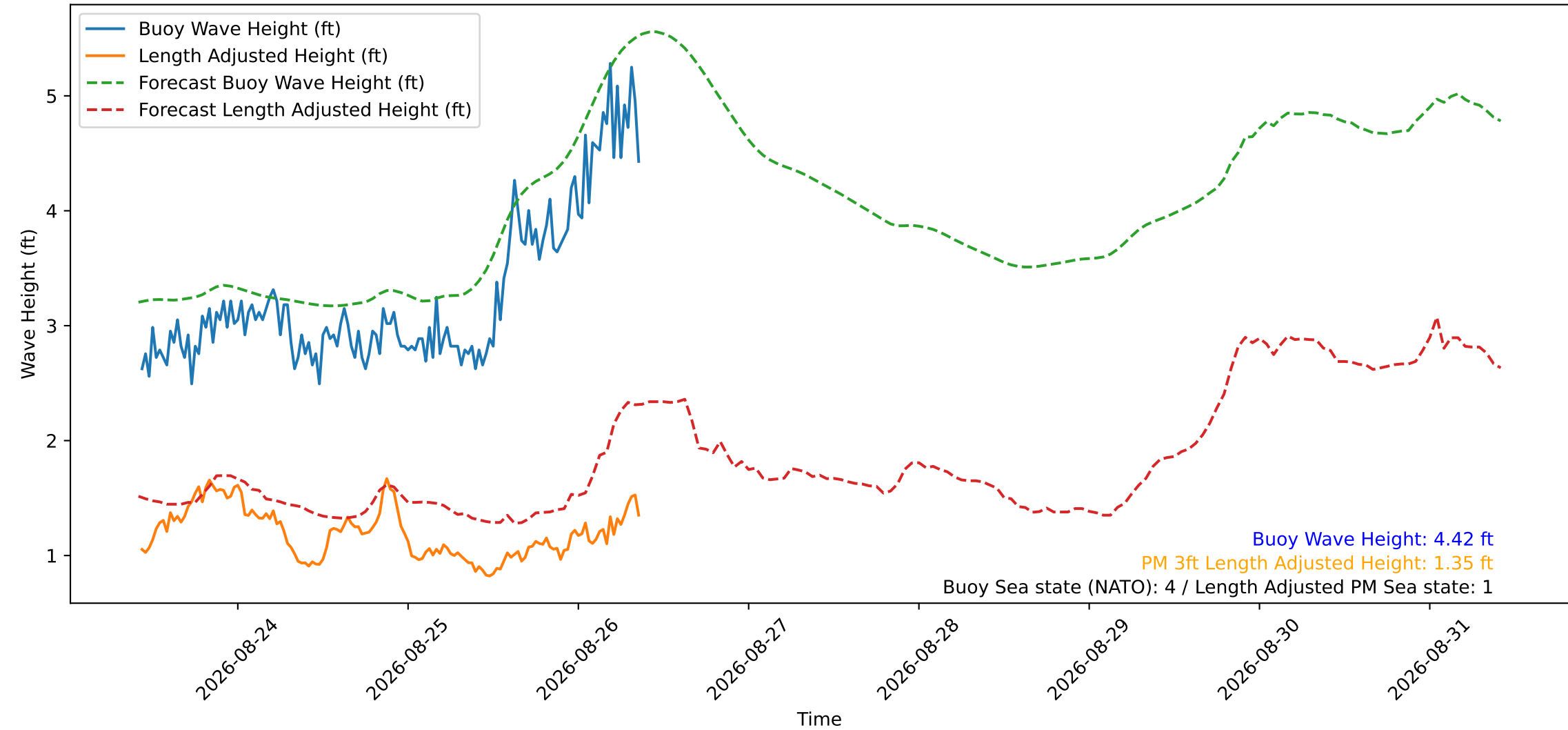
Wave Heights over Time for Green Beach at 2026-08-26 10:01:17
