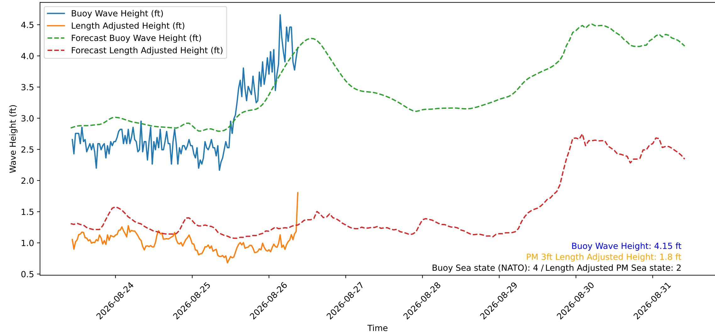
Wave Heights over Time for Red Beach at 2026-08-26 10:00:53
