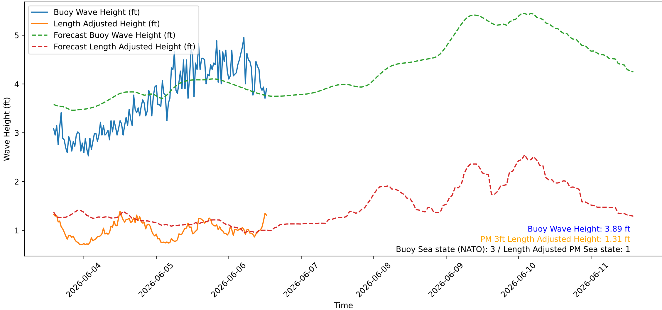
Wave Heights over Time for Red Beach at 2026-06-06 13:30:45
