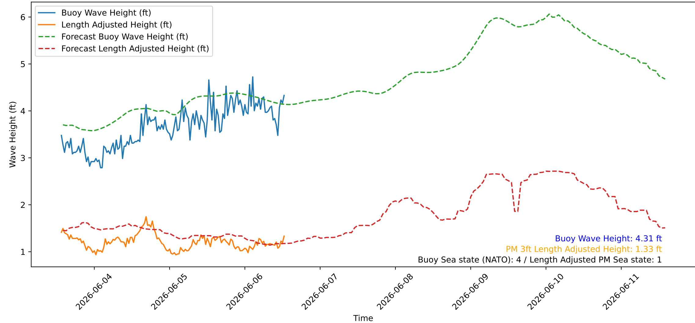
Wave Heights over Time for Green Beach at 2026-06-06 13:31:07
