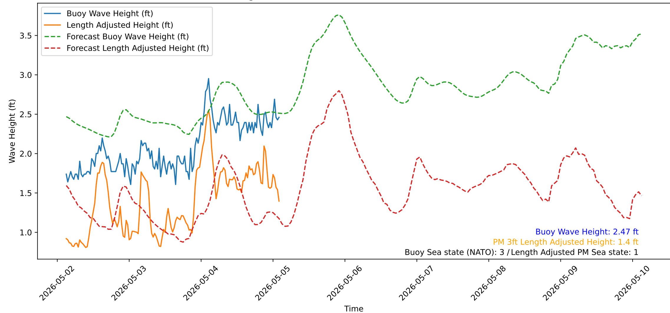
Wave Heights over Time for Red Beach at 2026-05-05 02:50:52
