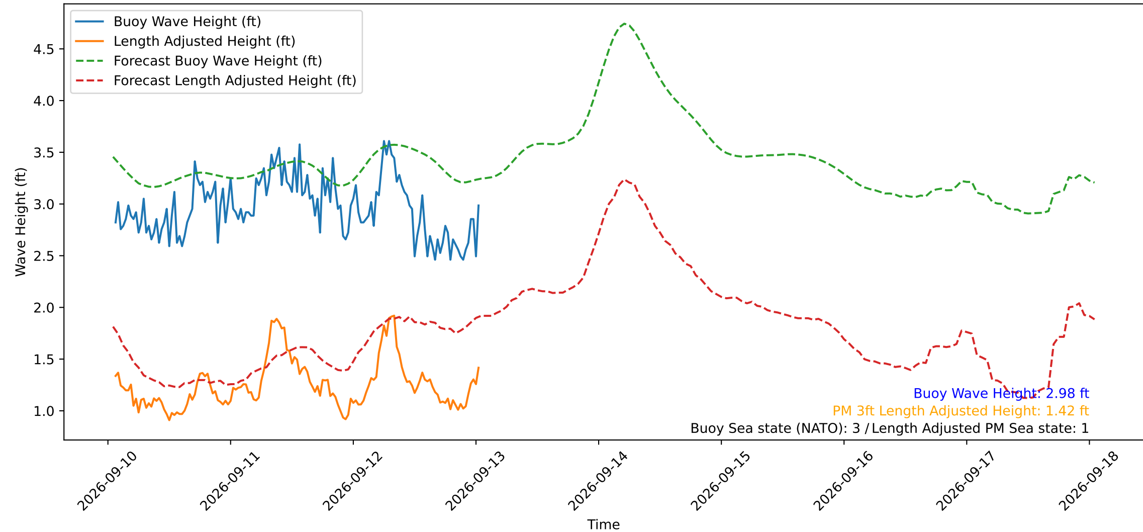
Wave Heights over Time for Green Beach at 2026-09-13 01:11:12
