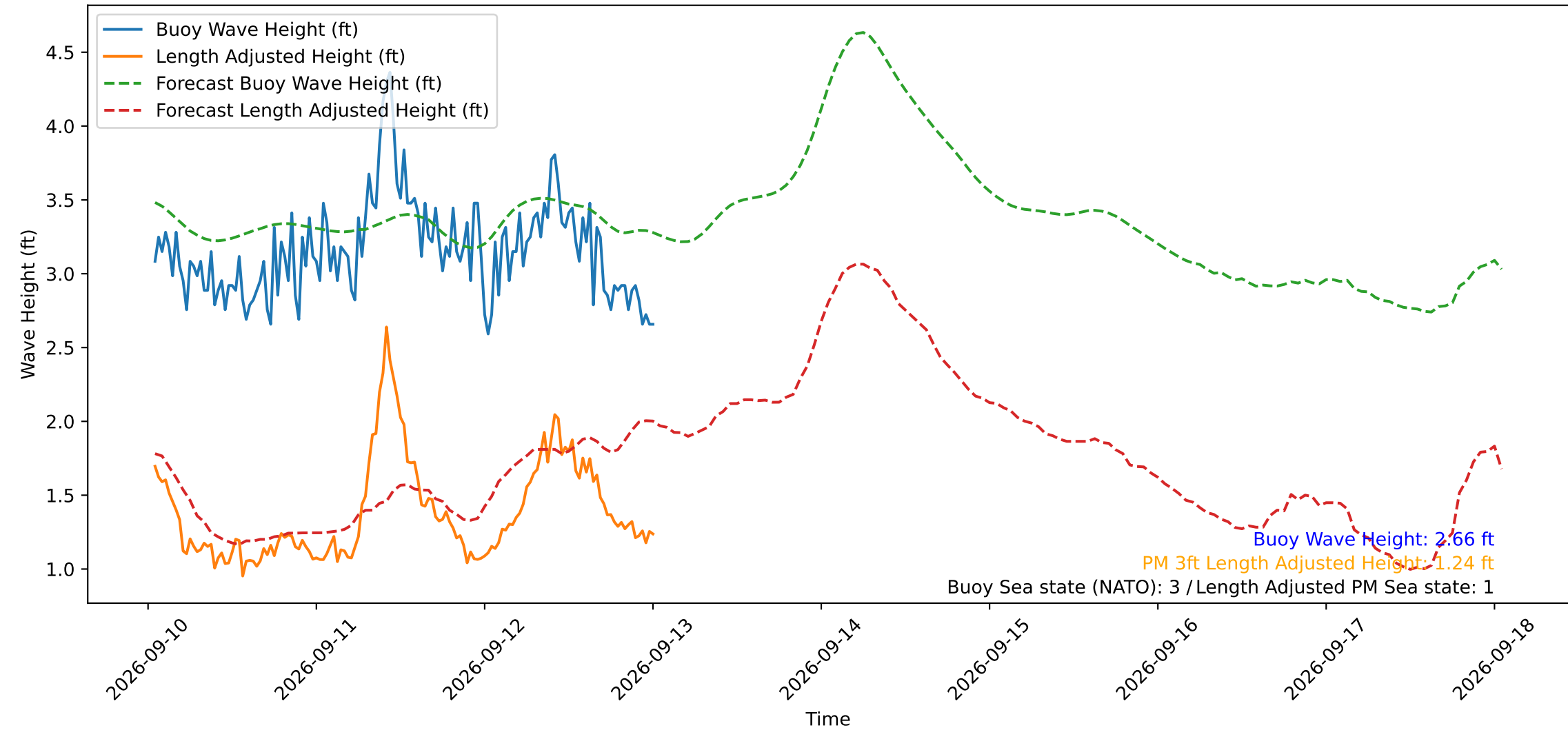
Wave Heights over Time for Oceanside Harbor at 2026-09-13 01:10:30
