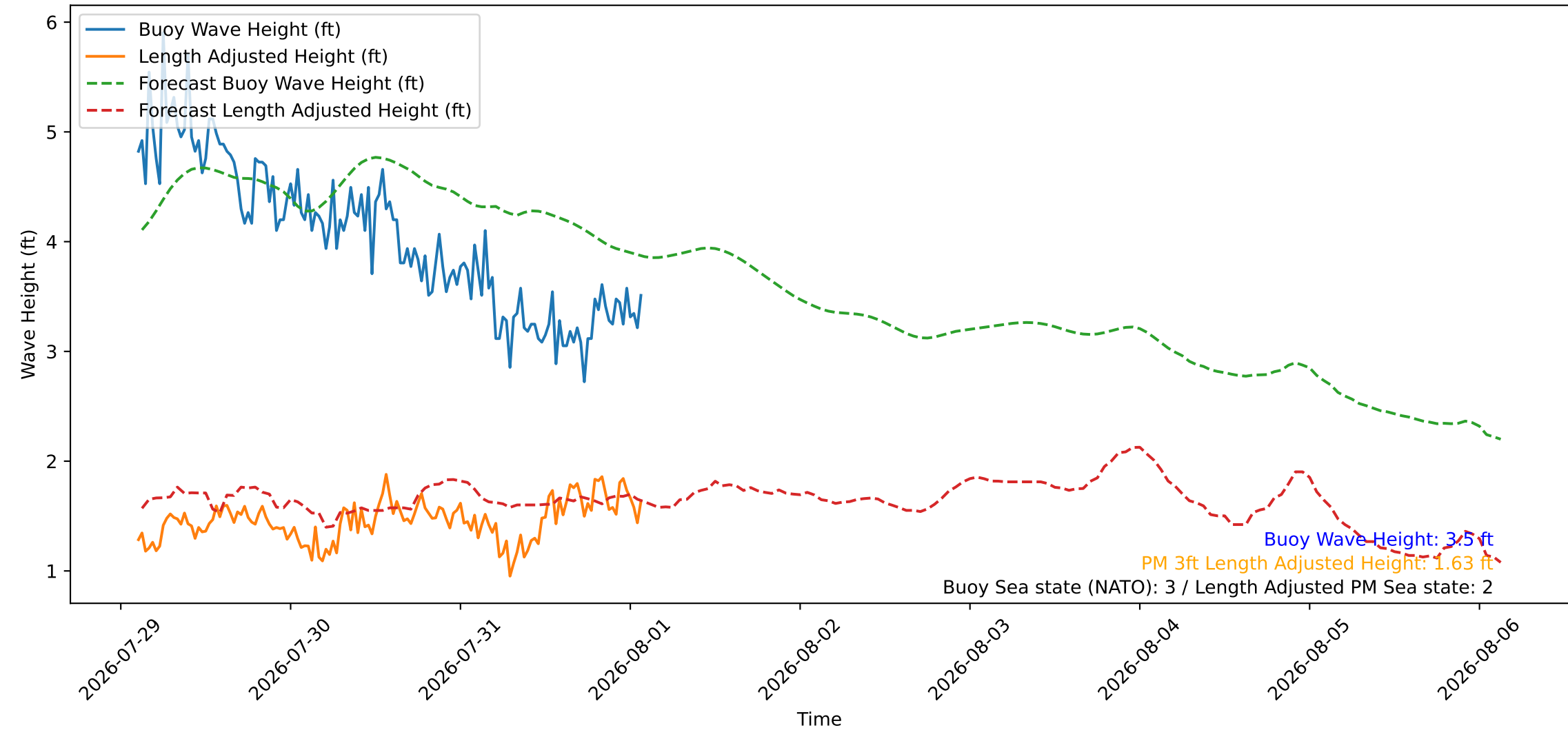
Wave Heights over Time for Oceanside Harbor at 2026-08-01 02:40:27
