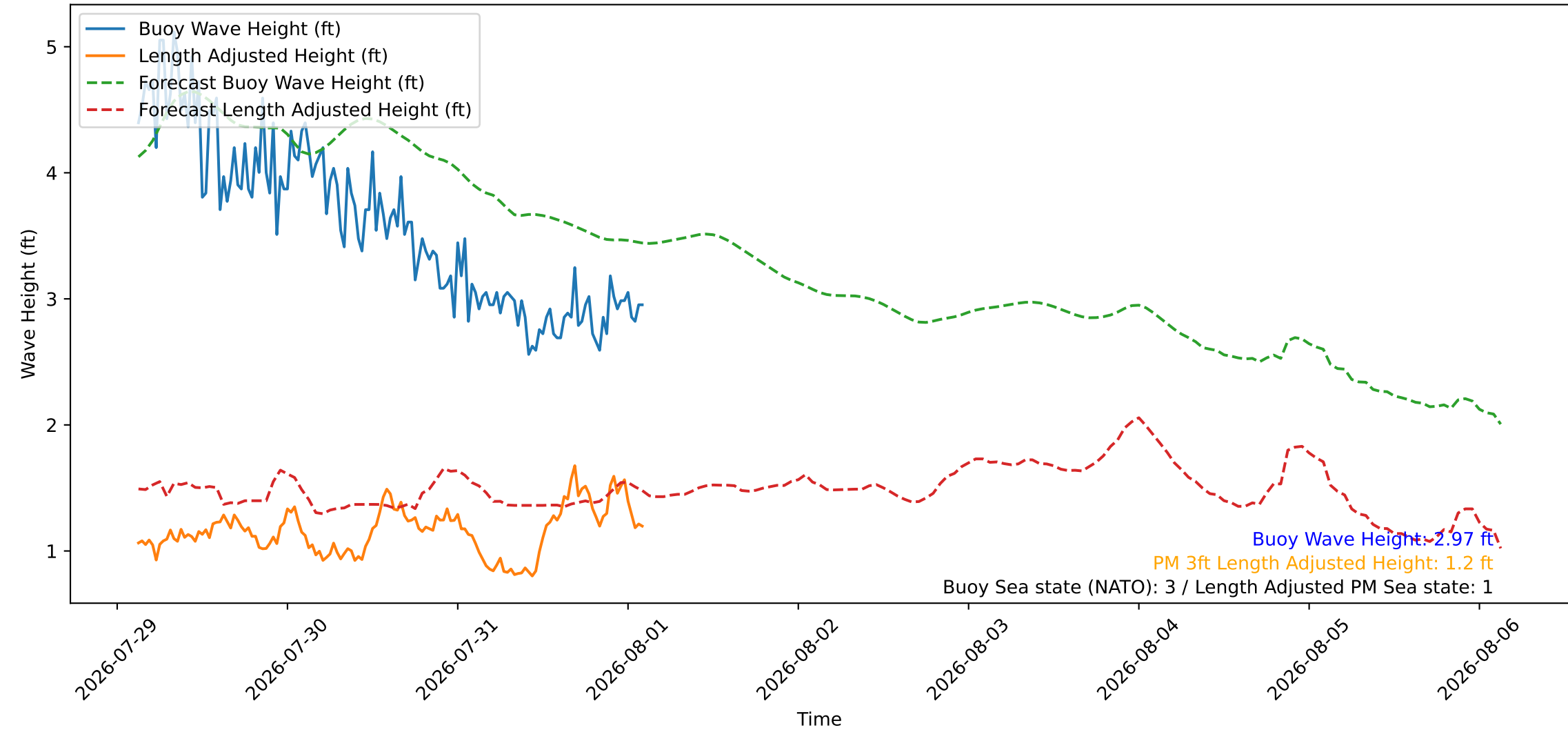
Wave Heights over Time for Red Beach at 2026-08-01 02:40:47
