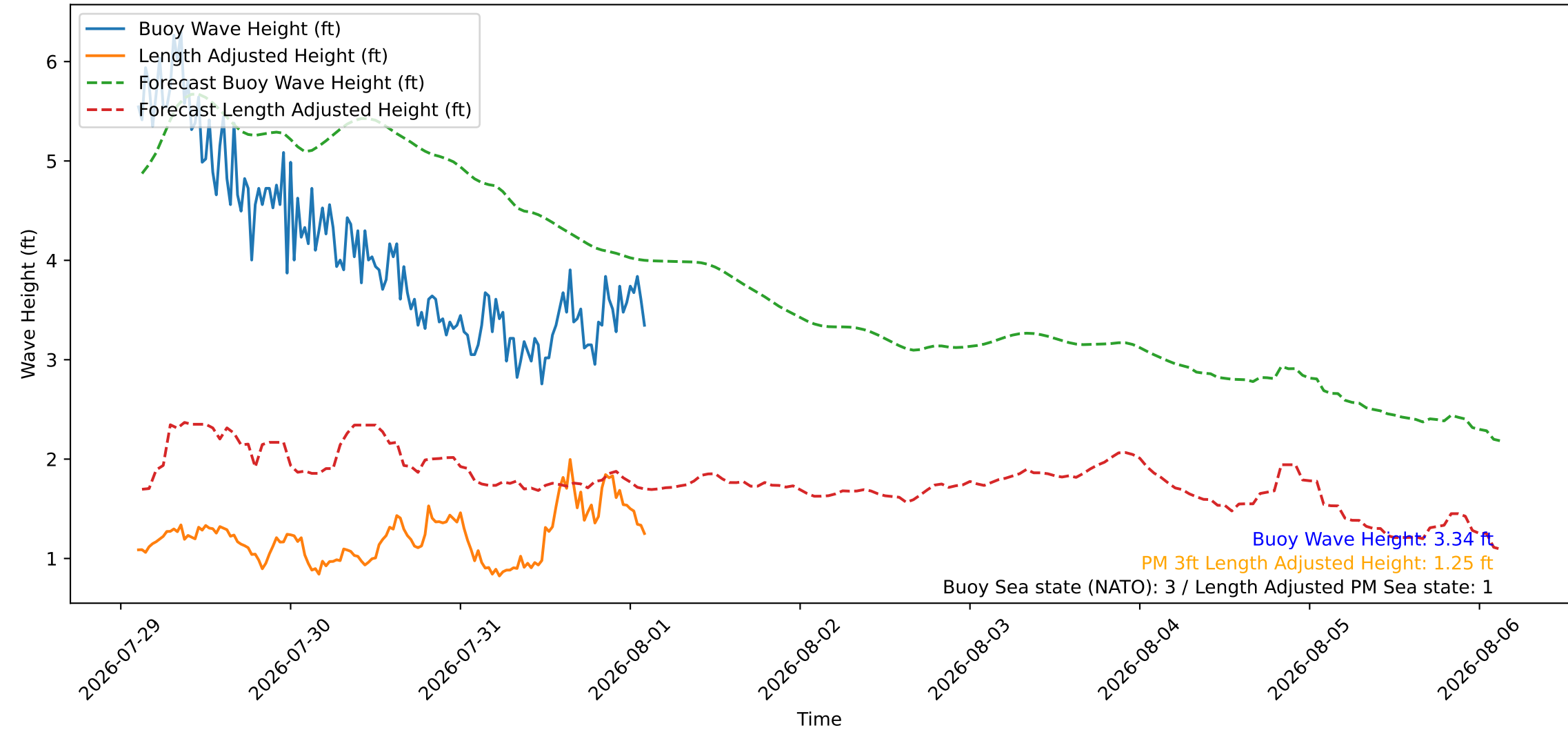
Wave Heights over Time for Green Beach at 2026-08-01 02:41:10
