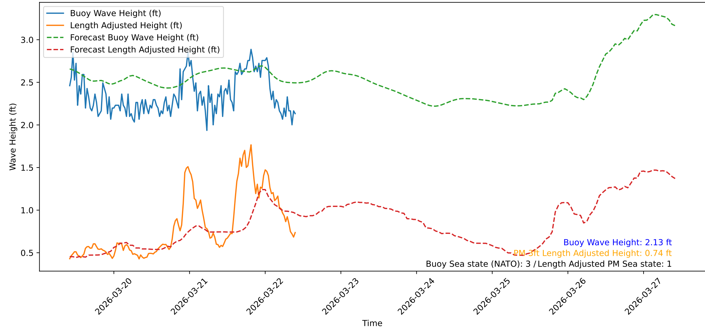
Wave Heights over Time for Green Beach at 2026-03-22 10:11:10
