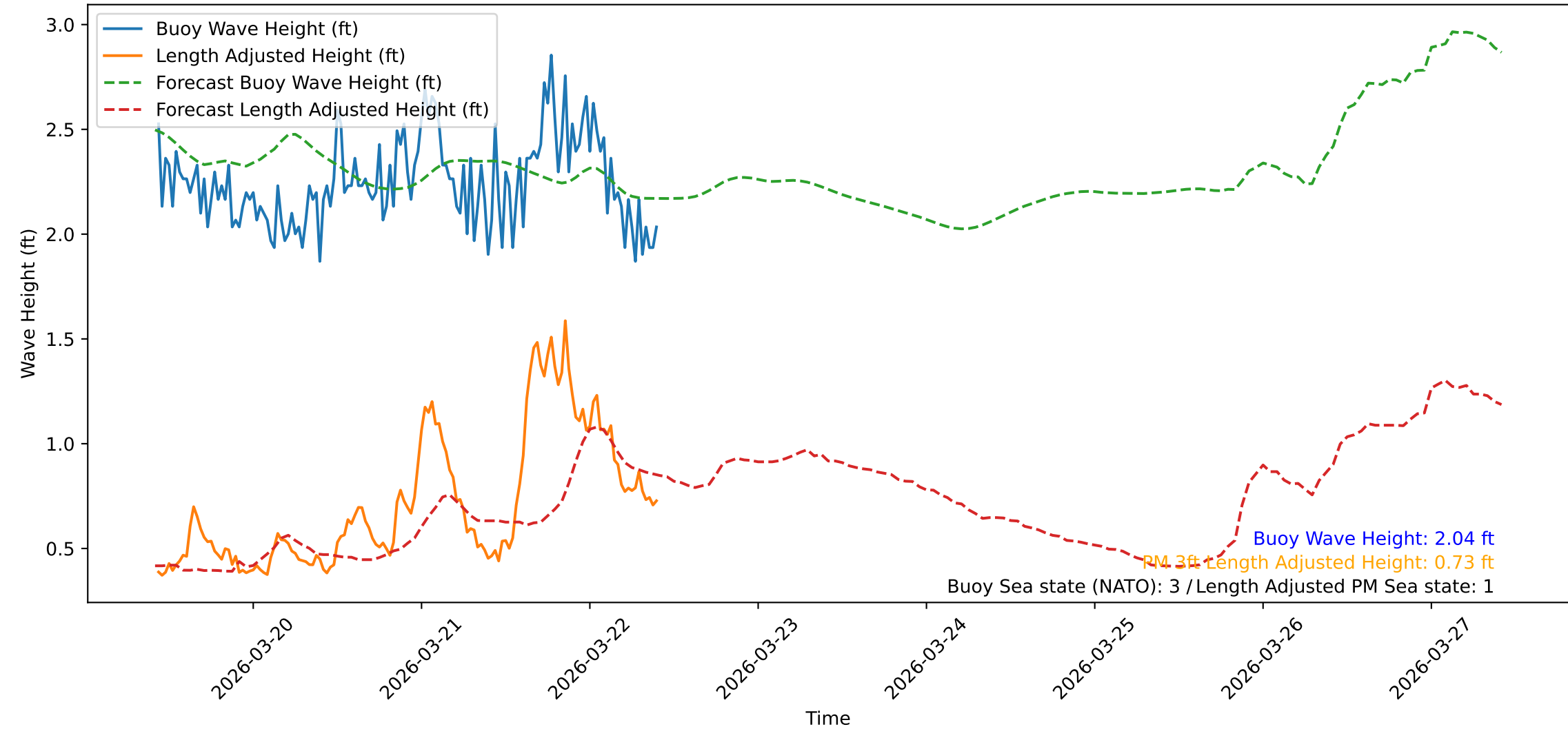
Wave Heights over Time for Red Beach at 2026-03-22 10:10:47
