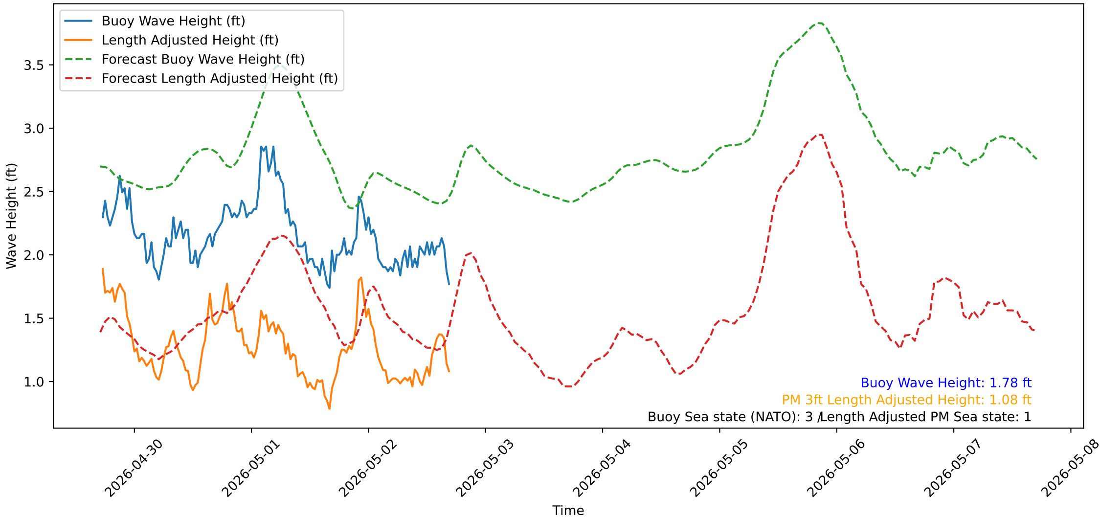
Wave Heights over Time for Green Beach at 2026-05-02 17:21:13
