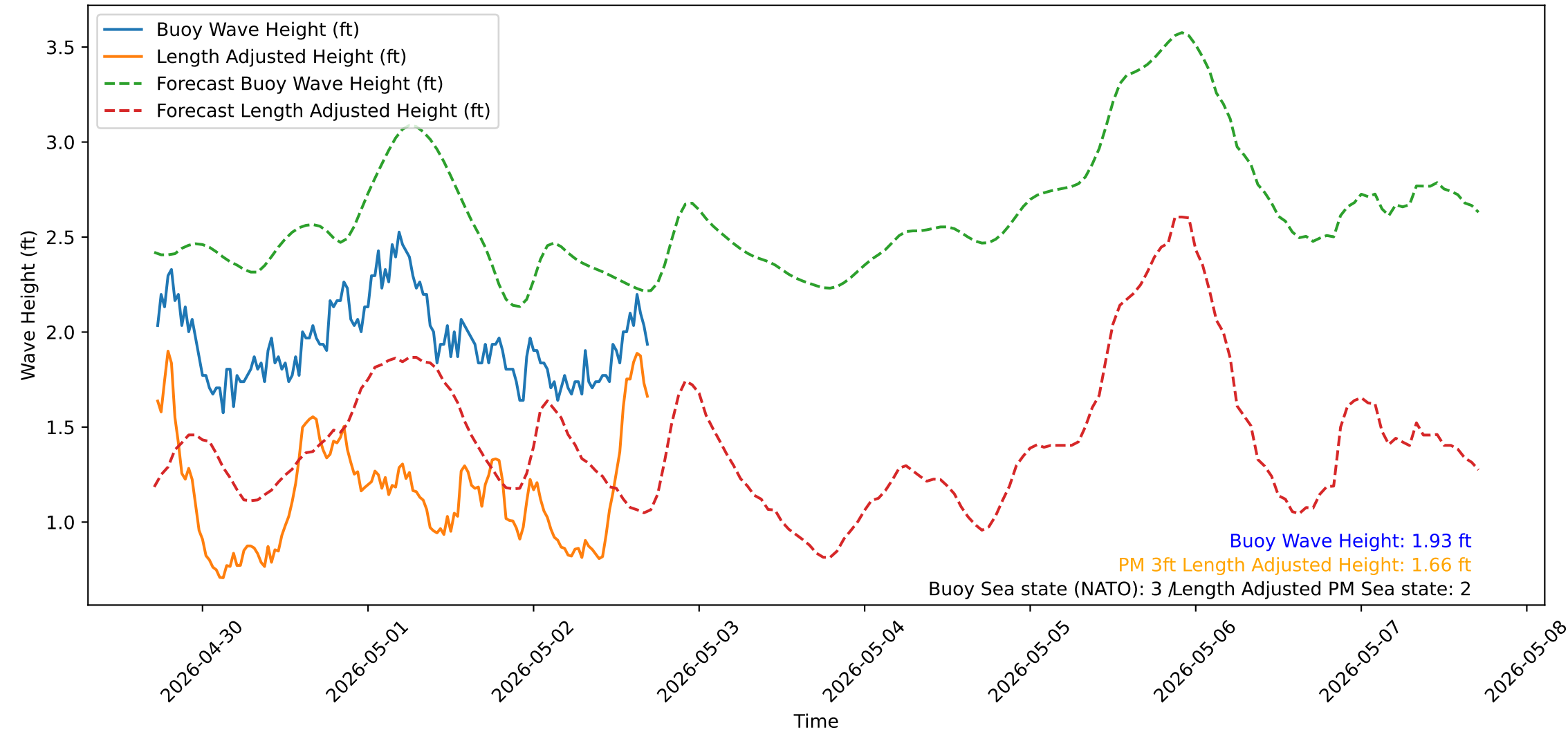
Wave Heights over Time for Red Beach at 2026-05-02 17:20:51
