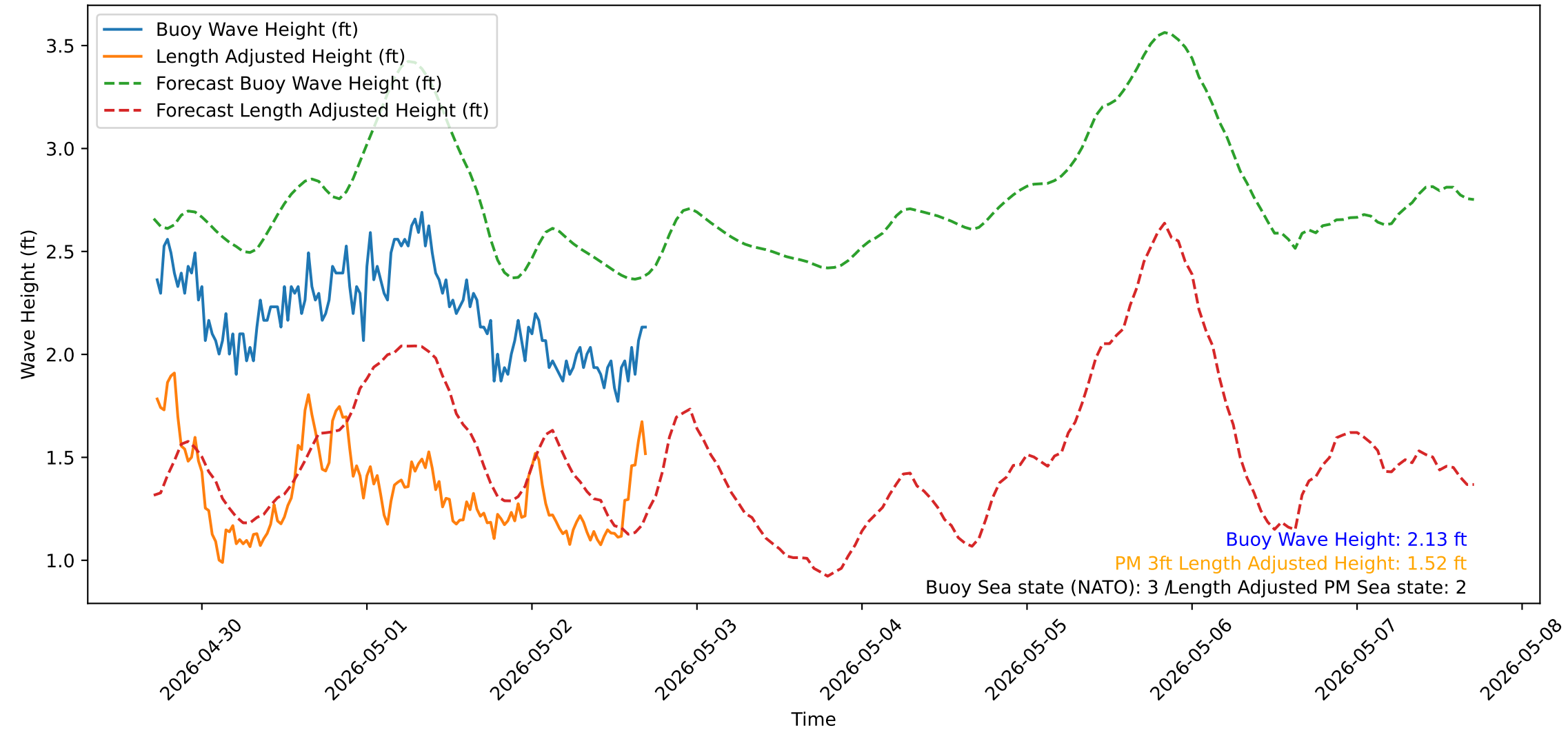
Wave Heights over Time for Oceanside Harbor at 2026-05-02 17:20:31
