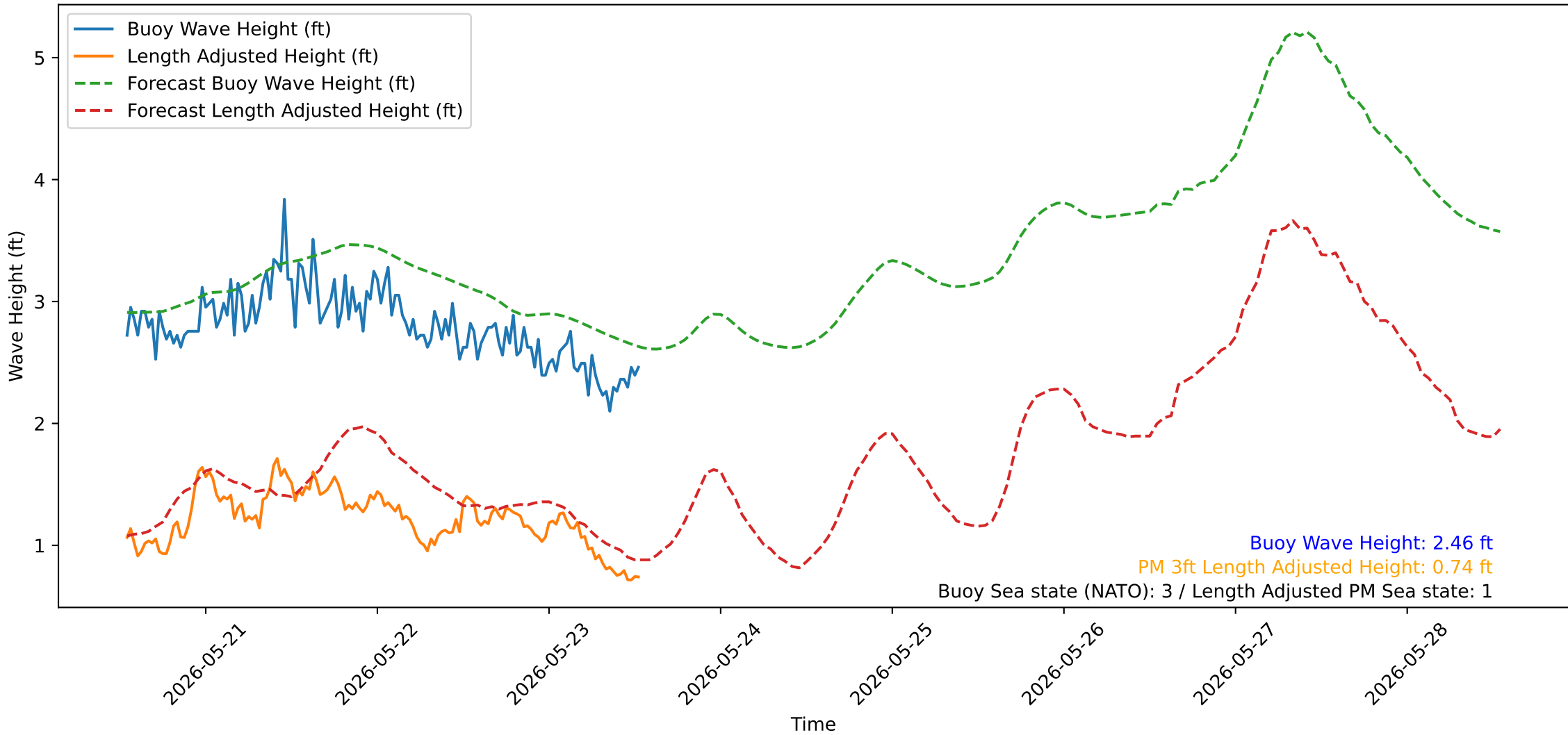
Wave Heights over Time for Oceanside Harbor at 2026-05-23 13:00:32
