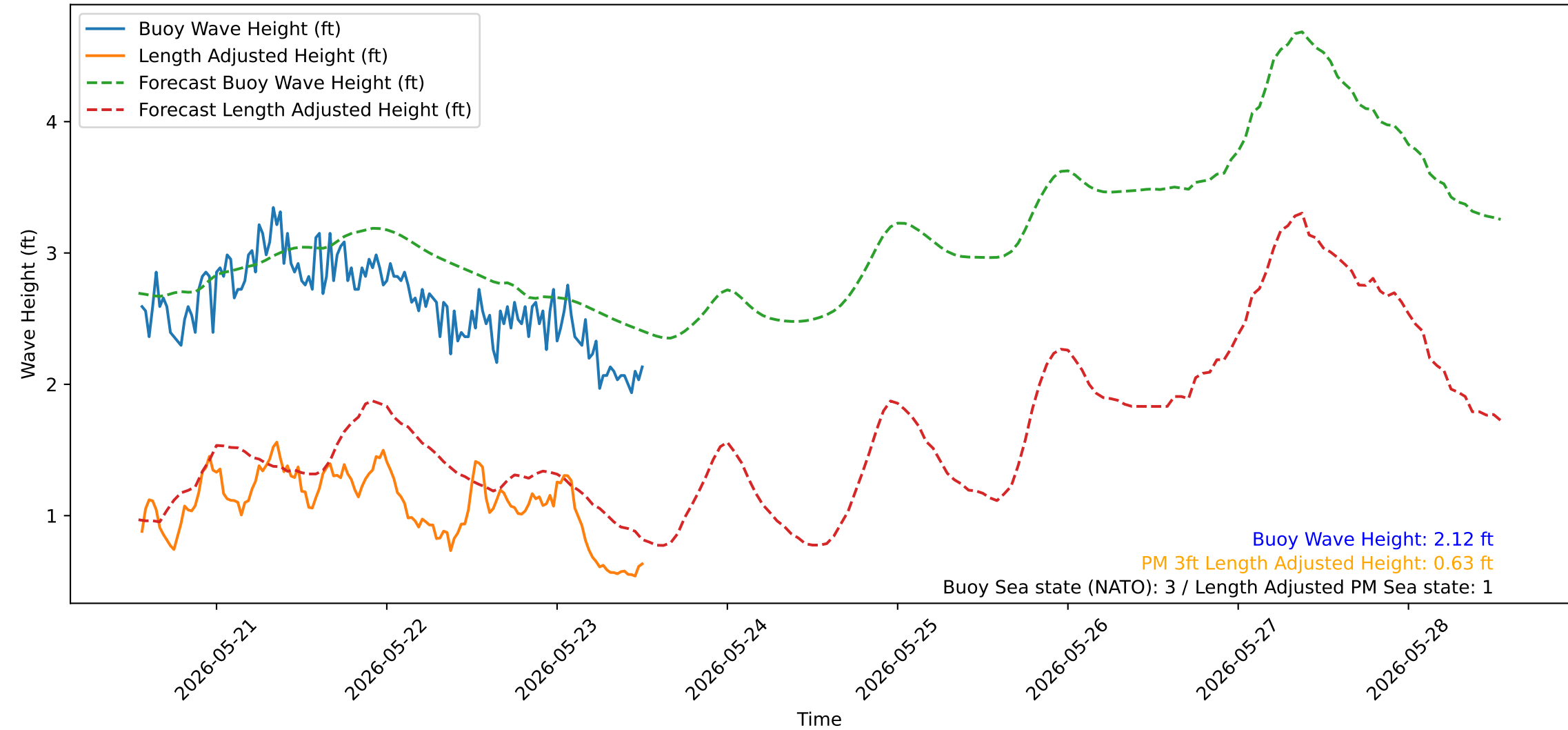
Wave Heights over Time for Red Beach at 2026-05-23 13:00:51
