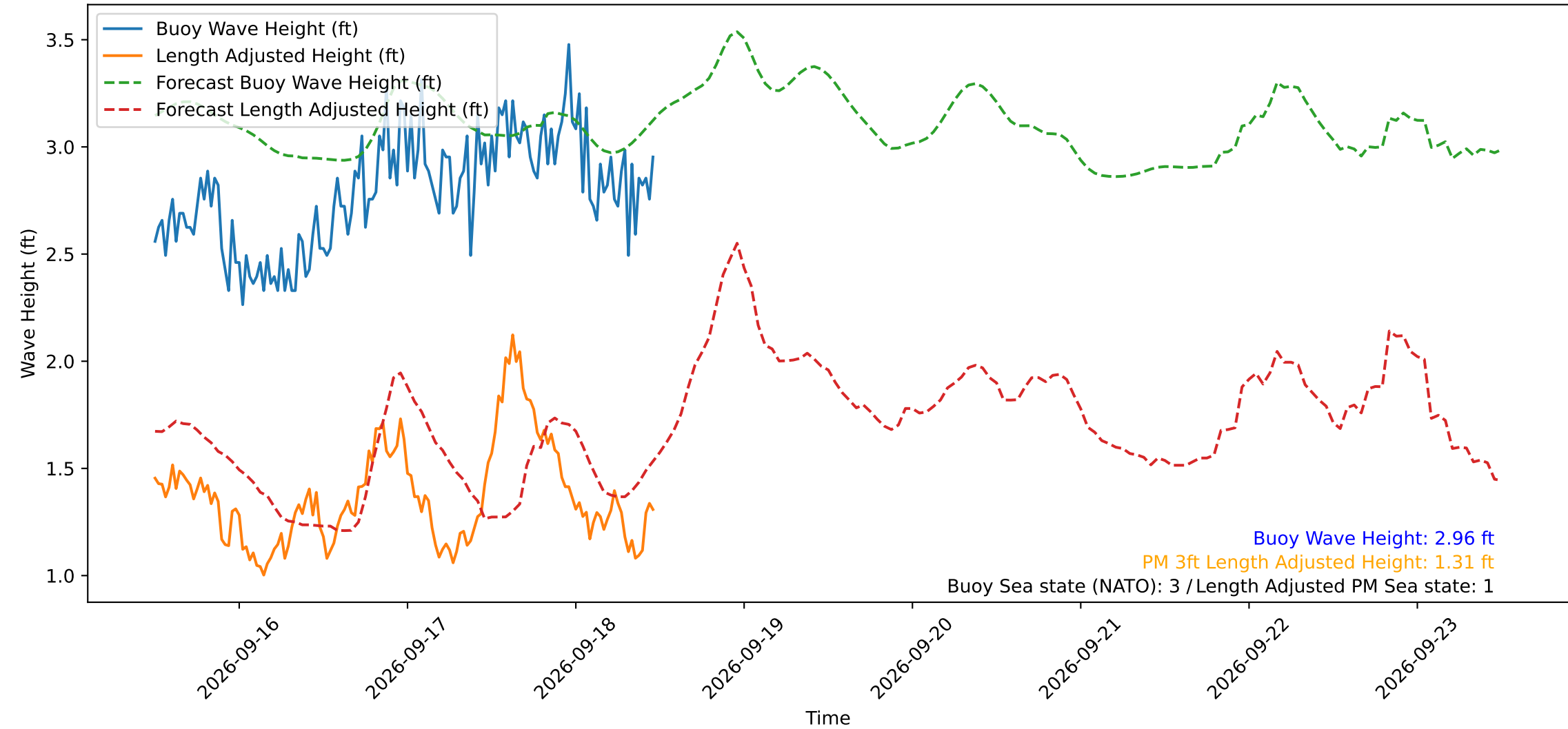
Wave Heights over Time for Green Beach at 2026-09-18 11:51:19
