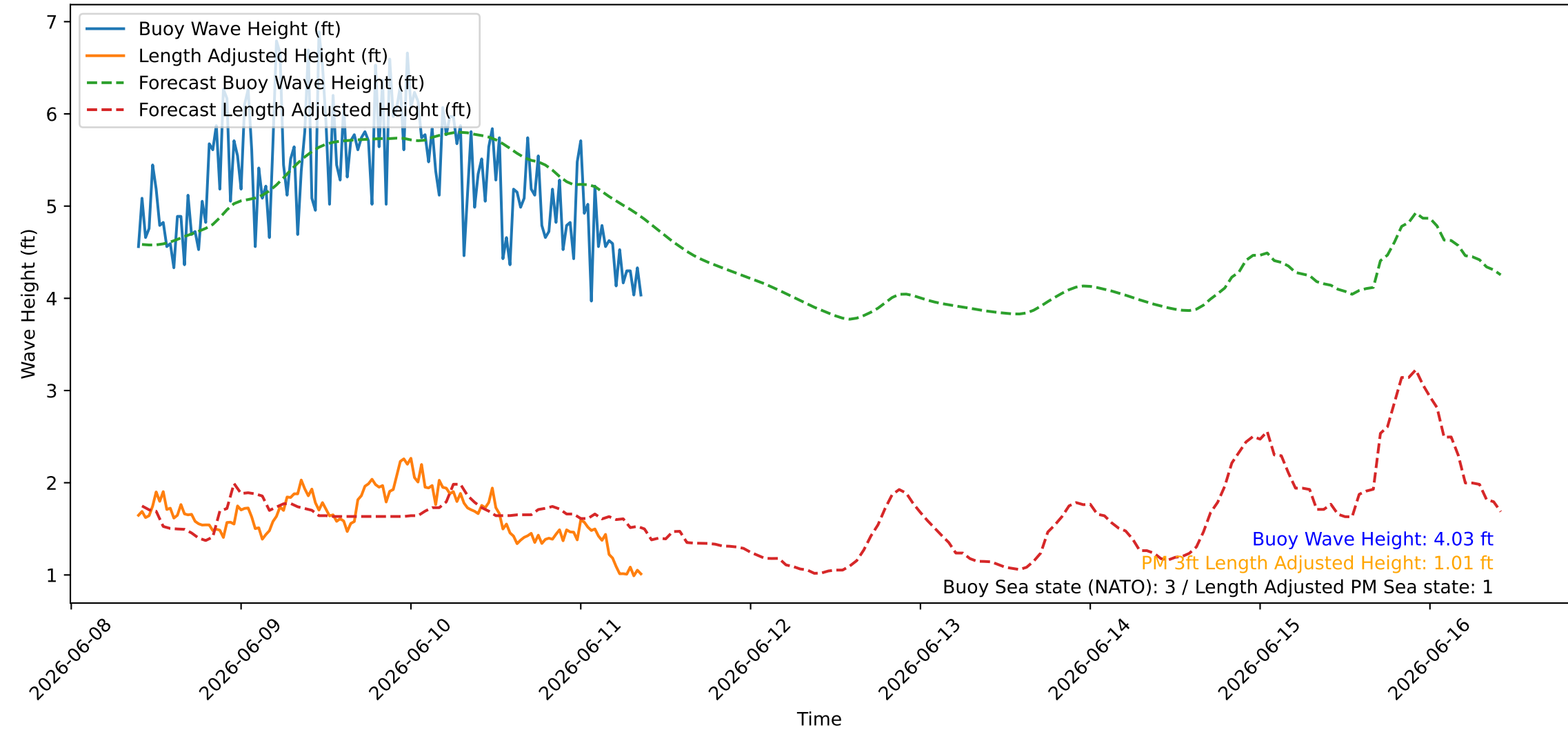
Wave Heights over Time for Green Beach at 2026-06-11 09:31:09
