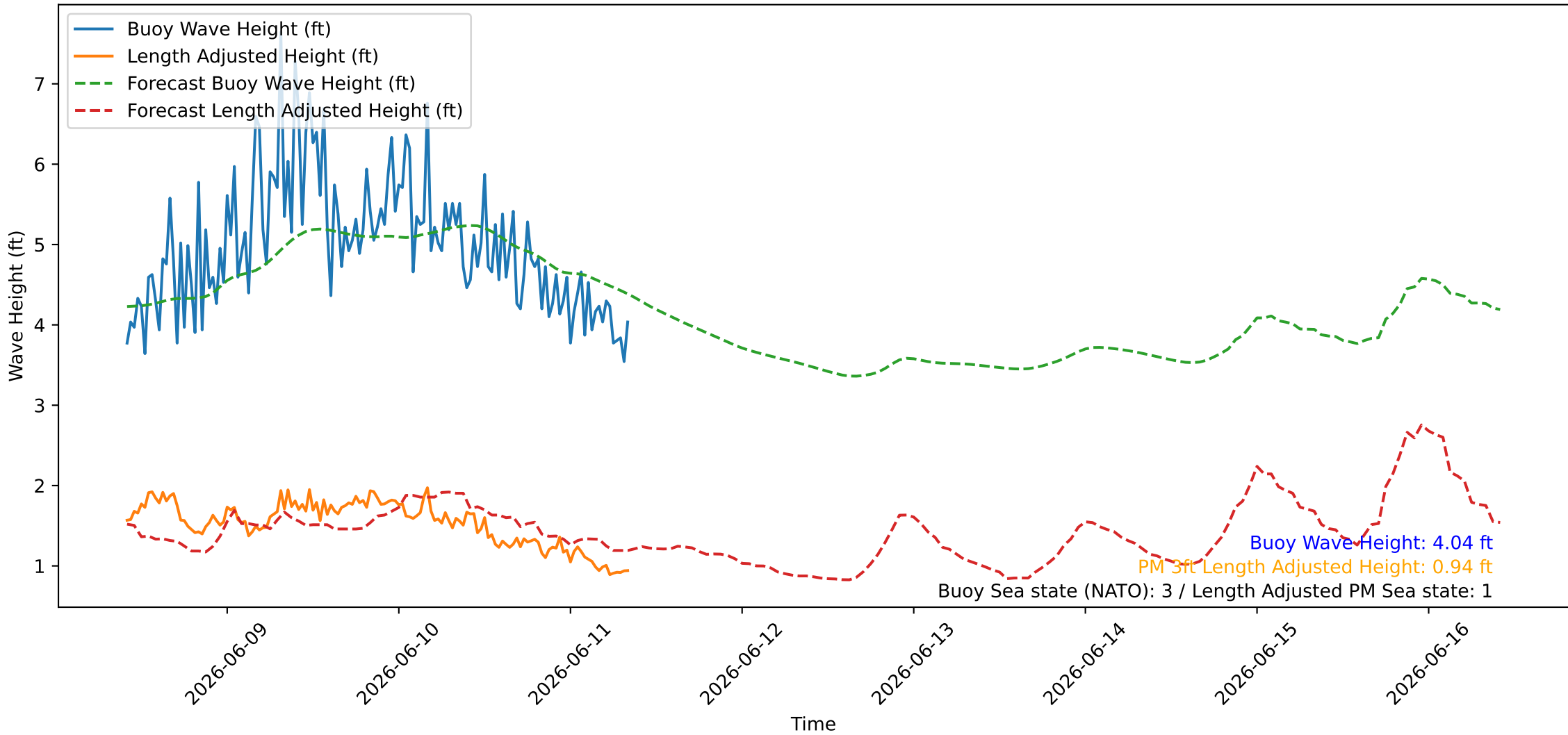
Wave Heights over Time for Red Beach at 2026-06-11 09:30:46
