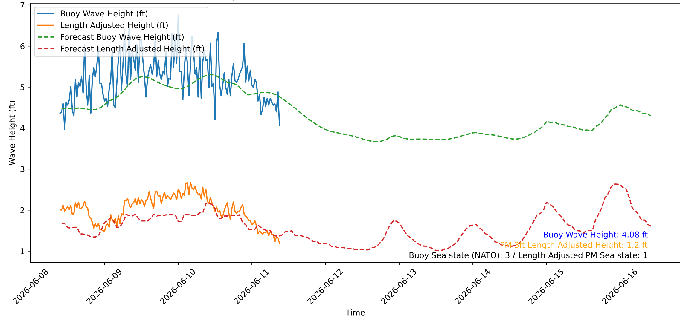
Wave Heights over Time for Oceanside Harbor at 2026-06-11 09:30:26
