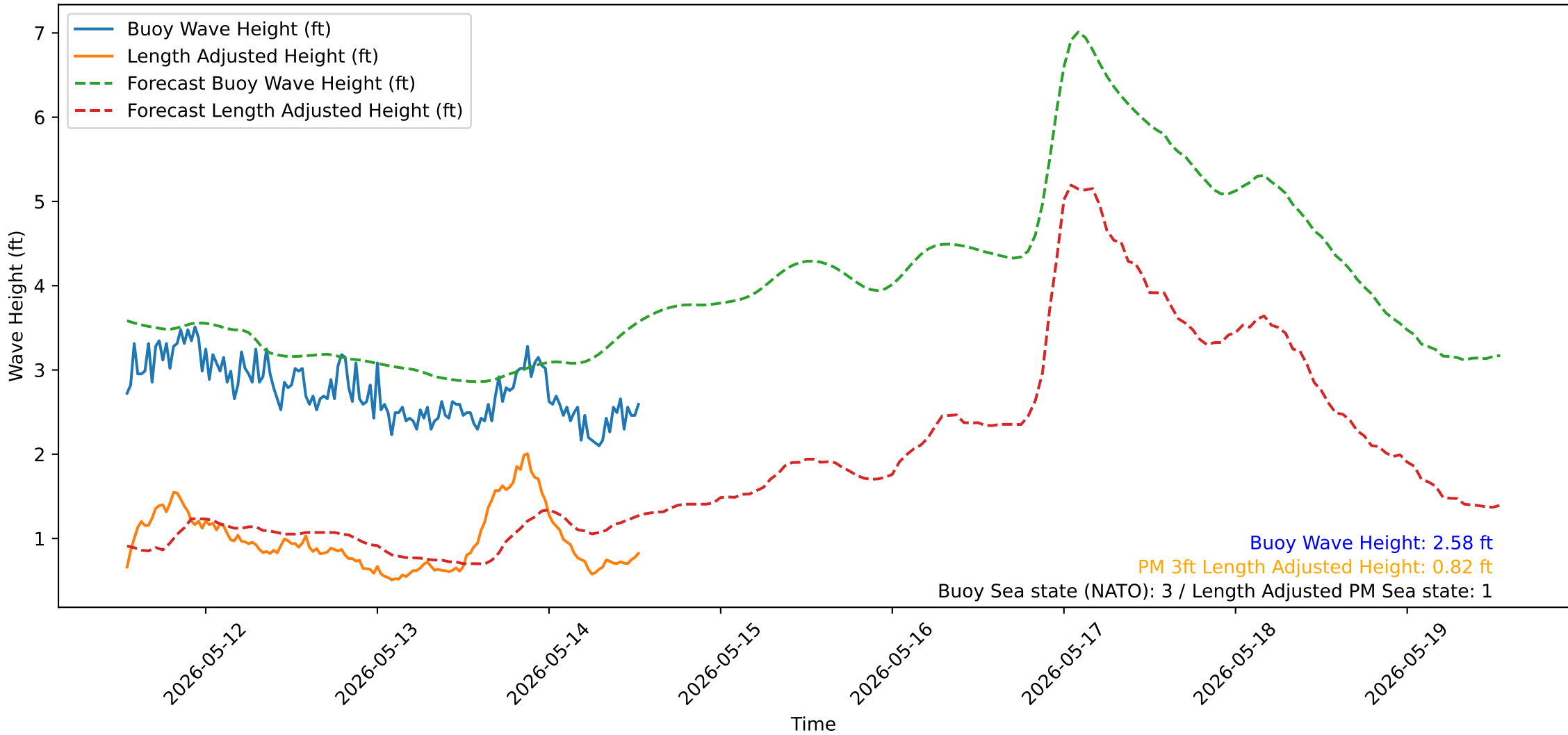
Wave Heights over Time for Green Beach at 2026-05-14 13:11:13
