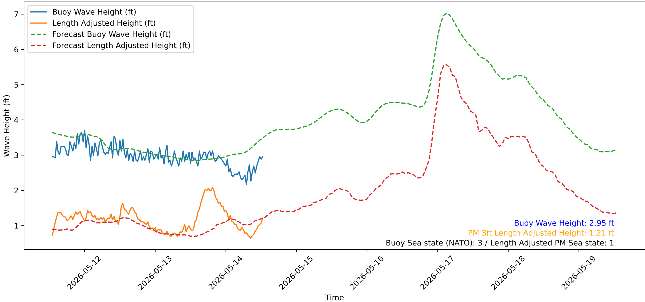
Wave Heights over Time for Oceanside Harbor at 2026-05-14 13:10:31
