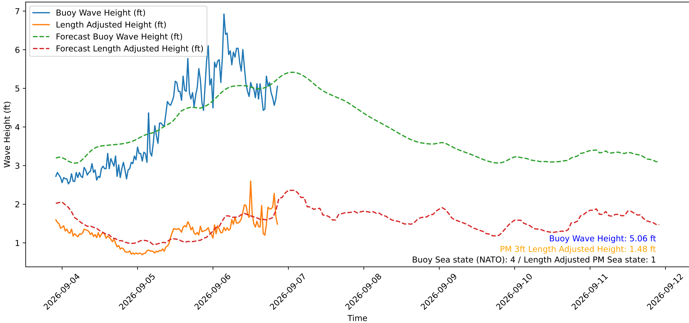
Wave Heights over Time for Red Beach at 2026-09-06 21:30:50
