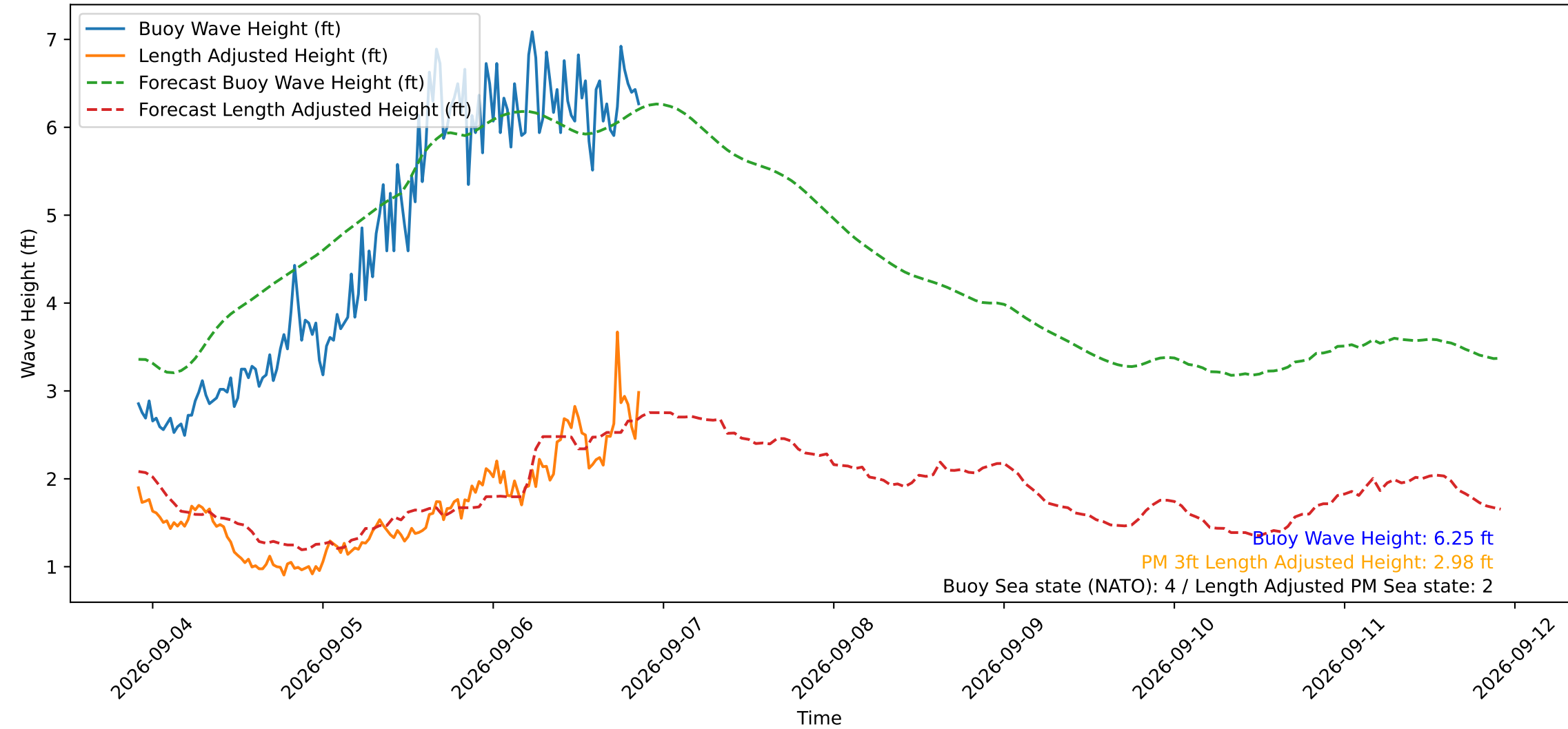
Wave Heights over Time for Green Beach at 2026-09-06 21:31:12
