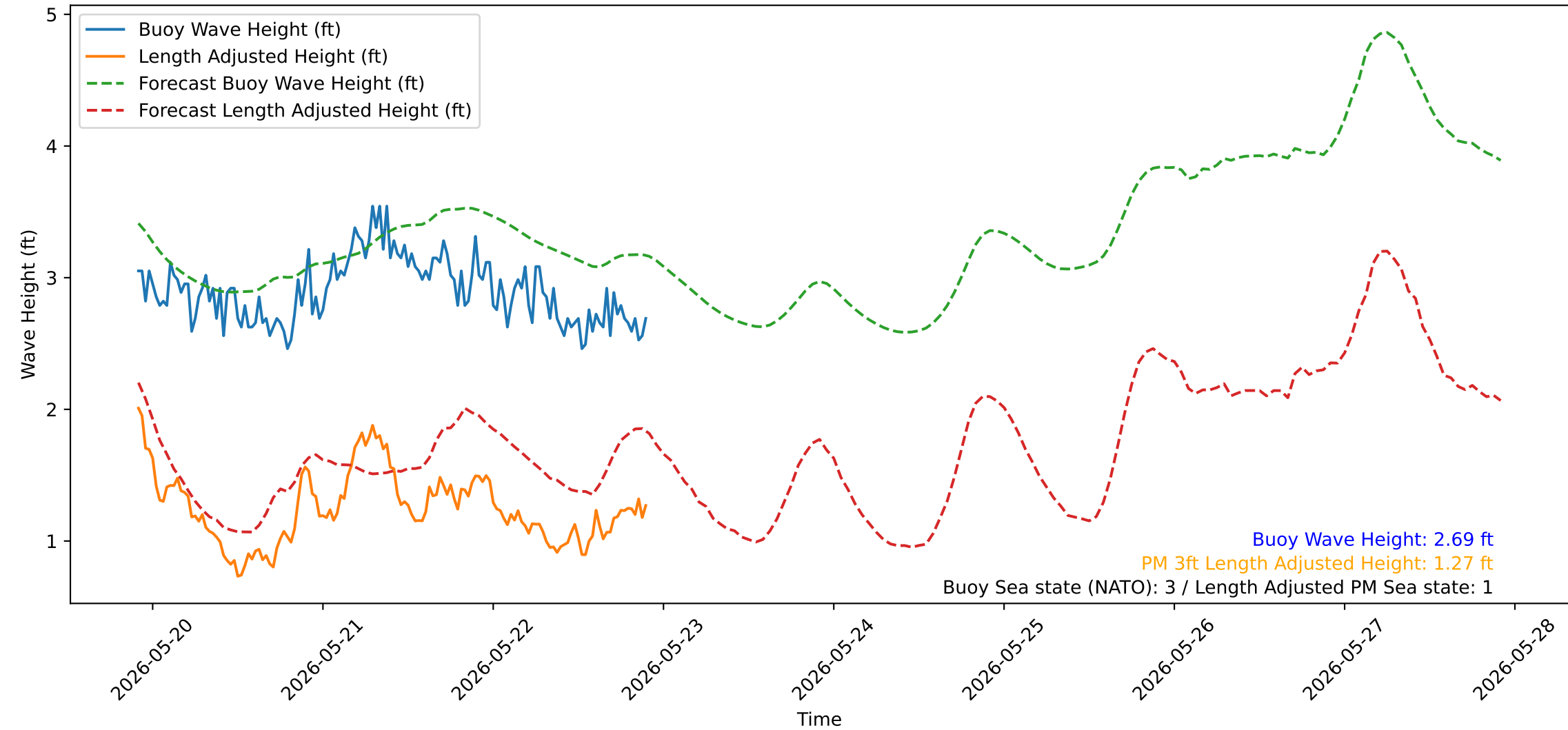
Wave Heights over Time for Green Beach at 2026-05-22 22:11:13
