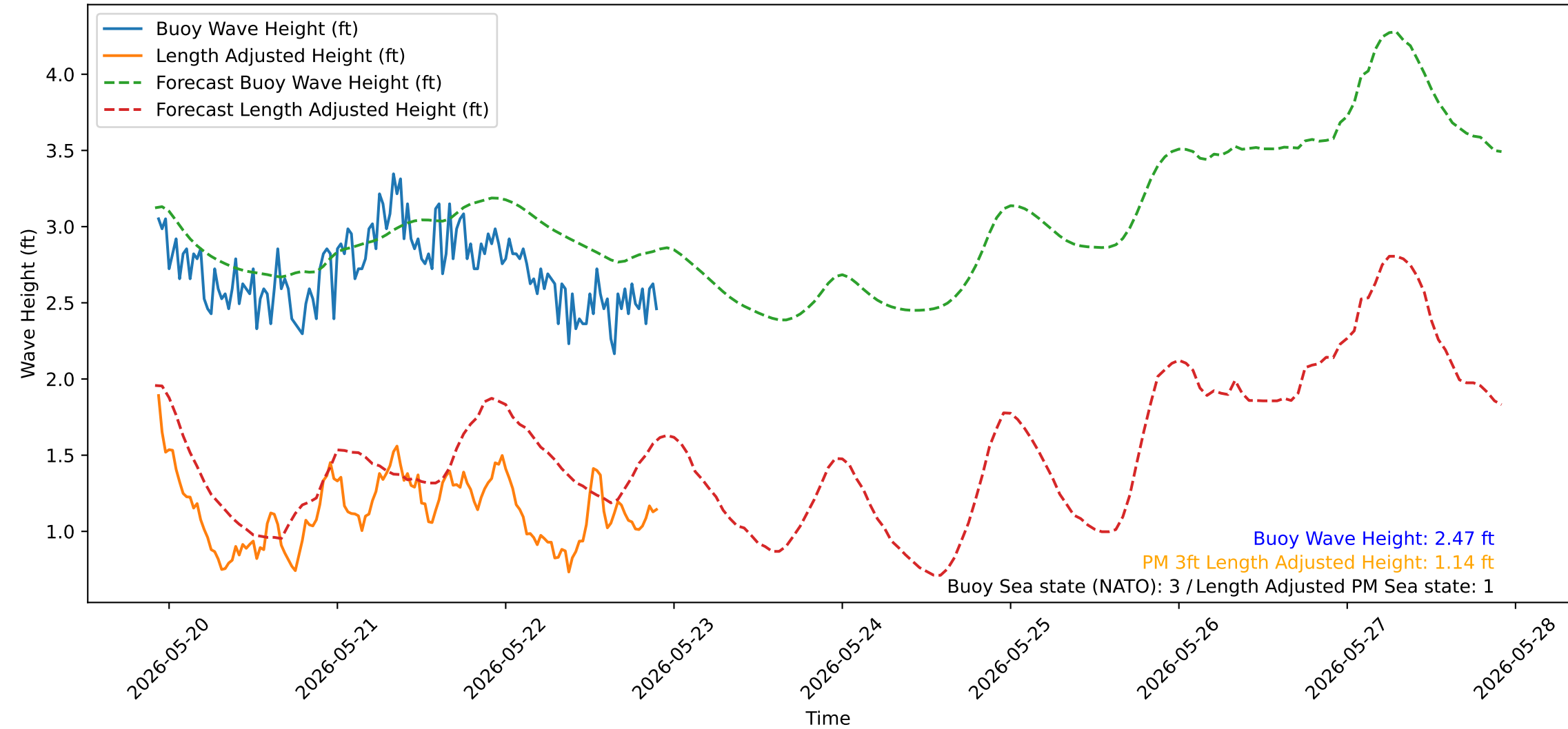
Wave Heights over Time for Red Beach at 2026-05-22 22:10:50
