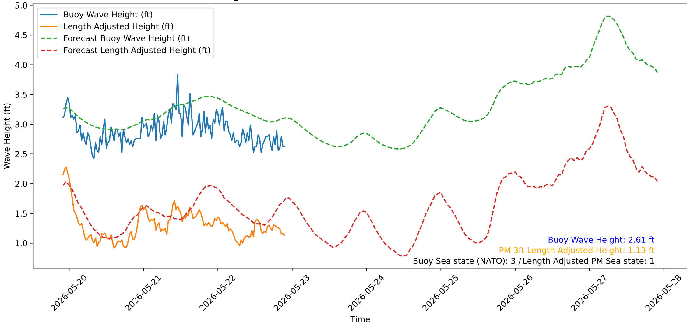
Wave Heights over Time for Oceanside Harbor at 2026-05-22 22:10:31
