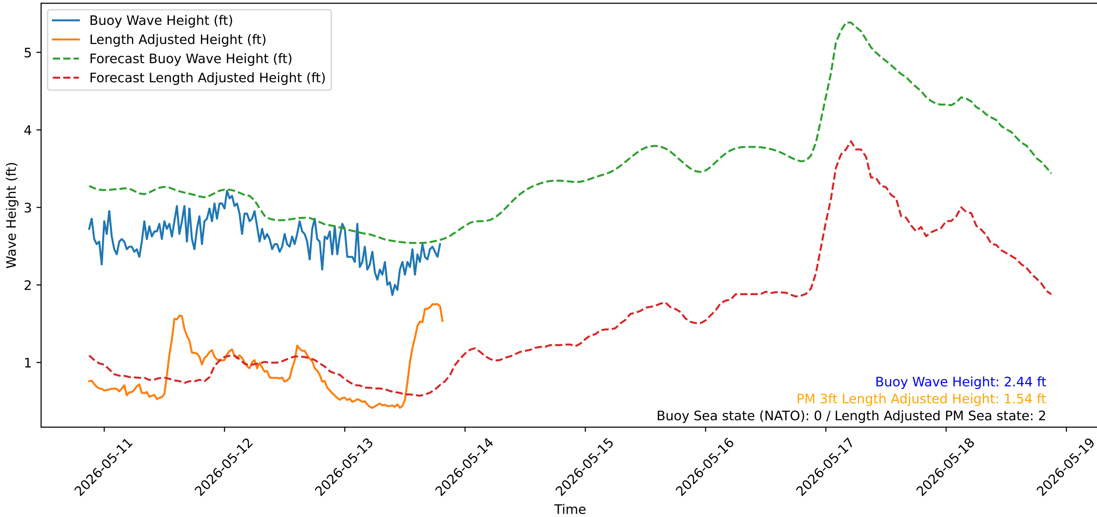
Wave Heights over Time for Red Beach at 2026-05-13 20:30:50
