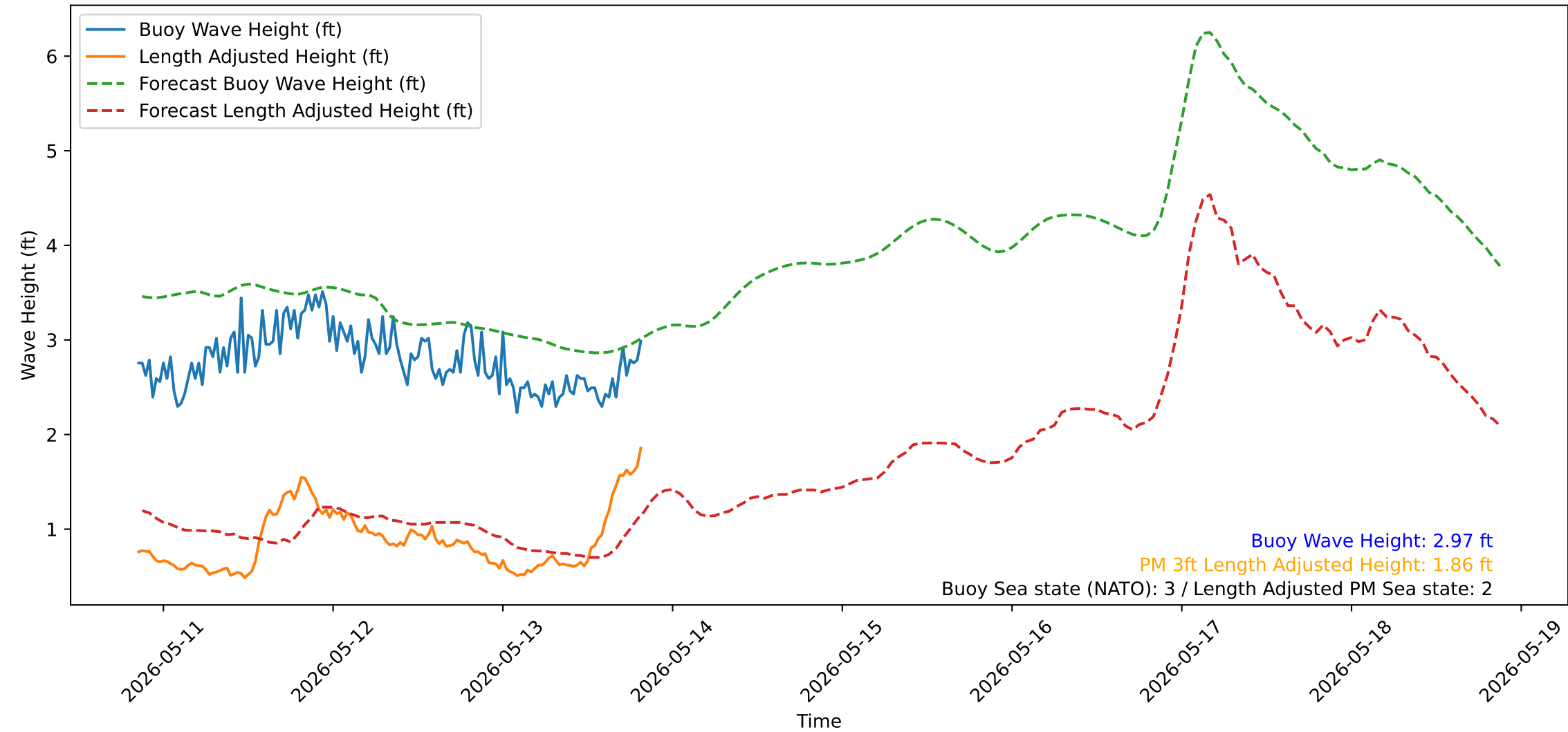
Wave Heights over Time for Green Beach at 2026-05-13 20:31:13
