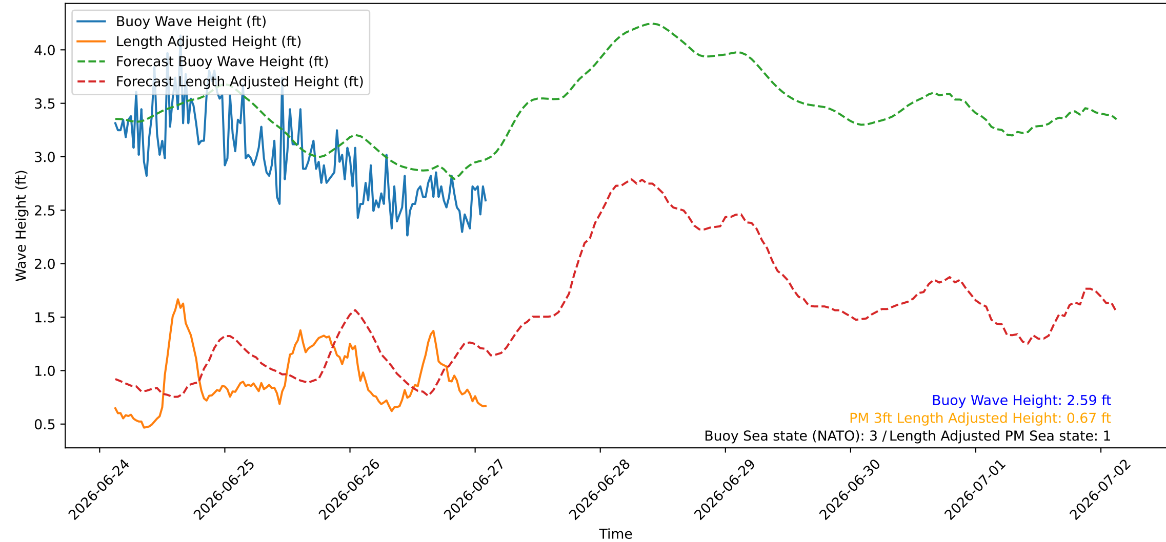
Wave Heights over Time for Red Beach at 2026-06-27 02:50:47
