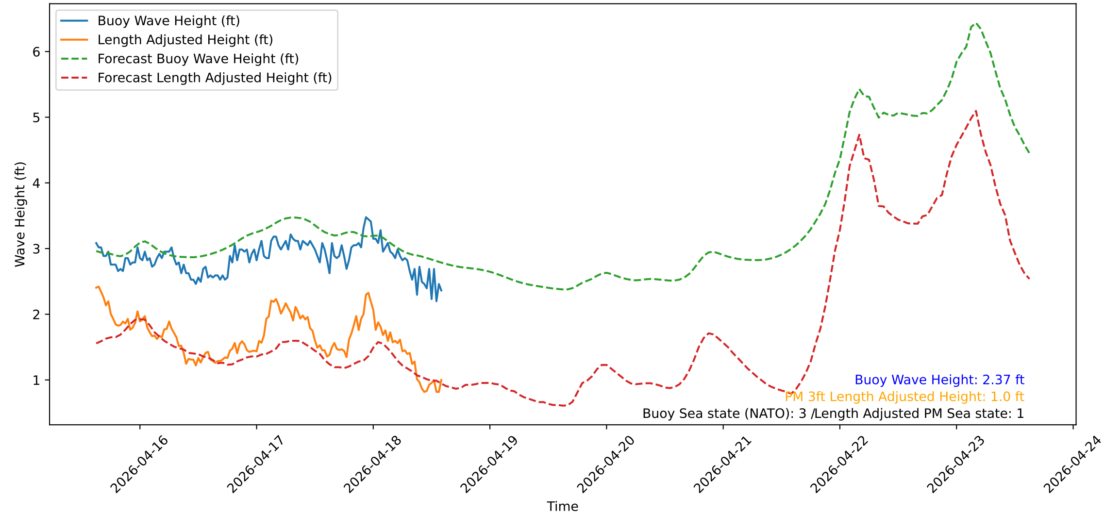
Wave Heights over Time for Green Beach at 2026-04-18 15:01:12
