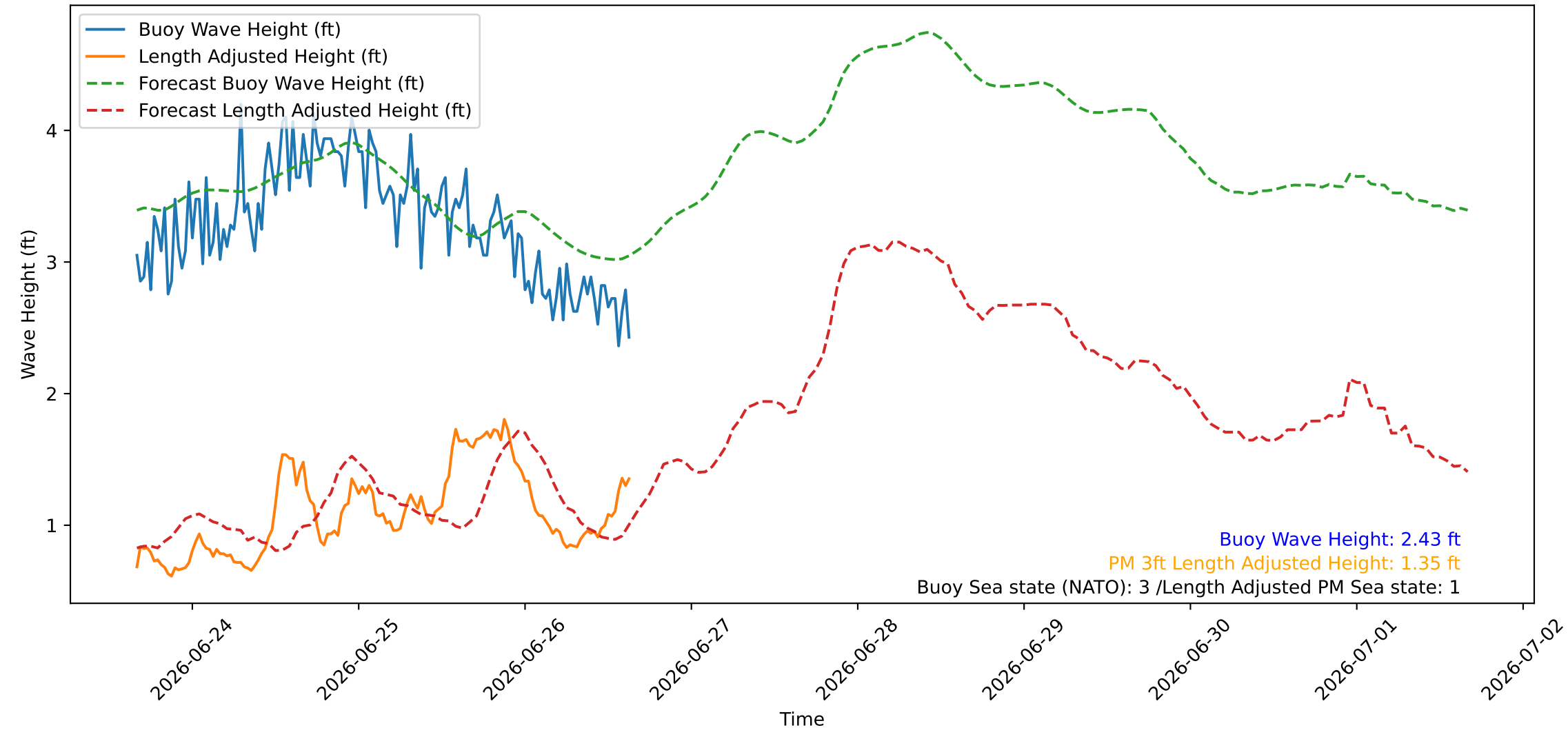
Wave Heights over Time for Green Beach at 2026-06-26 16:01:08
