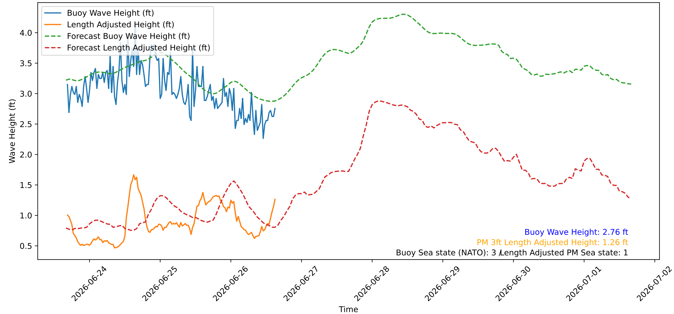
Wave Heights over Time for Red Beach at 2026-06-26 16:00:45
