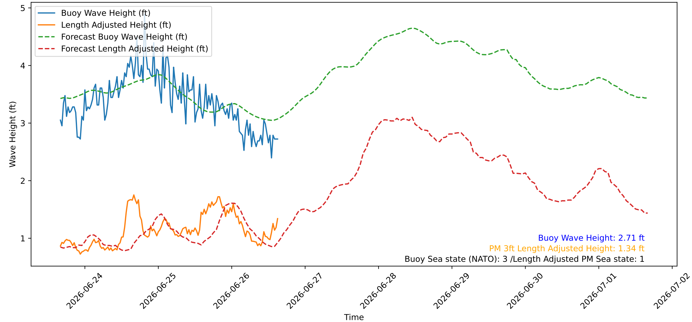
Wave Heights over Time for Oceanside Harbor at 2026-06-26 16:00:26
