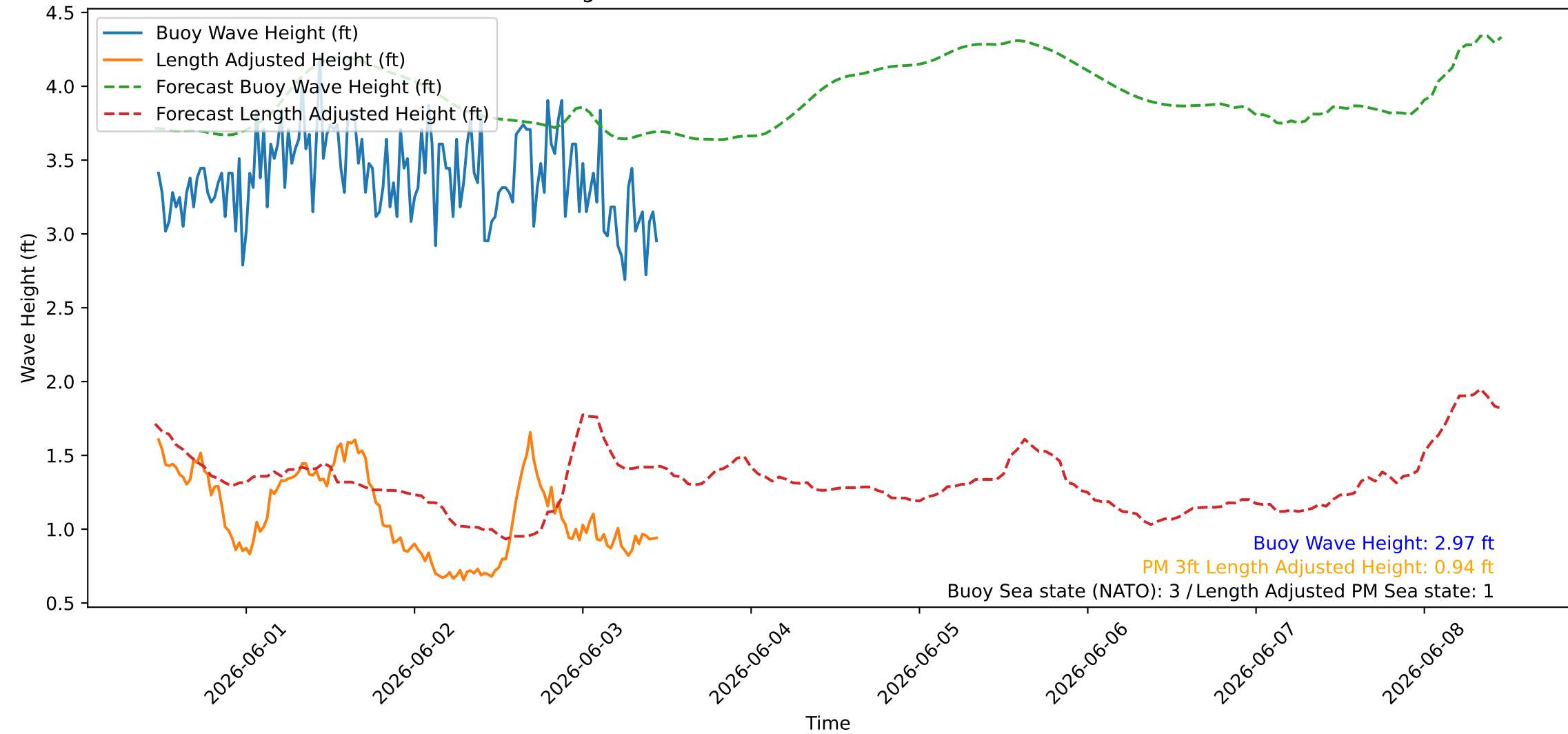
Wave Heights over Time for Red Beach at 2026-06-03 11:20:46
