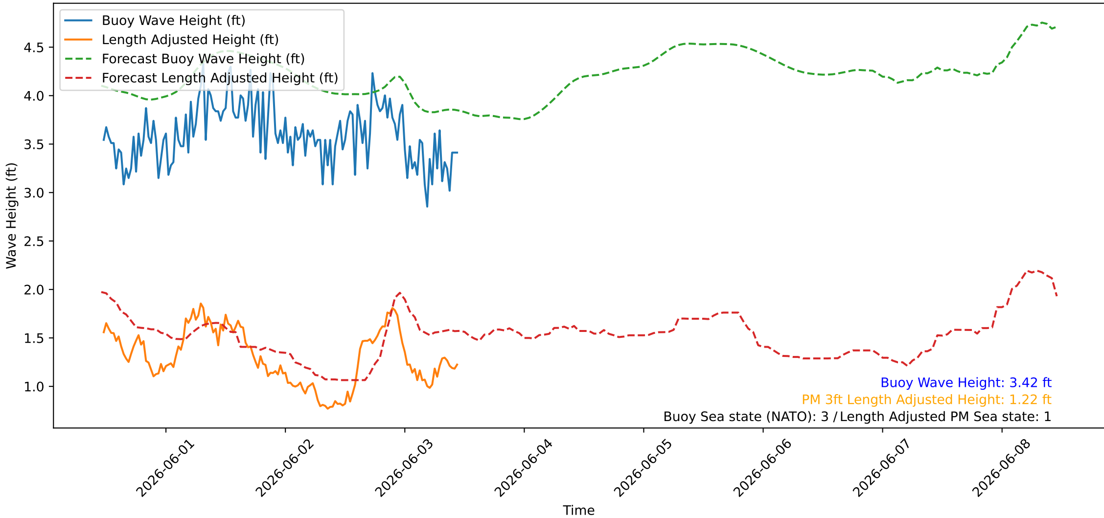
Wave Heights over Time for Green Beach at 2026-06-03 11:21:09
