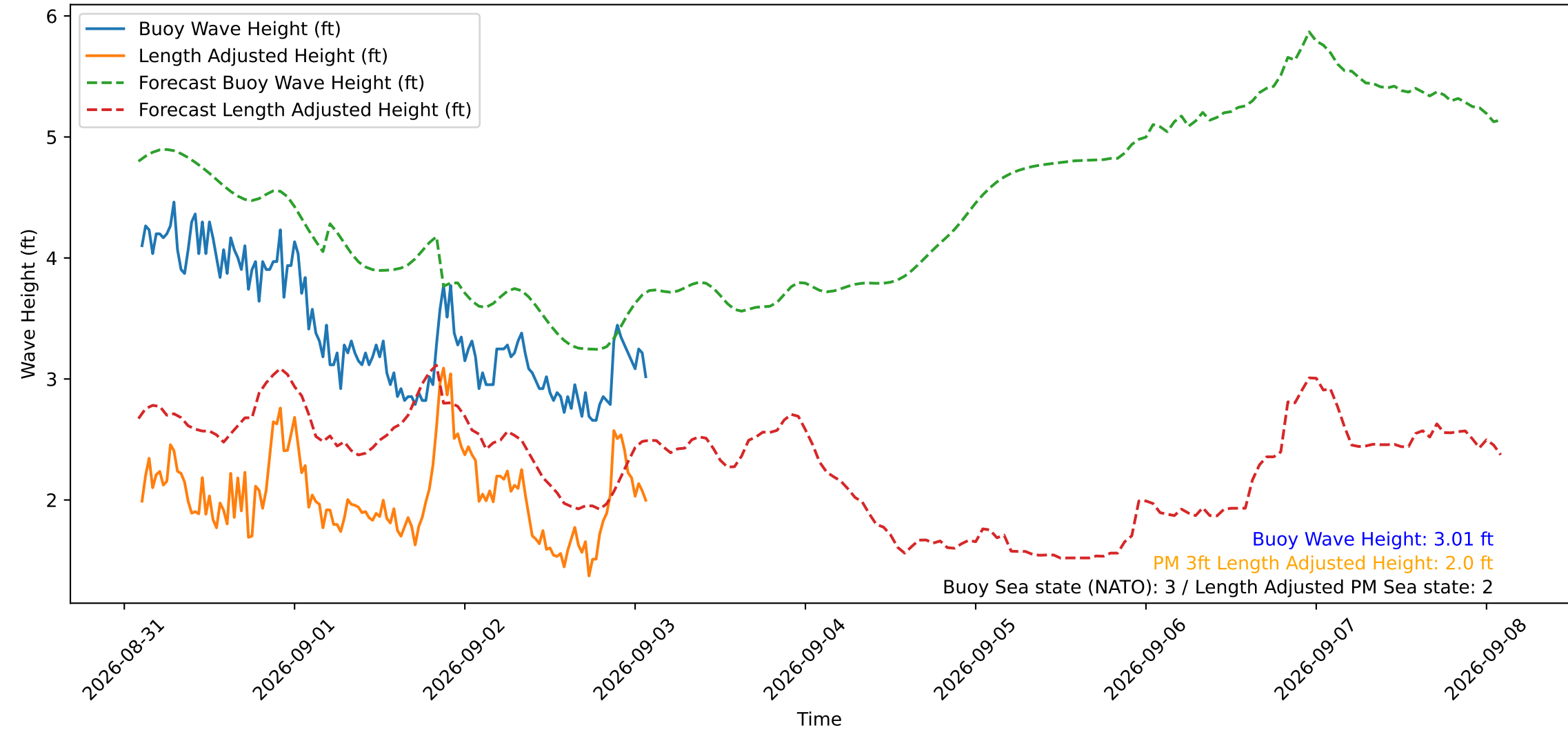
Wave Heights over Time for Green Beach at 2026-09-03 02:21:15
