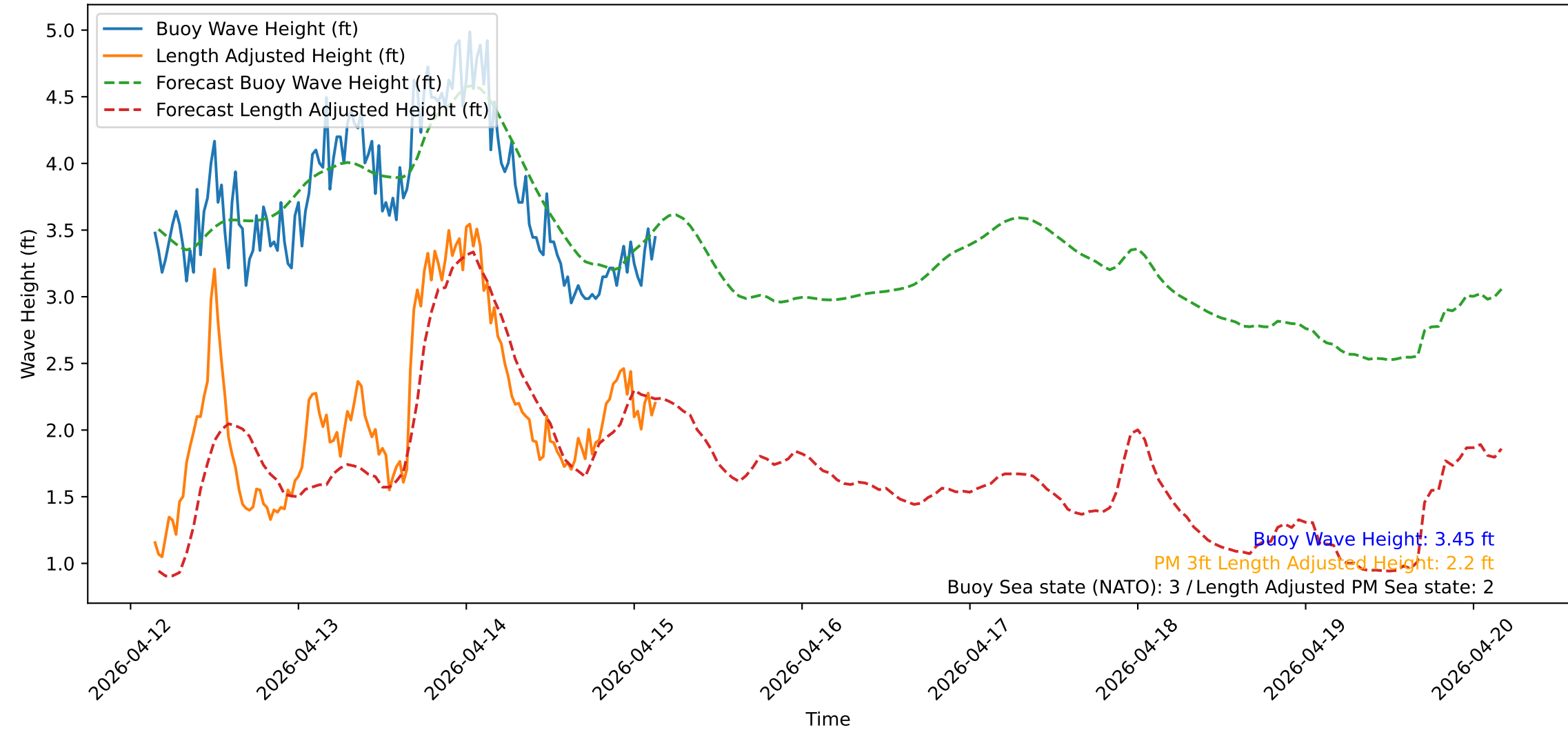
Wave Heights over Time for Green Beach at 2026-04-15 03:41:11
