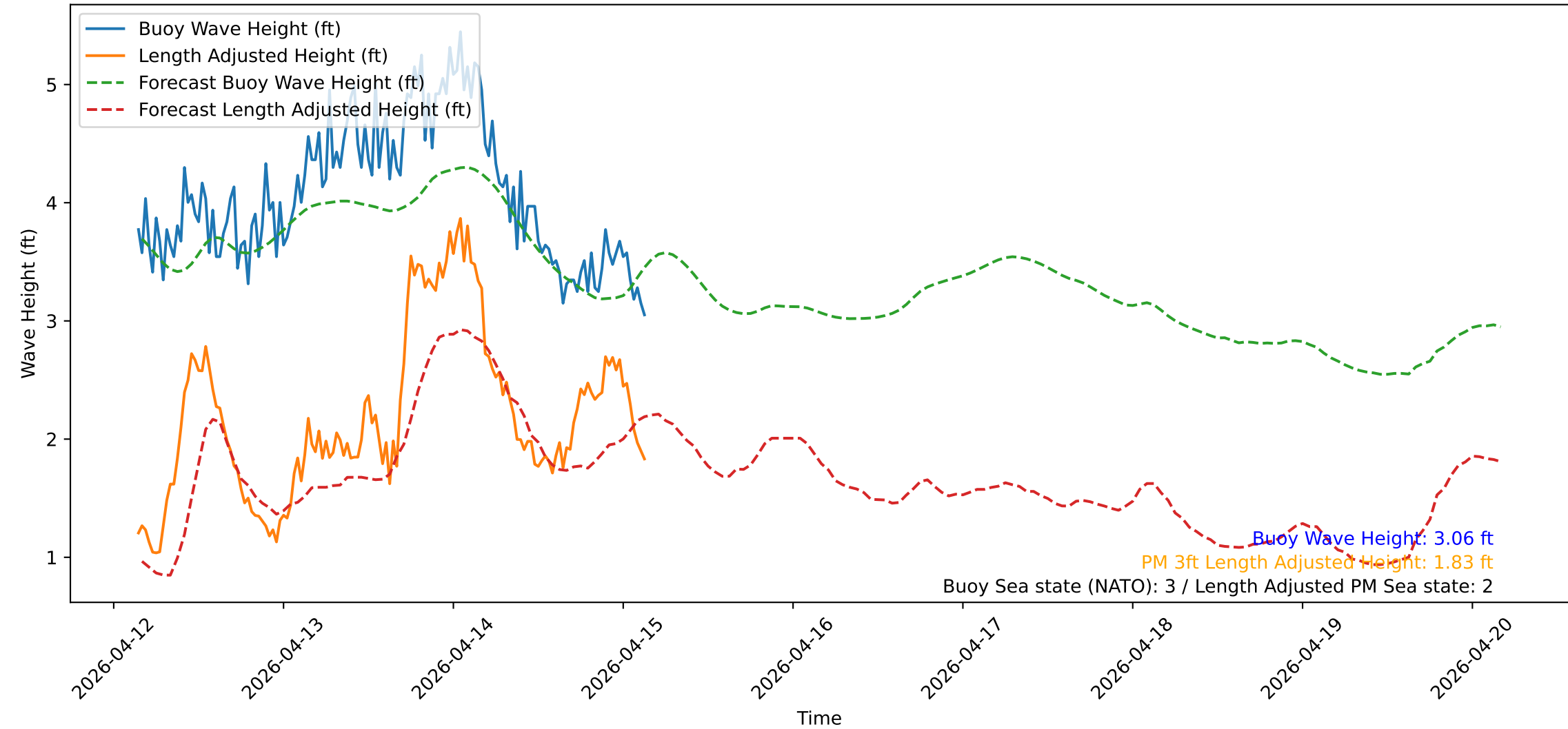
Wave Heights over Time for Oceanside Harbor at 2026-04-15 03:40:31
