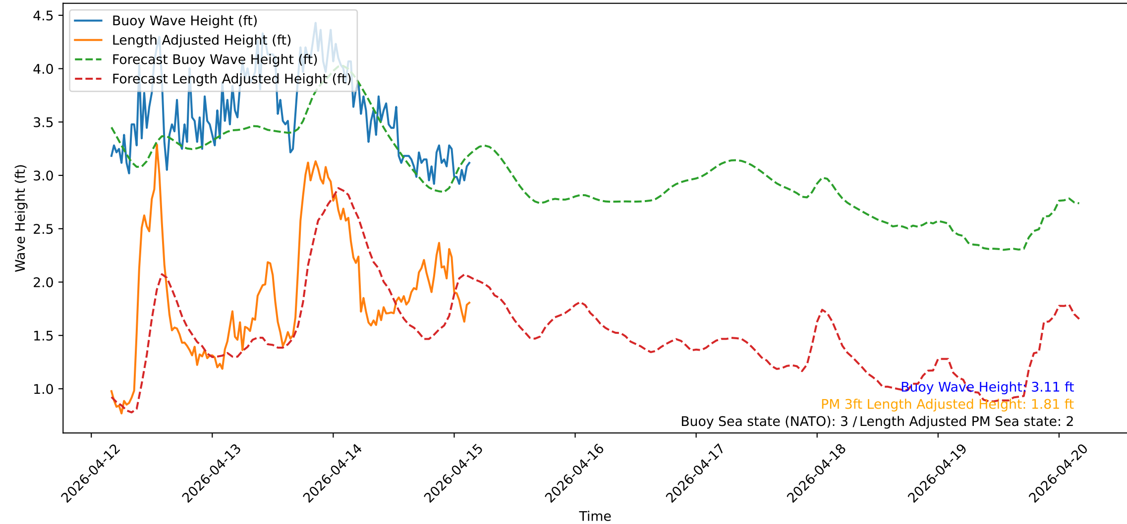
Wave Heights over Time for Red Beach at 2026-04-15 03:40:50
