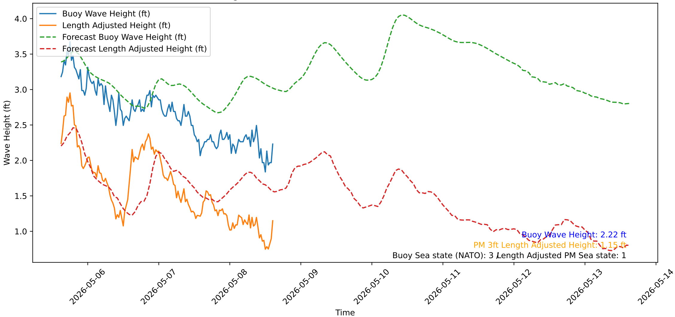
Wave Heights over Time for Green Beach at 2026-05-08 15:11:12
