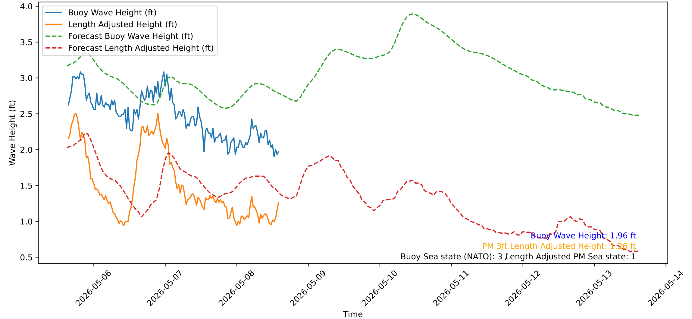
Wave Heights over Time for Red Beach at 2026-05-08 15:10:50
