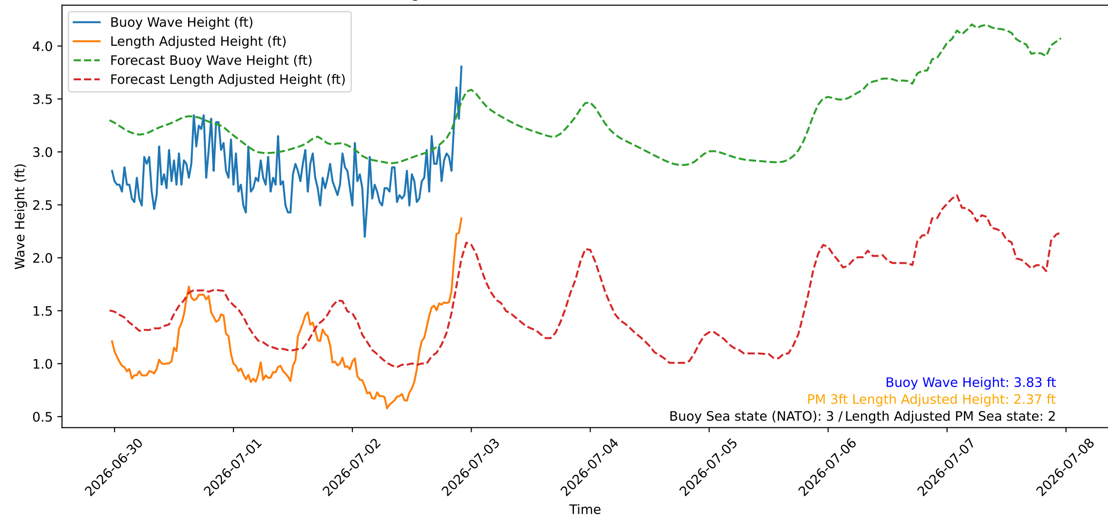
Wave Heights over Time for Red Beach at 2026-07-02 23:00:45
