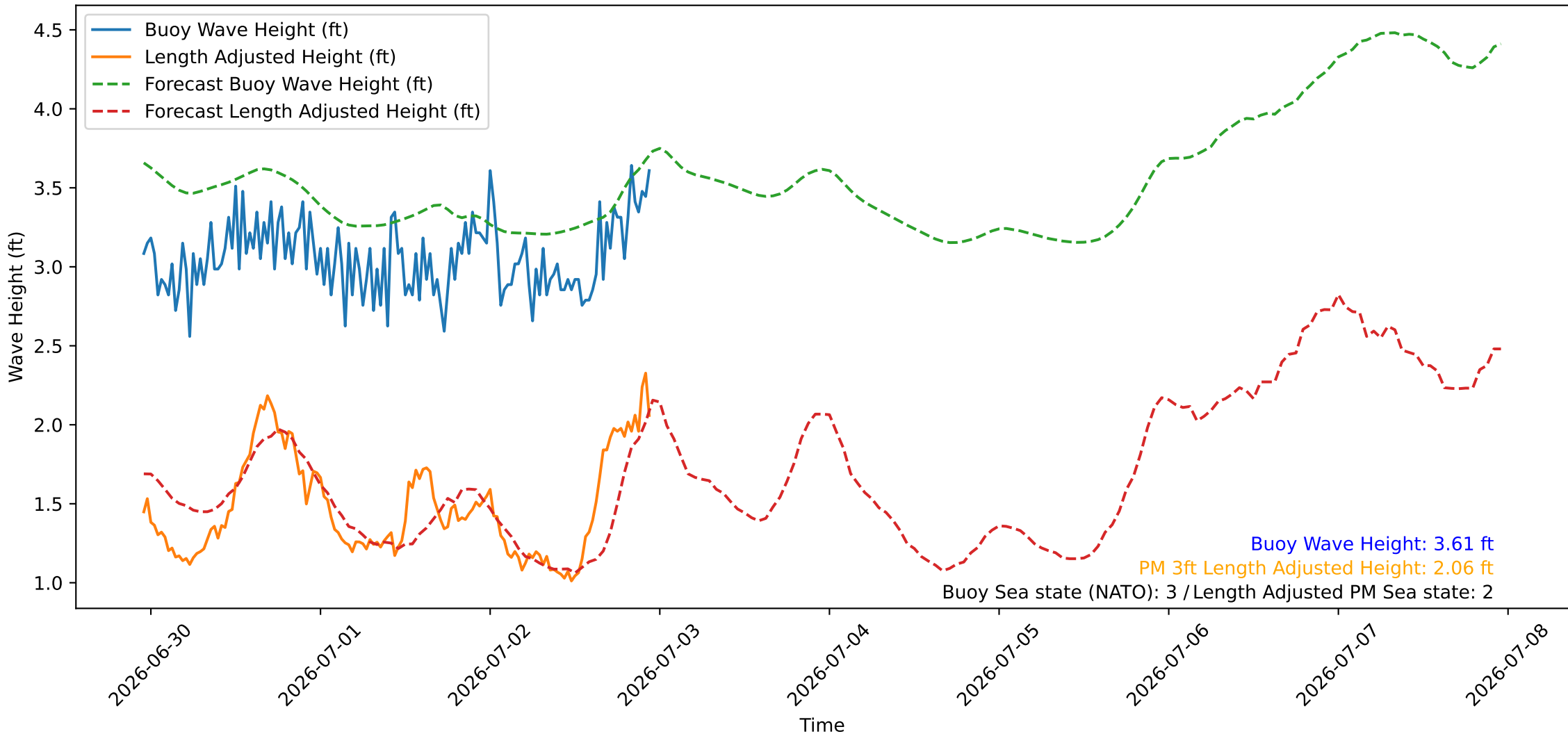
Wave Heights over Time for Oceanside Harbor at 2026-07-02 23:00:26
