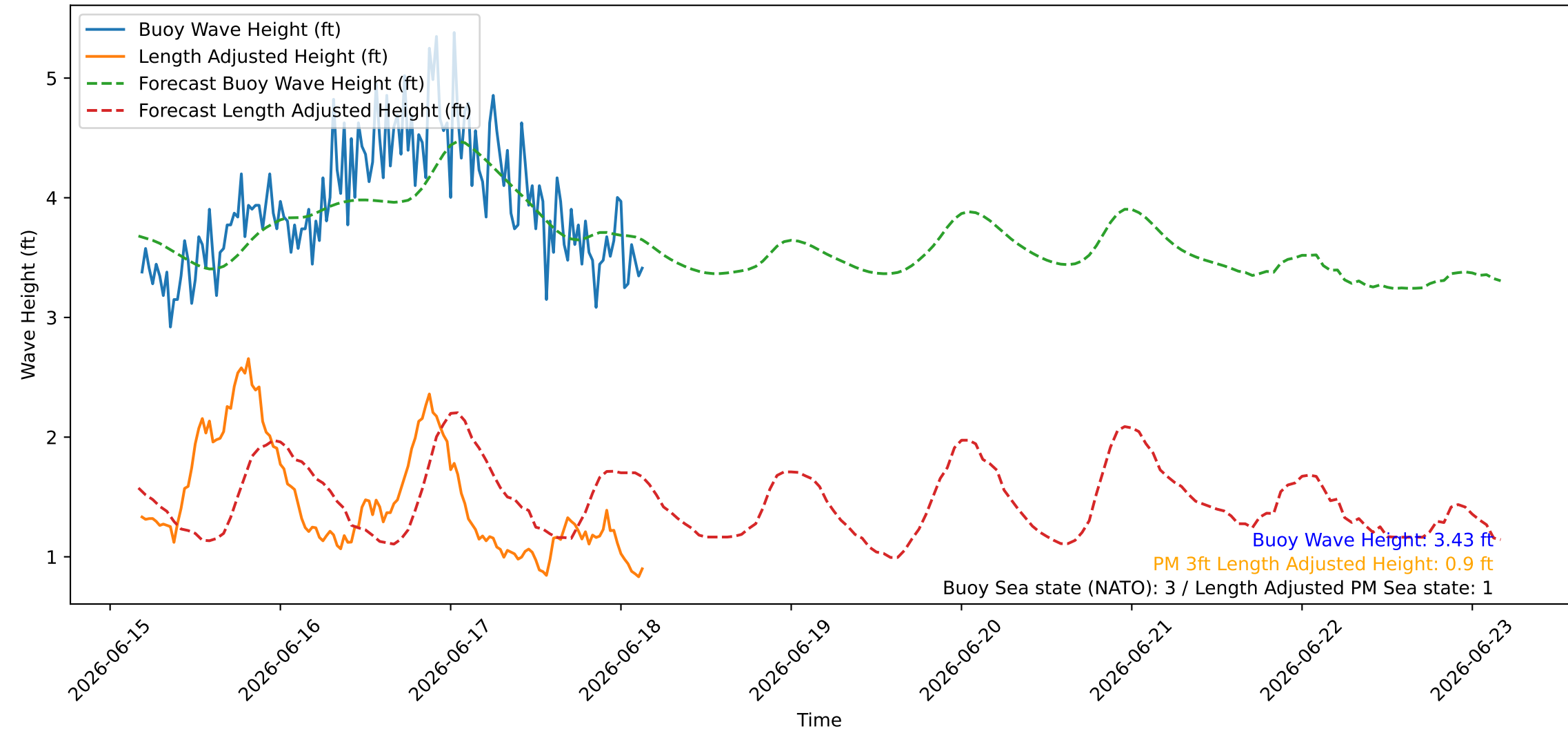
Wave Heights over Time for Red Beach at 2026-06-18 04:00:46
