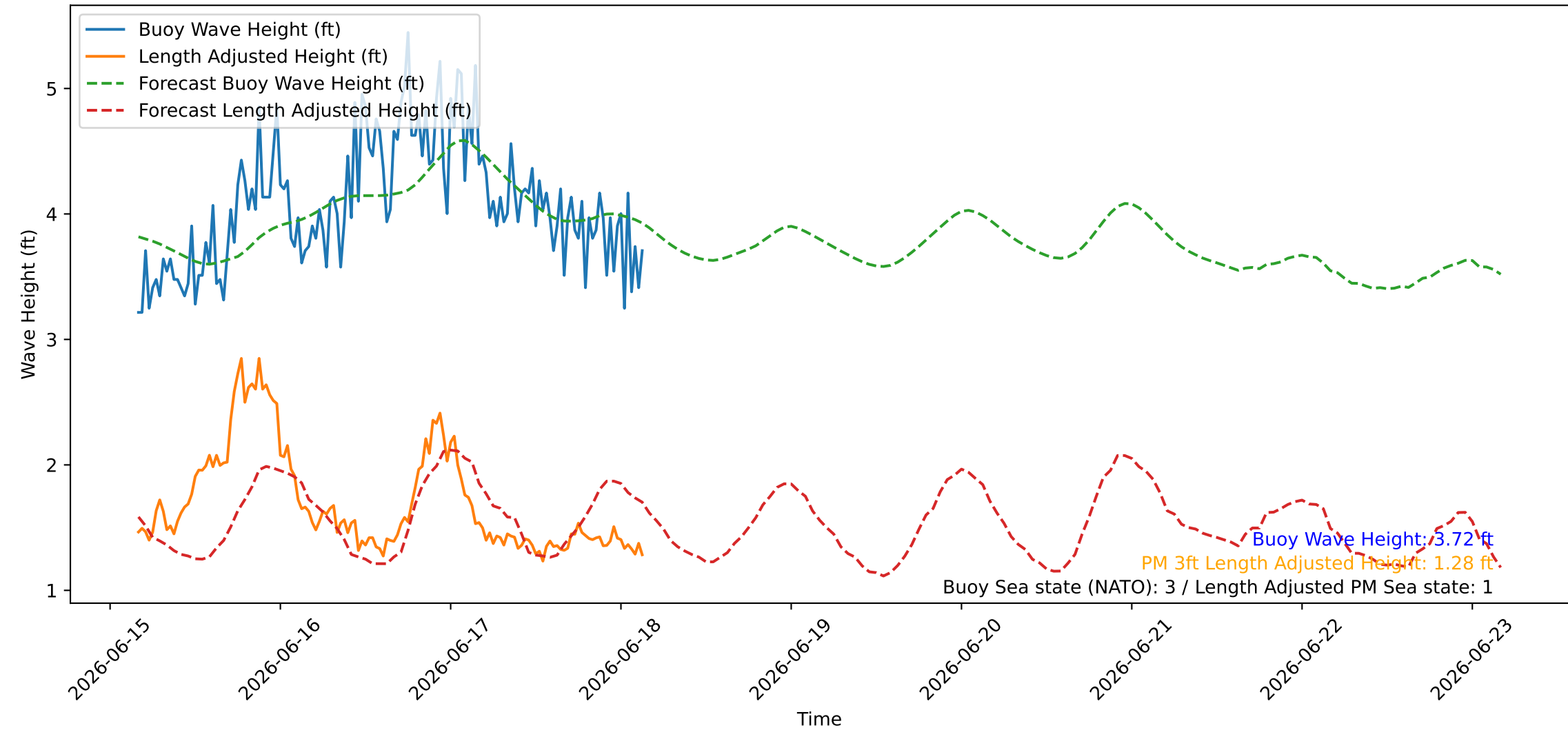
Wave Heights over Time for Oceanside Harbor at 2026-06-18 04:00:26
