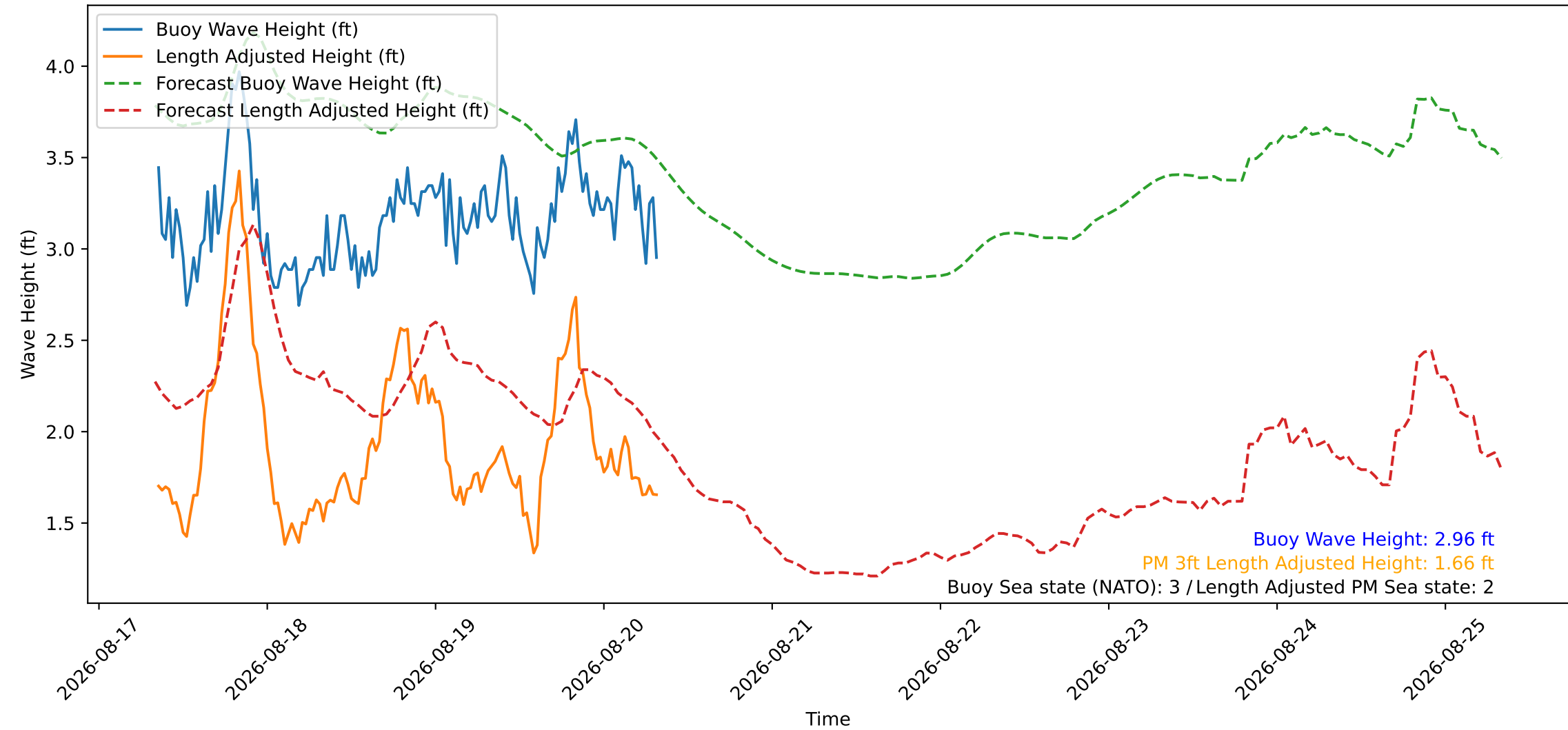
Wave Heights over Time for Green Beach at 2026-08-20 08:11:08
