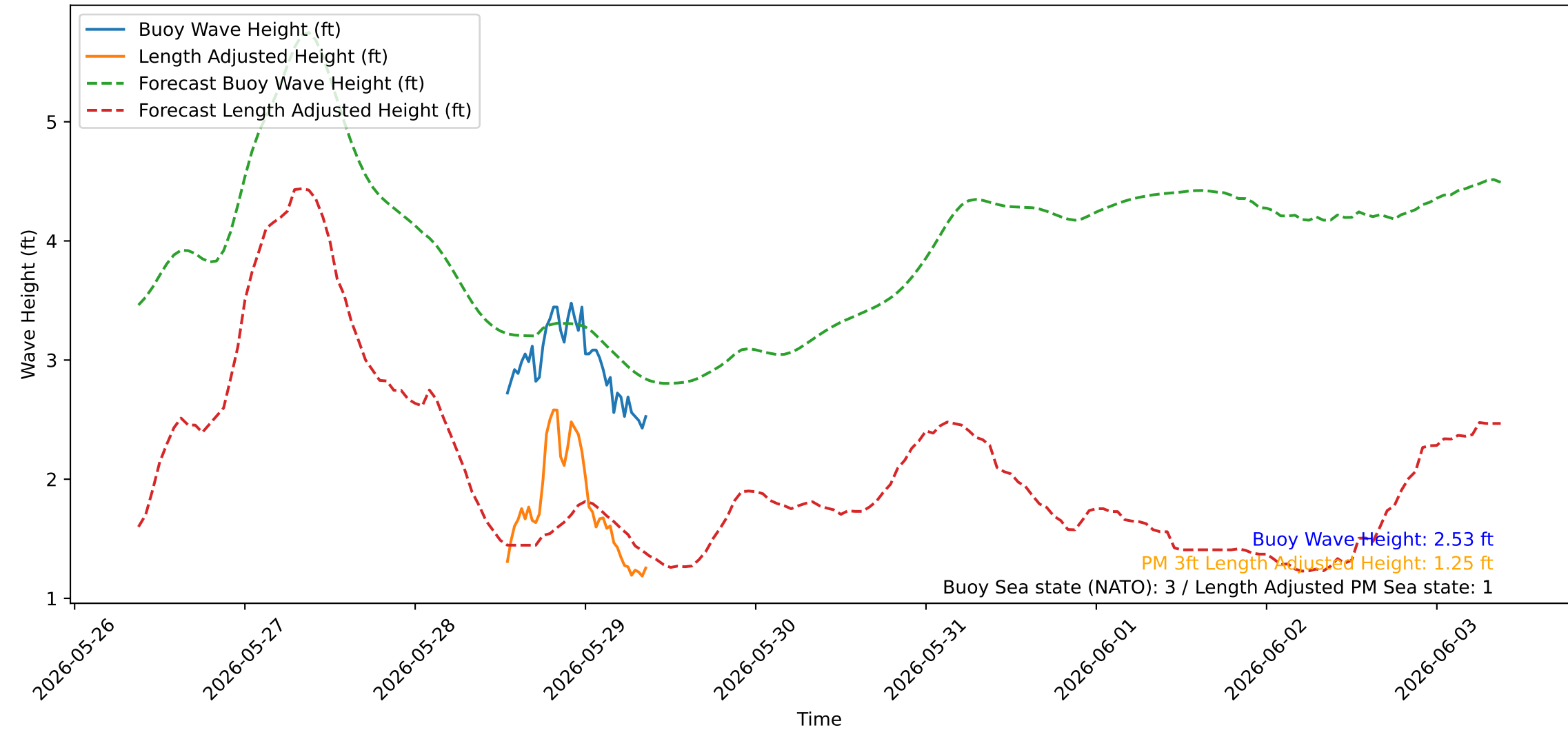
Wave Heights over Time for Oceanside Harbor at 2026-05-29 09:00:21
