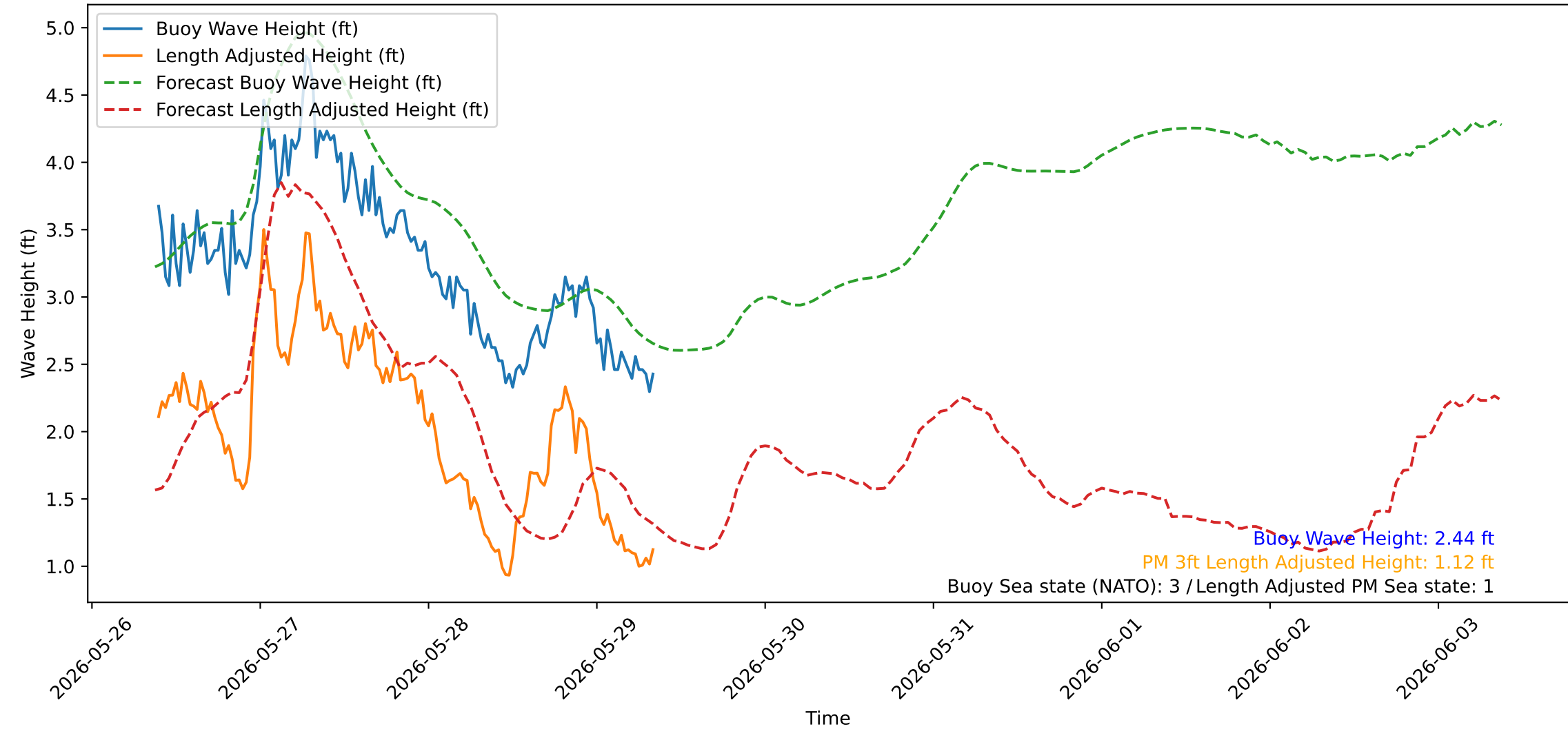
Wave Heights over Time for Red Beach at 2026-05-29 09:00:40
