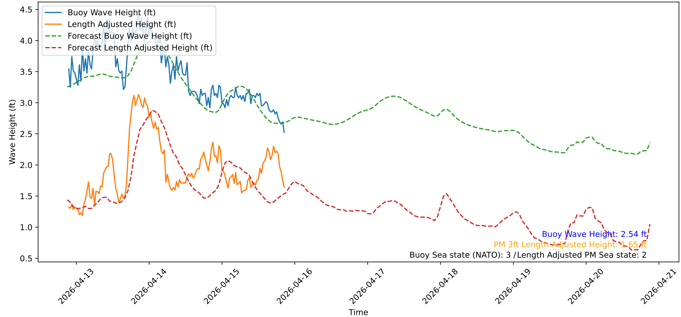
Wave Heights over Time for Red Beach at 2026-04-15 21:10:50
