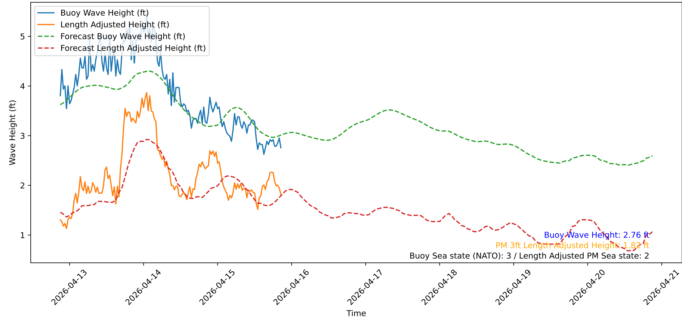
Wave Heights over Time for Oceanside Harbor at 2026-04-15 21:10:31
