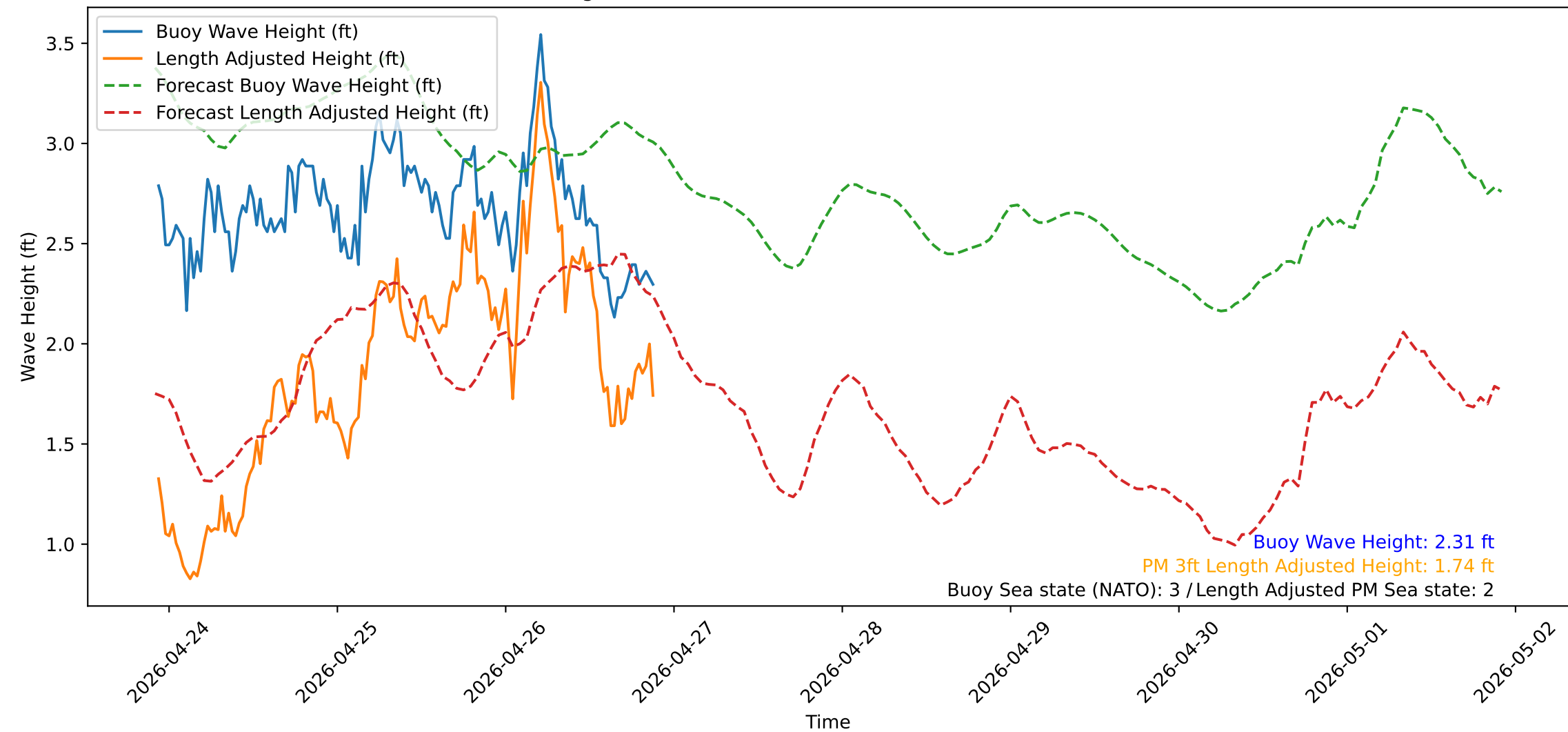
Wave Heights over Time for Red Beach at 2026-04-26 22:00:51
