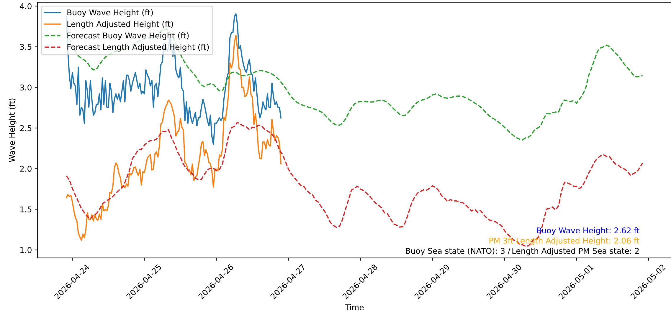
Wave Heights over Time for Oceanside Harbor at 2026-04-26 22:00:32
