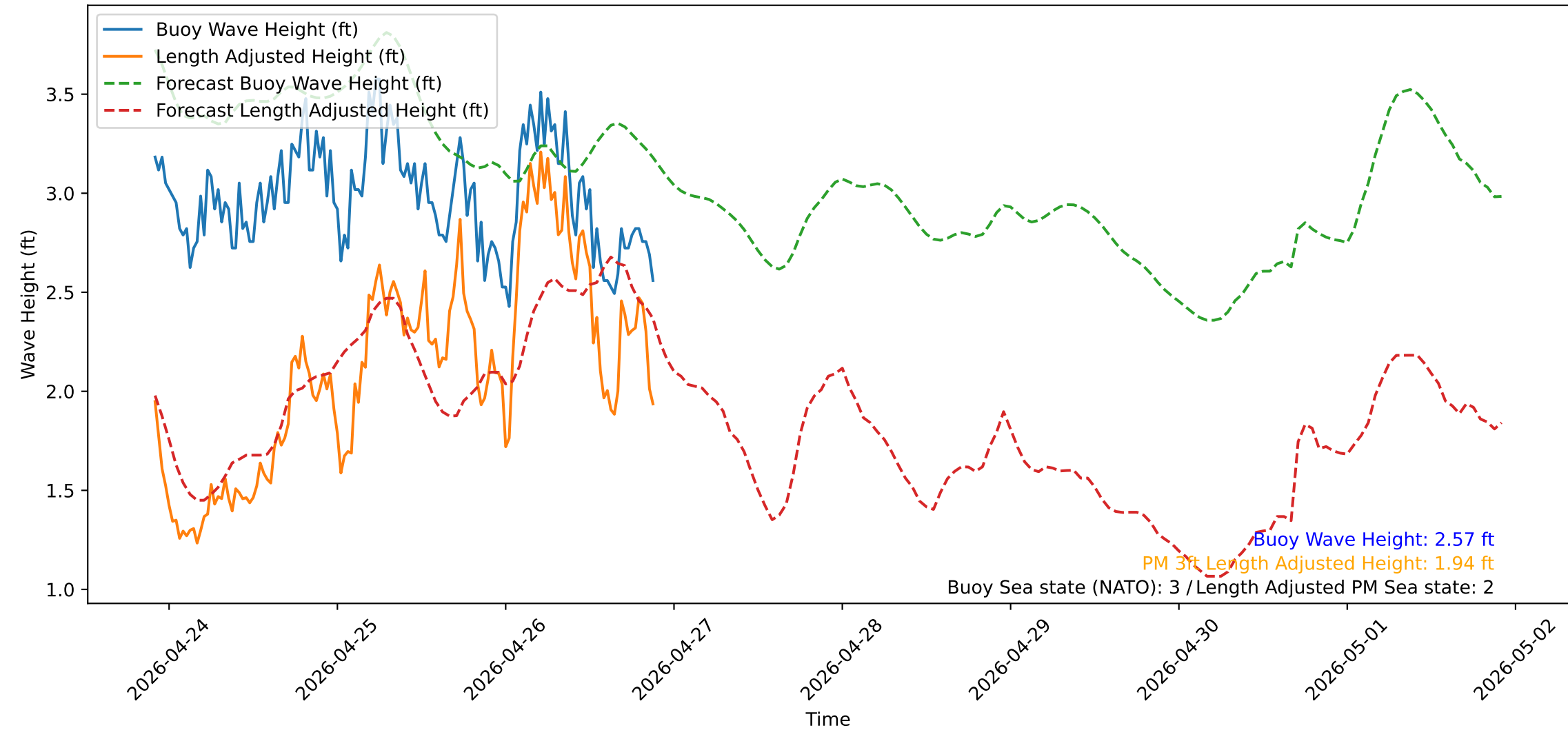
Wave Heights over Time for Green Beach at 2026-04-26 22:01:14
