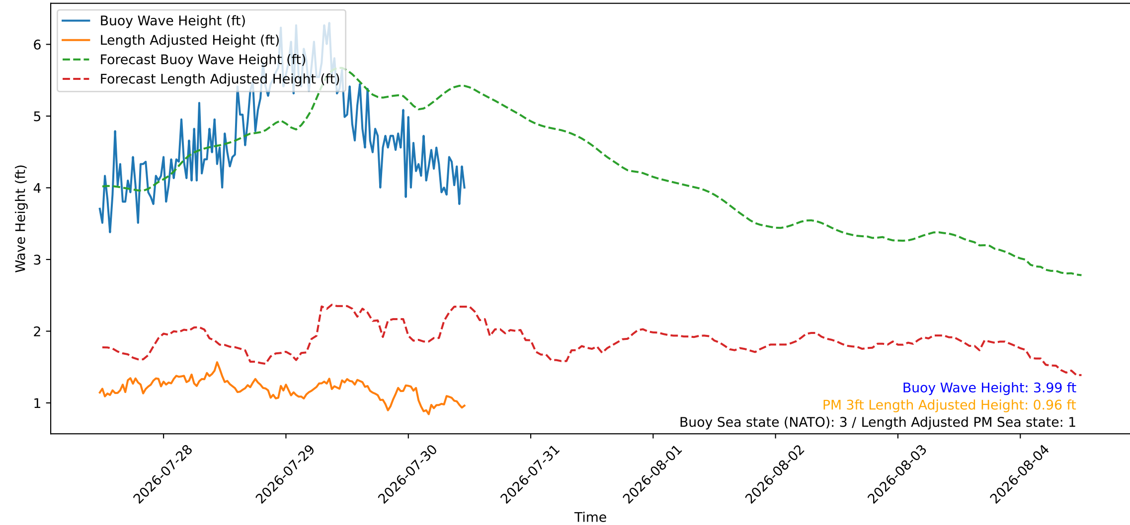
Wave Heights over Time for Green Beach at 2026-07-30 11:41:10
