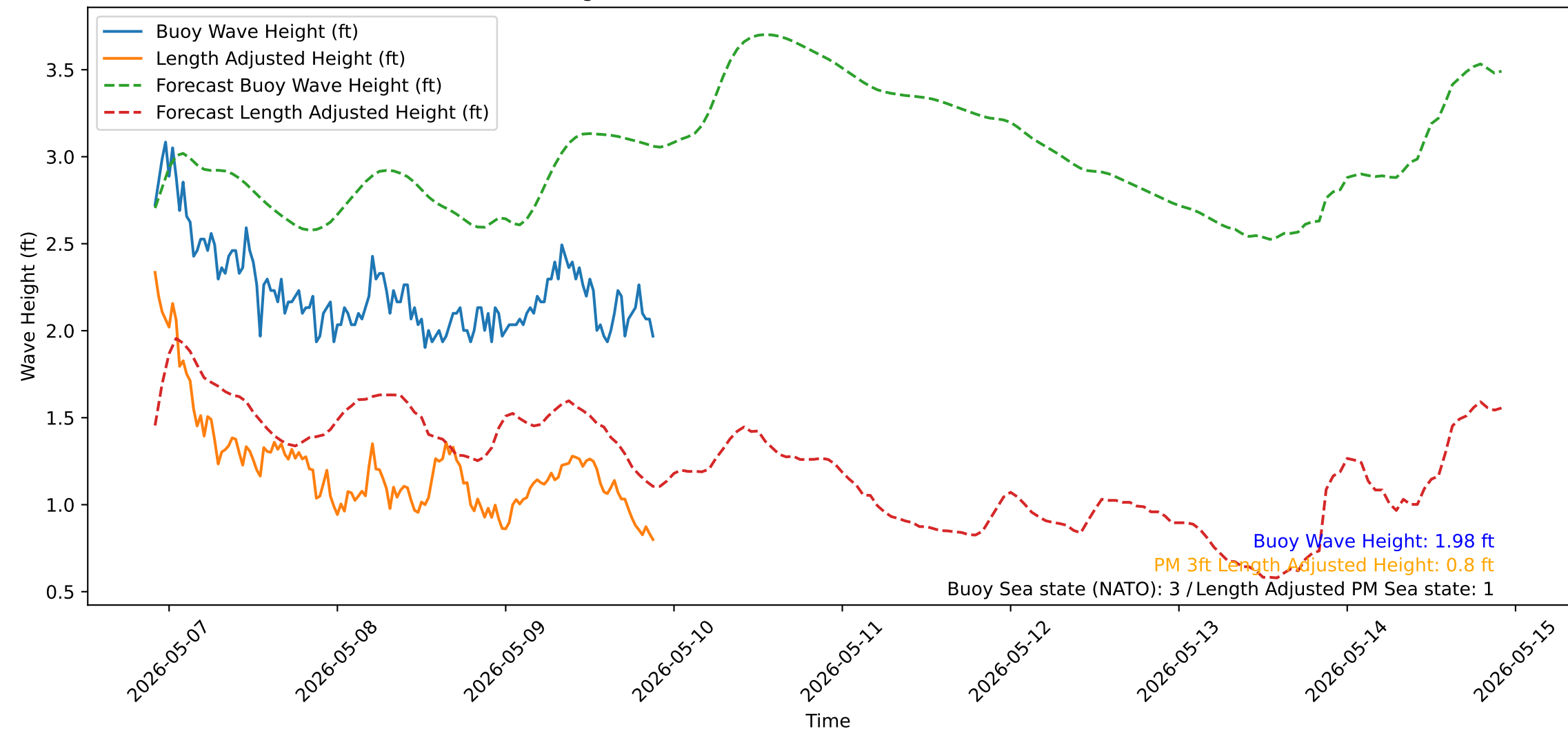
Wave Heights over Time for Red Beach at 2026-05-09 21:50:52
