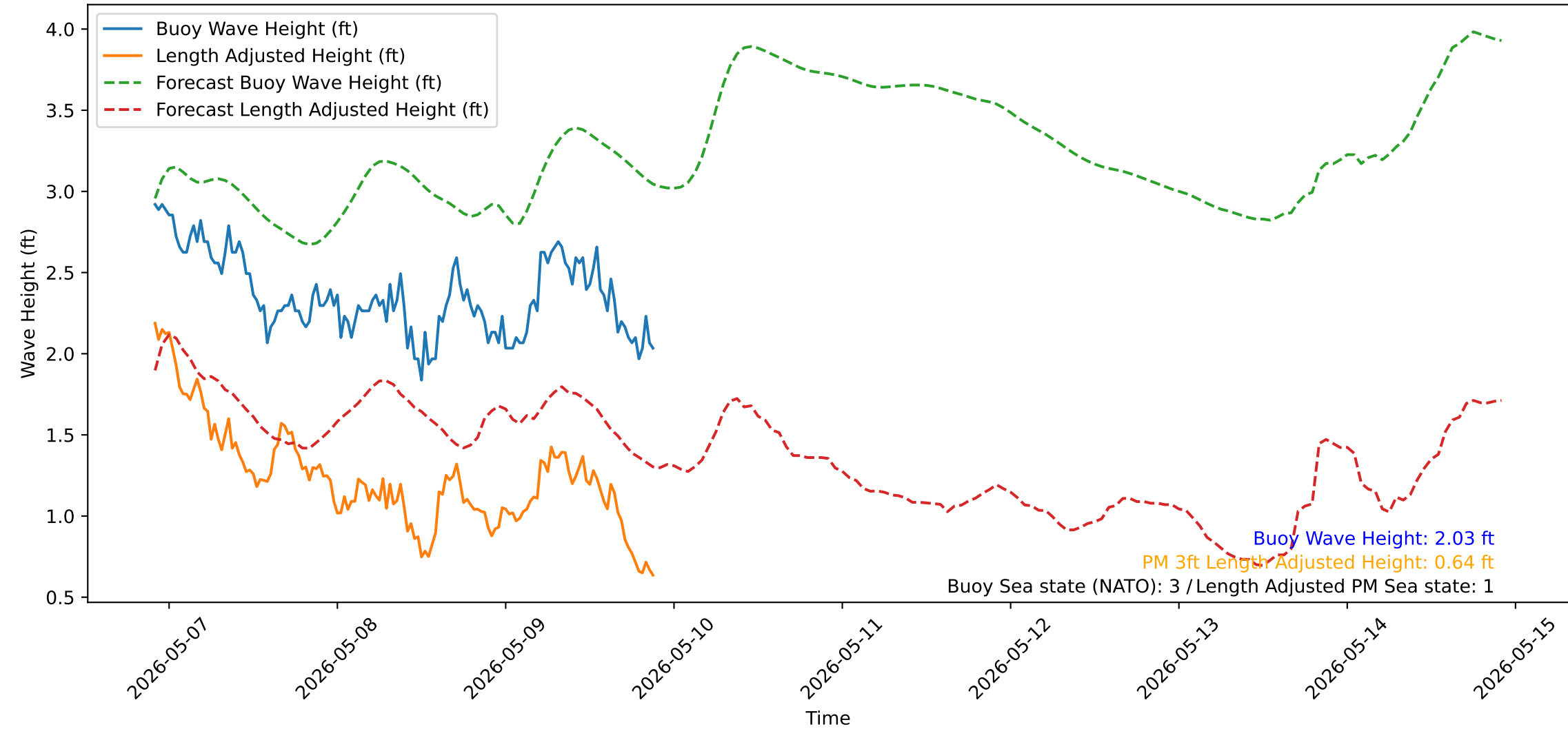
Wave Heights over Time for Green Beach at 2026-05-09 21:51:15
